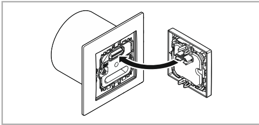
Abb. 10: Montage Sensor
