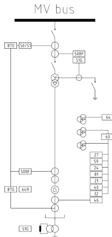
Fig. 4 Typical MV Generator Protection Single Line Diagram
