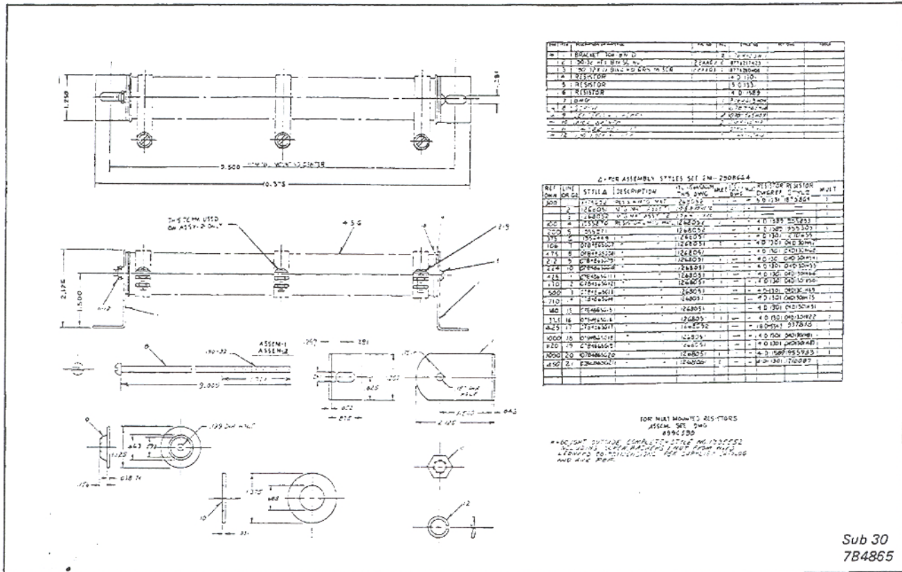
Fig. 11 Outline and Drilling Plan for External Resistor used with 250 V.D.C. Type DT-3 Temperature Relay.
