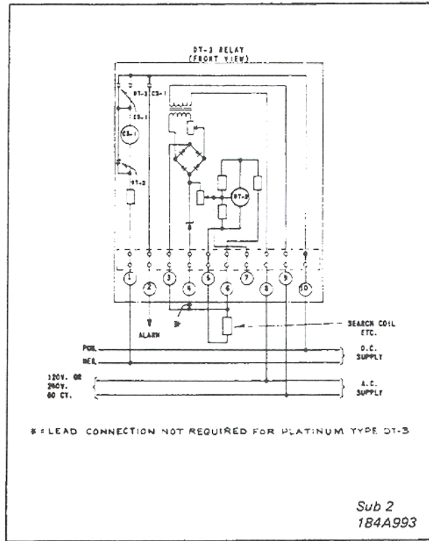
Fig. 10. Diagram of Test Connections for the AC Type DT-3 Temperature Relay in the Type FT21 Case.
