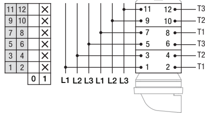
Switch-disconnector 6P
