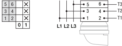
Switch-disconnector 4P
