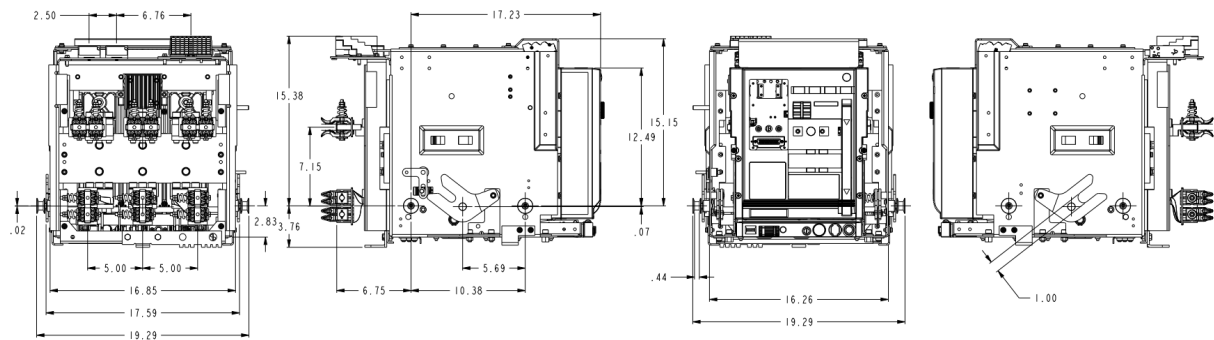
Figure 3. 800-2000A Retrofill Breaker (Entellisys Version) Dimensioning (REGX-08, REGS-16, REGH-16, REGS-20)
