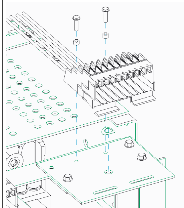
Figure 16. Entellisys— Secondary Disconnect Exploded View
