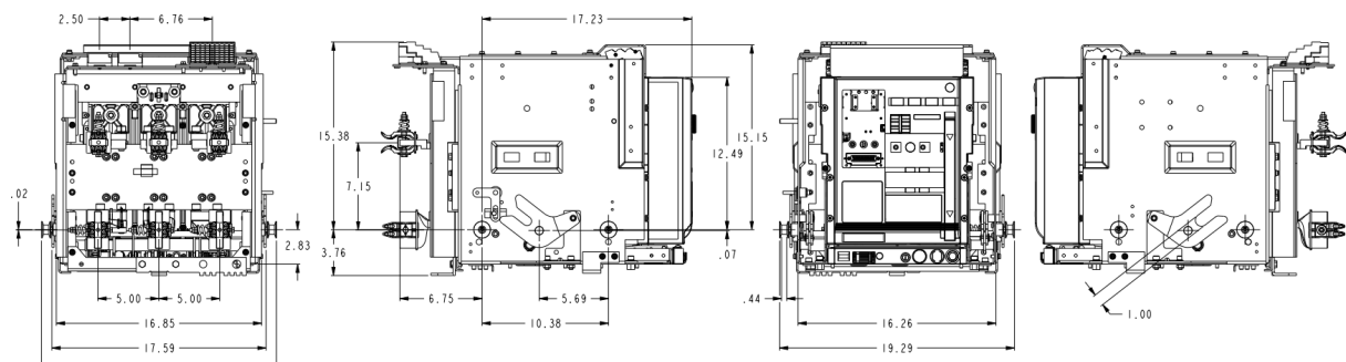
Figure 2. 800A Retrofill Breaker (Entellisys Version) Dimensioning (REGS-08, REGH-08)
