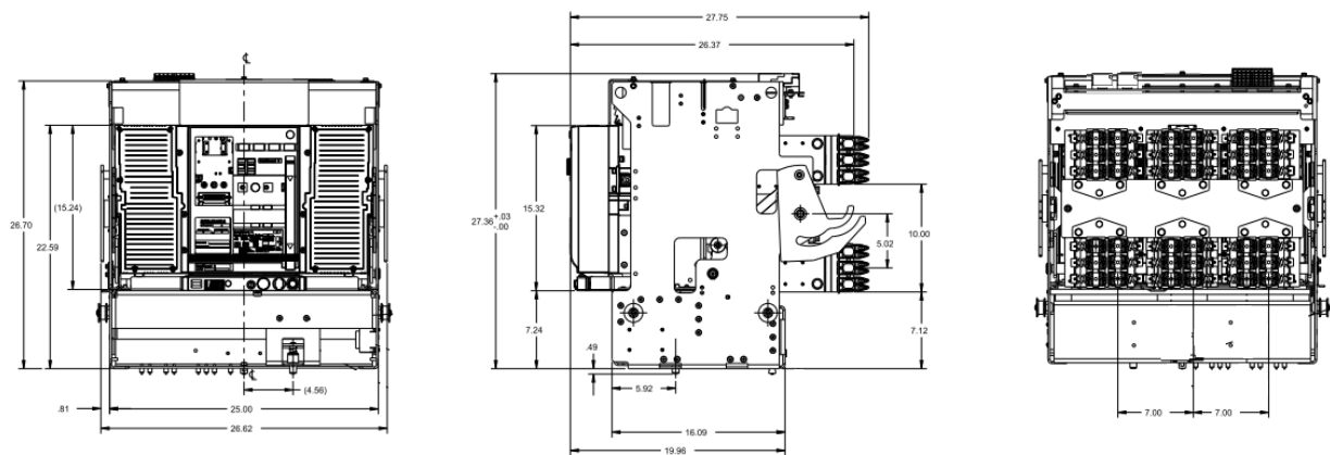
Figure 3B. 5000A Retrofill Breaker (Entellisys Version) Dimensioning (REGS-50,REGX-50)
