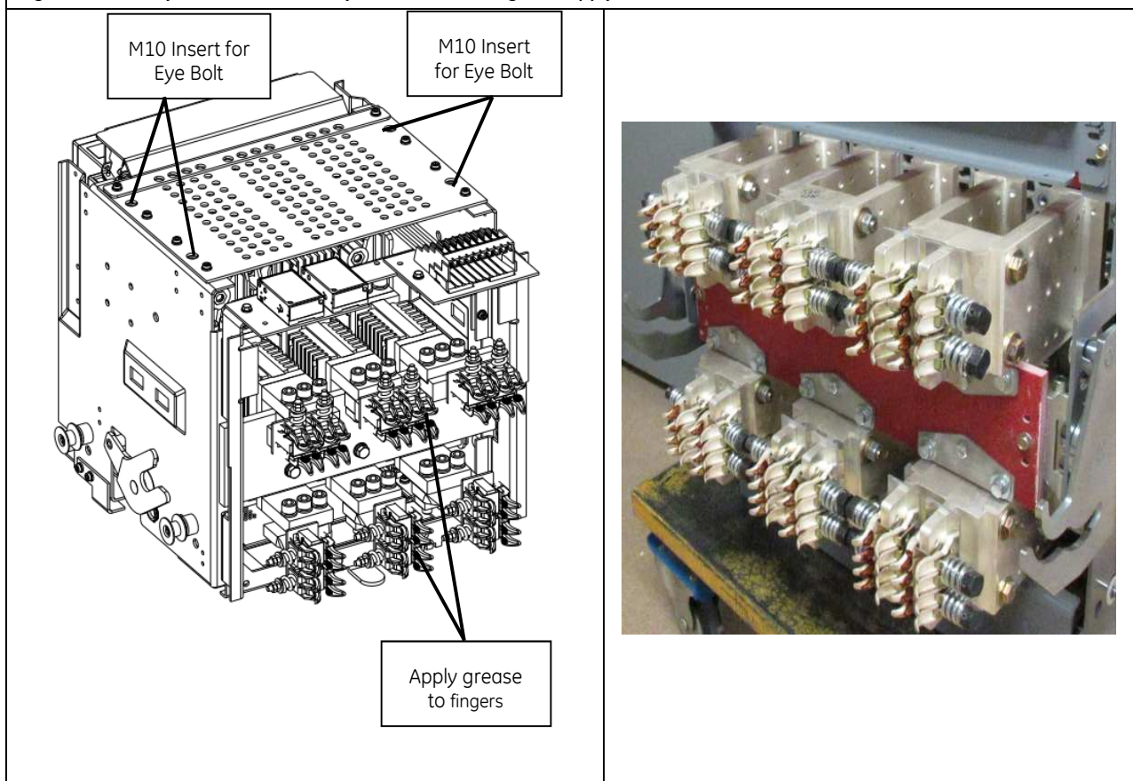
Figure 7. Entellisys Retrofill—Primary Contacts or “Fingers” (Apply Grease)
