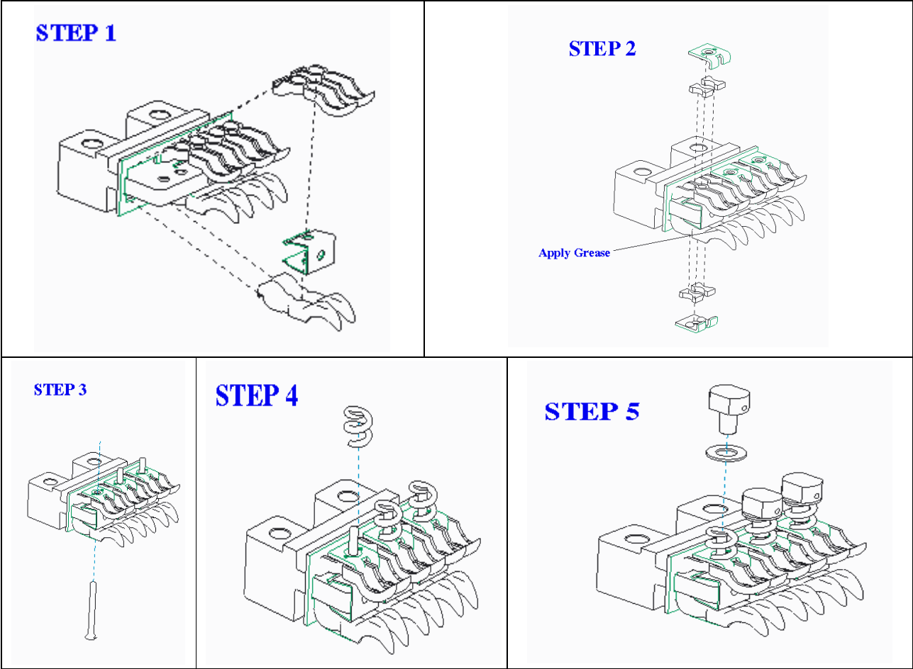
Figure 26. Steps in Exploded Views ( REGS-40/ REGX-40/REGS-50/REGX-50 )
