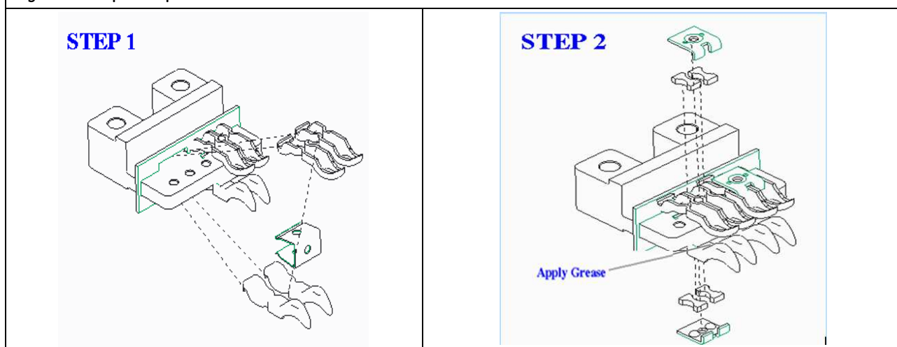
Figure 25. Steps in Exploded Views (REGS-32/REGH-32/REGX-32)
