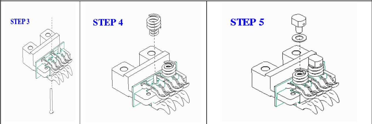
Figure 25. Steps in Exploded Views (REGS-32/REGH-32/REGX-32)
