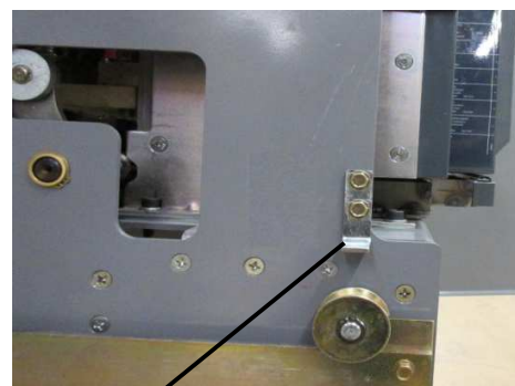
Door Interlock Bracket REGS-32, REGH-32, REGX-32, REGS-40, REGX-40, REGS-50, REGX-50
