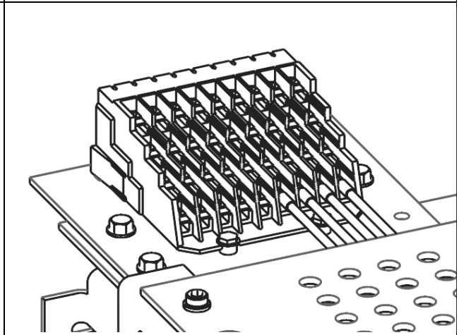
Figure 15. Entellisys Secondary Disconnect View 2
