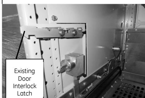
Figure 30. Entellisys—Door Interlocking Components
