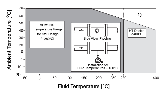
FIGURE 3-13 AMBIENT/FLUID TEMPERATURE RELATIONSHIP
