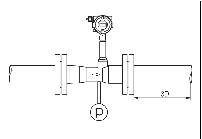
FIGURE 2-9 MEASURING PRESSURE
