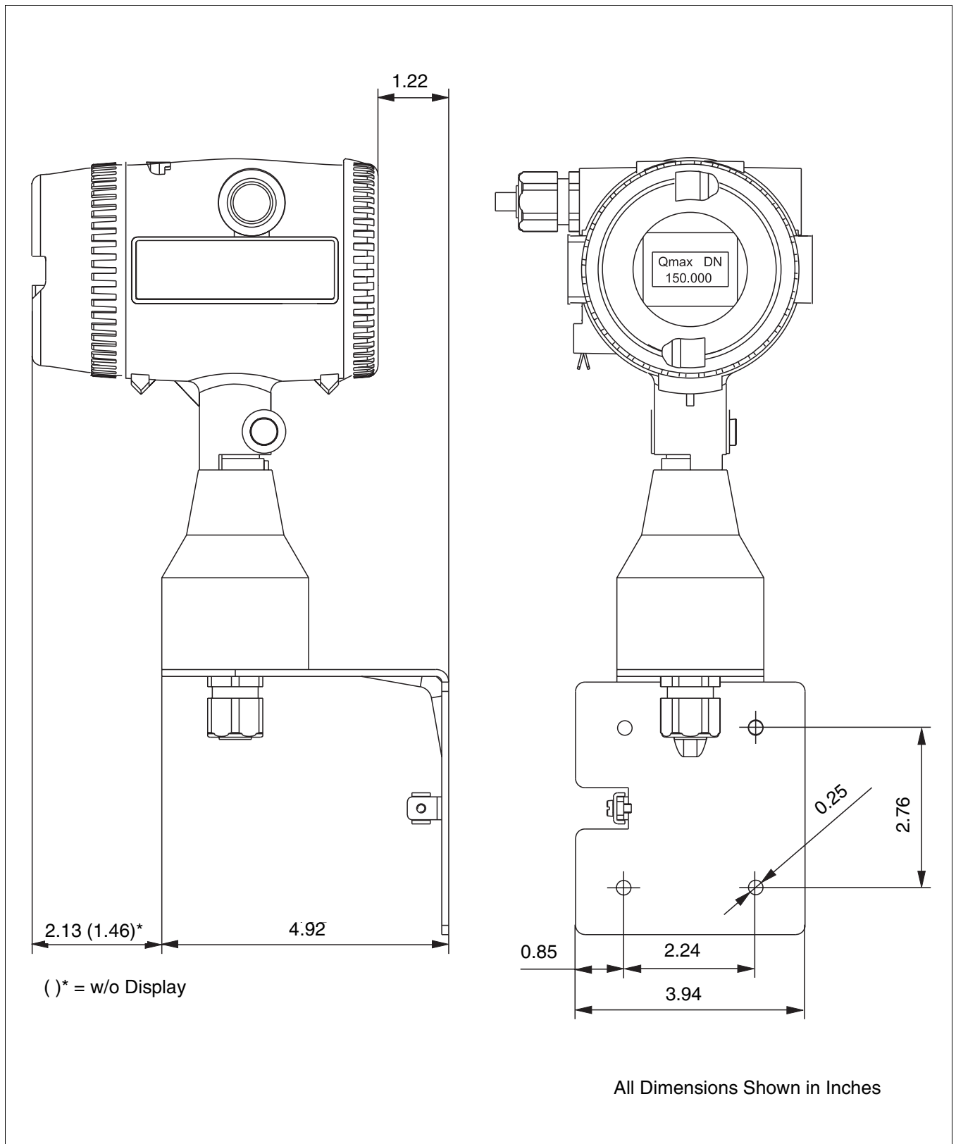
FIGURE 4-8 OUTLINE DIMENSIONS, VR/SR IN WALL-MOUNT HOUSING
