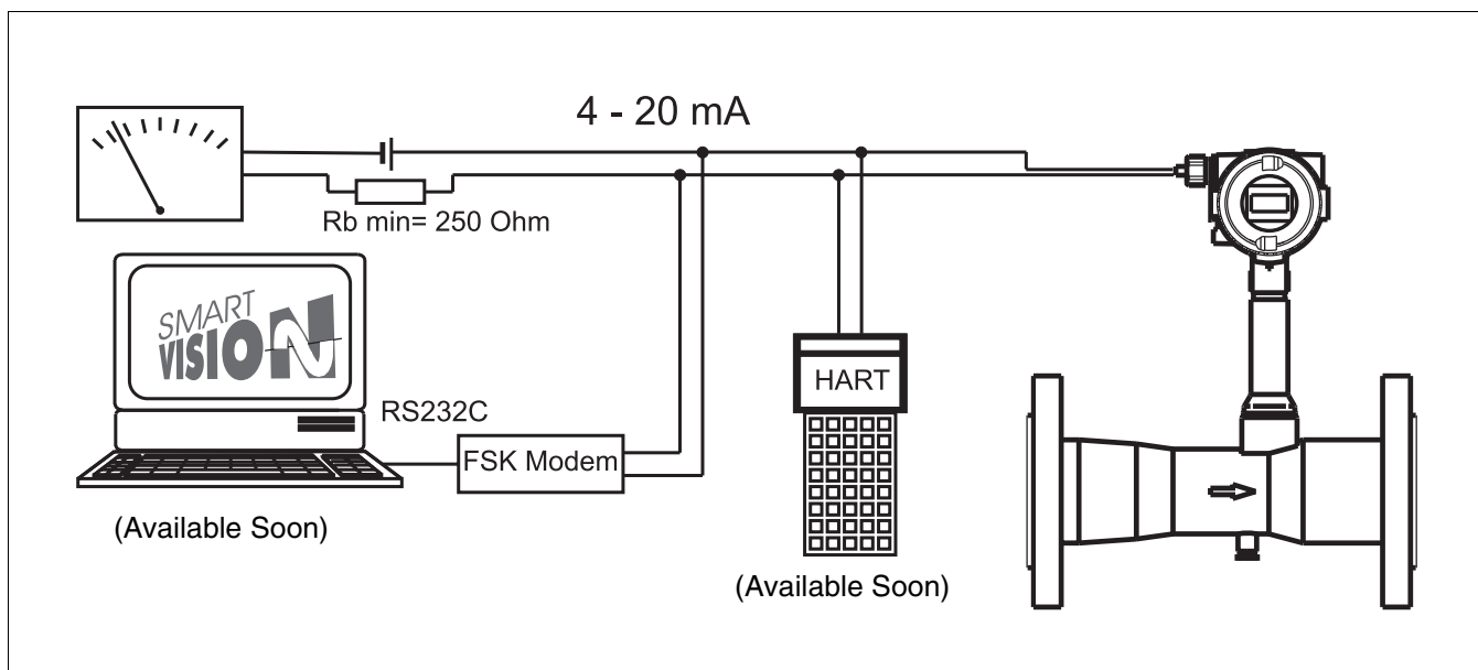
FIGURE 4-6 HART-Communication
