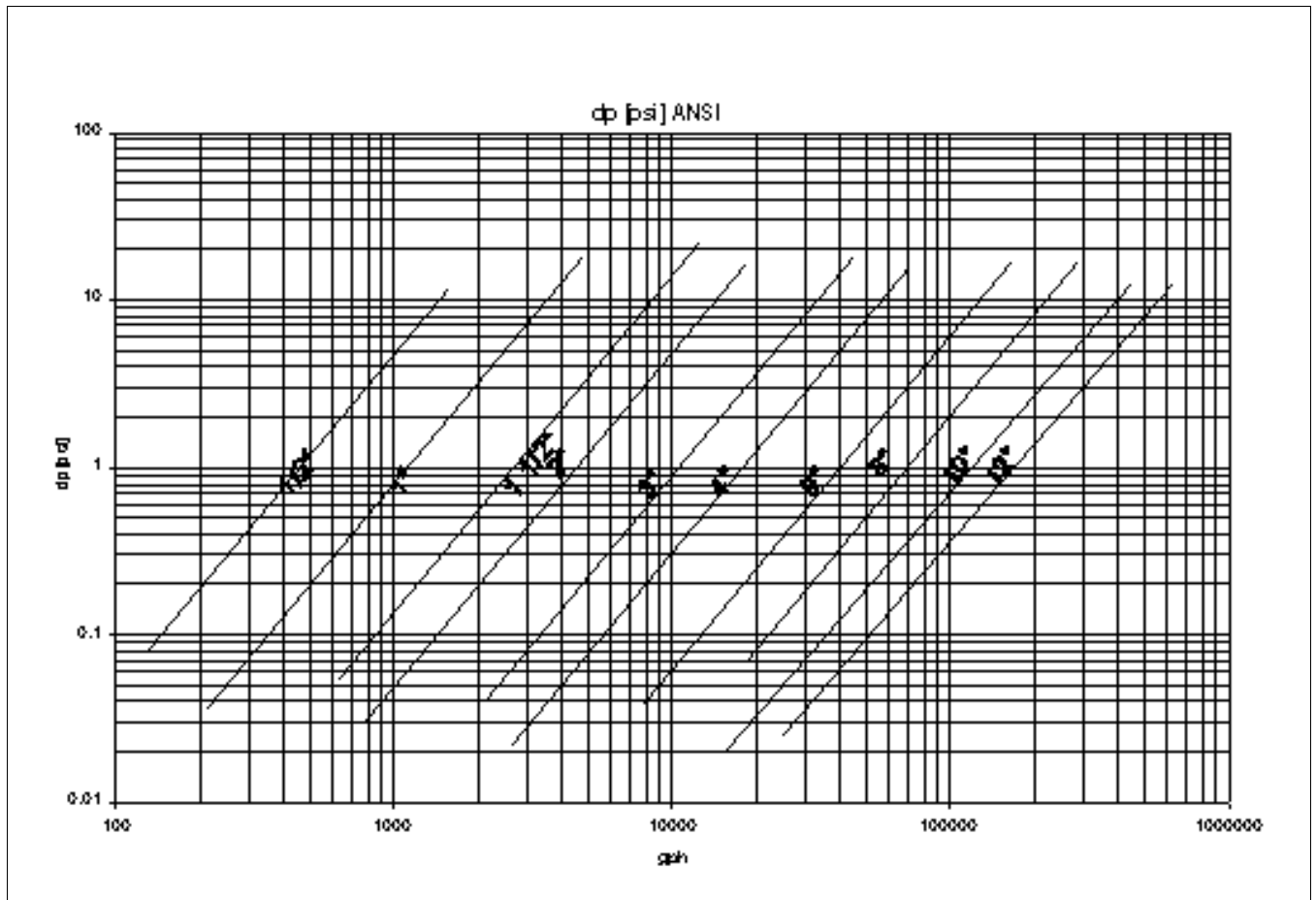
FIGURE 3-15 PRESSURE DROP, WATER (70° F, 14.67 psia, \rho=8.34 lb/gal)
