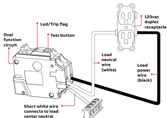
Wiring diagram
