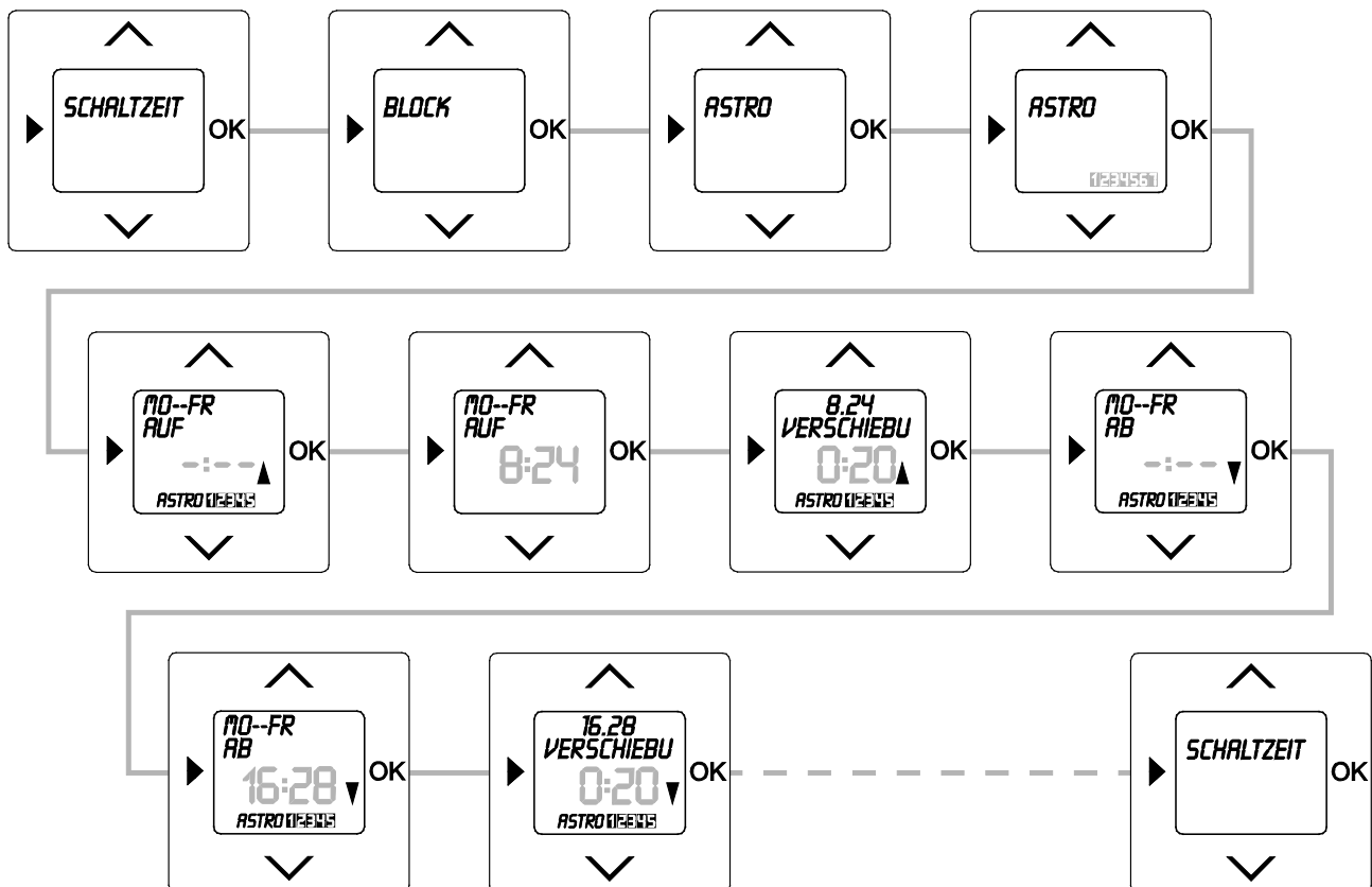
Fig. 11: Menu item – Astro
