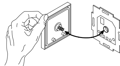
Fig. 16: Plug-on of attachment
