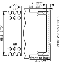
Capot scellable COV.01
