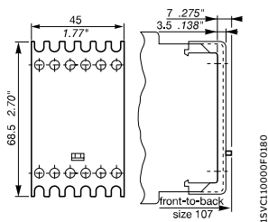
Capot scellable COV.02
