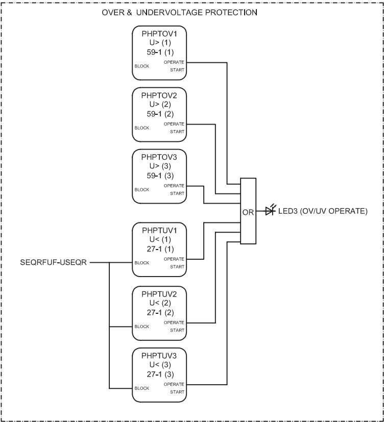
Figure 90: Overvoltage and undervoltage protection
