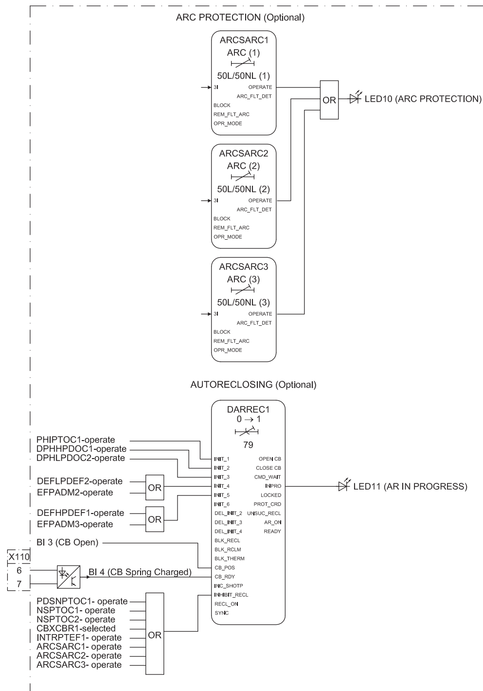
Figure 60: Arc protection
