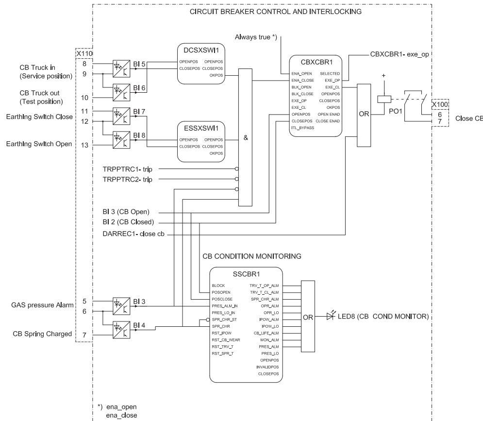
Figure 45: Circuit breaker control
