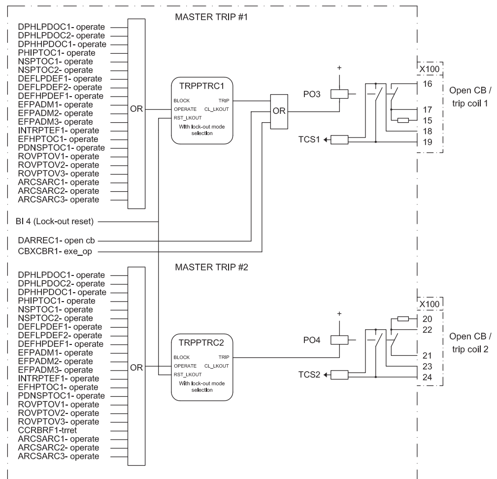
Figure 66: Master trip
