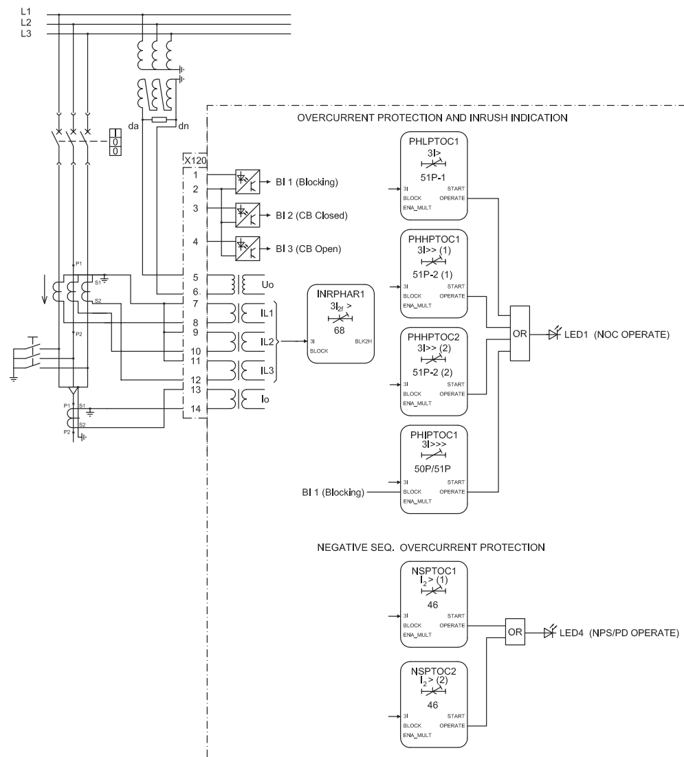
Figure 13: Overcurrent protection
