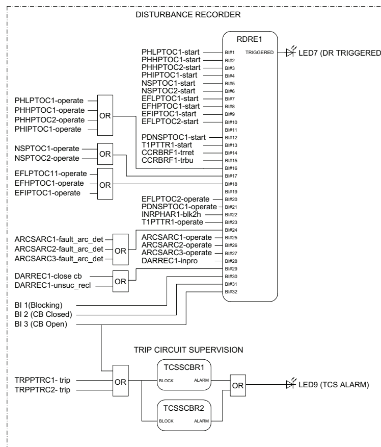
Figure 35: Disturbance recorder
