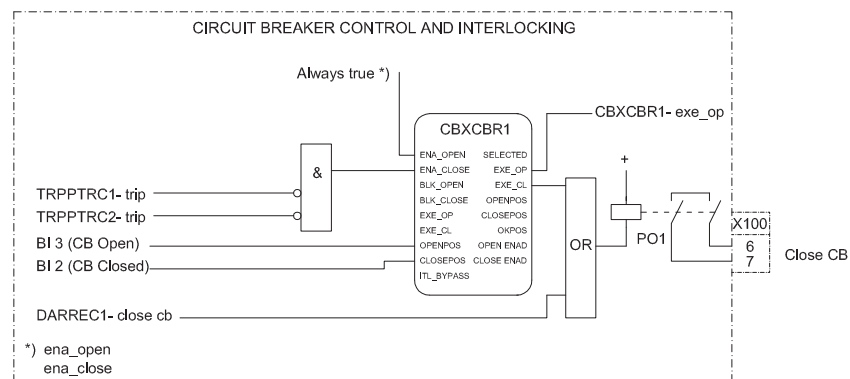
Figure 37: Circuit breaker control
