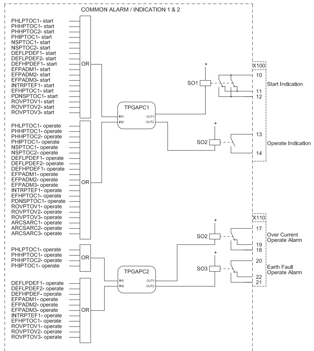
Figure 30: Alarm indication
