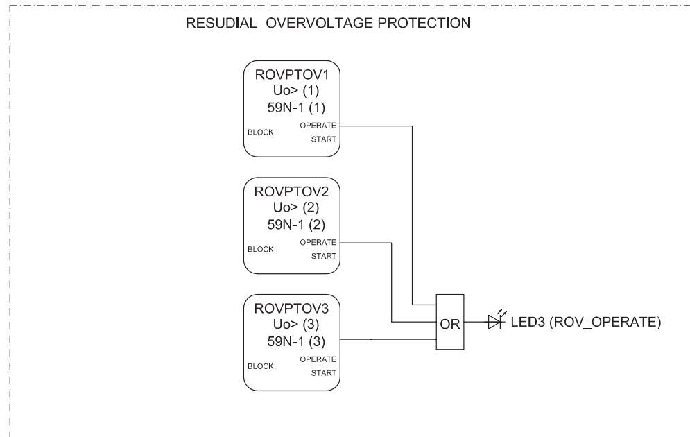
Figure 15: Residual overvoltage protection
