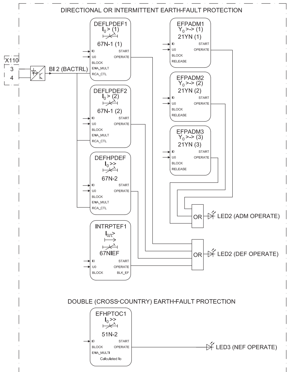
Figure 23: Directional earth-fault protection
