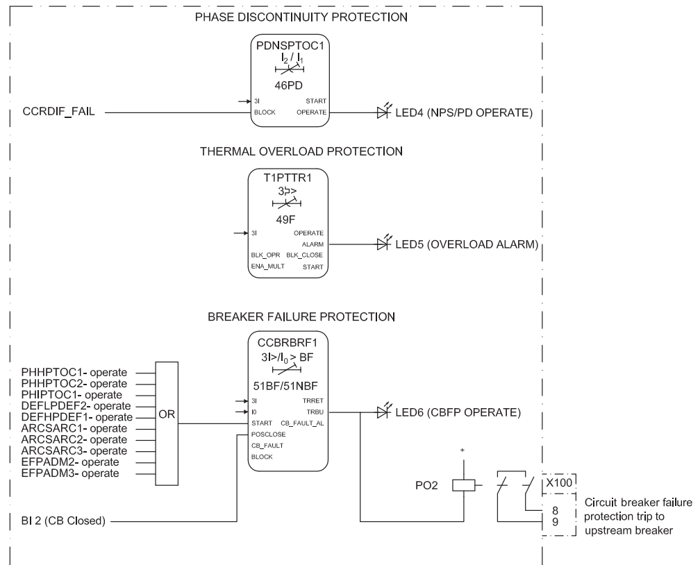
Figure 50: Phase discontinuity, thermal overload and circuit breaker failure protection
