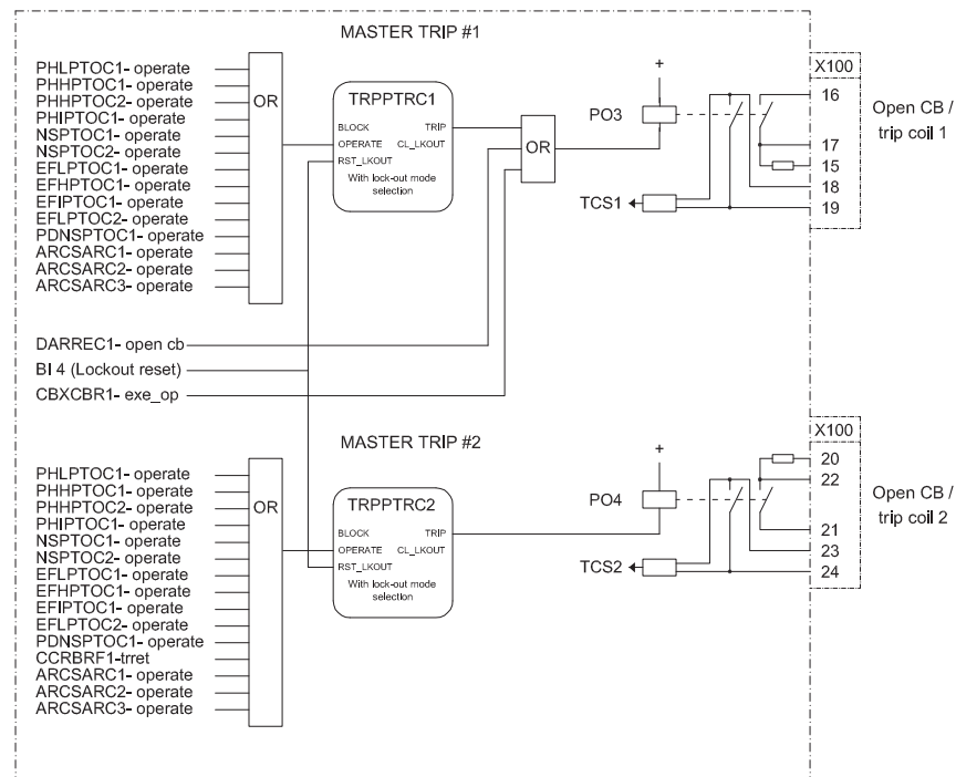
Figure 36: Master trip
