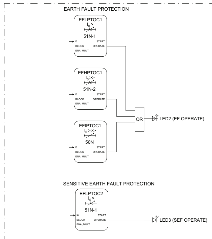
Figure 40: Non-directional earth-fault protection
