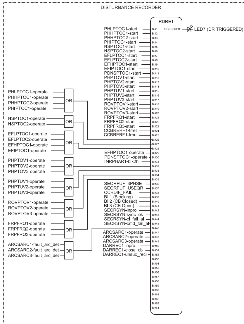
Figure 93: Disturbance recorder
