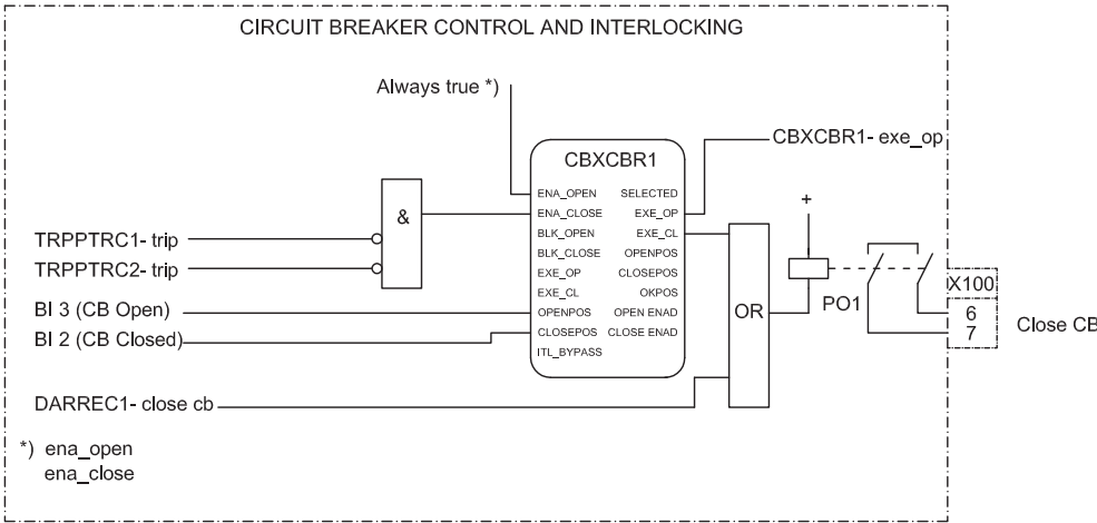
Figure 20: Circuit breaker control
