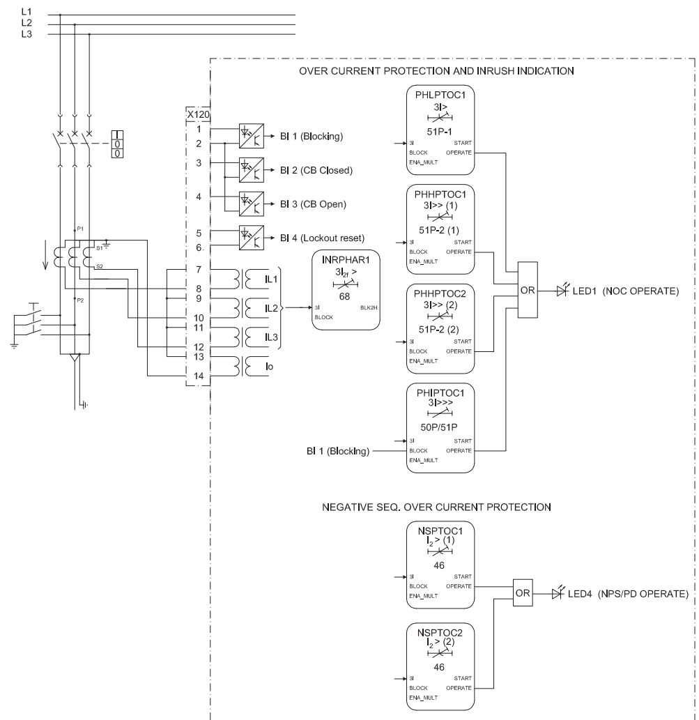
Figure 31: Overcurrent protection
