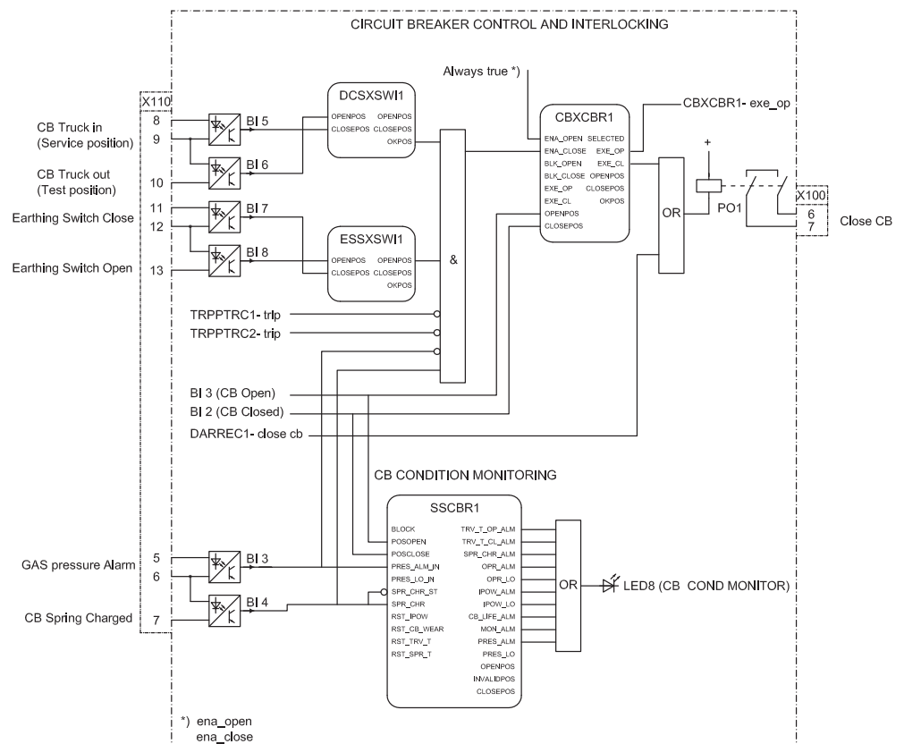
Figure 67: Circuit breaker control
