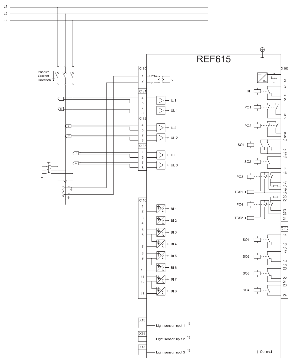
Figure 11: Connection diagram for the G configuration
