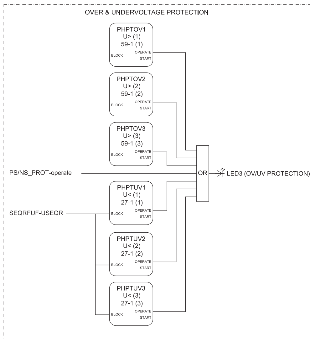
Figure 61: Overvoltage and undervoltage protection
