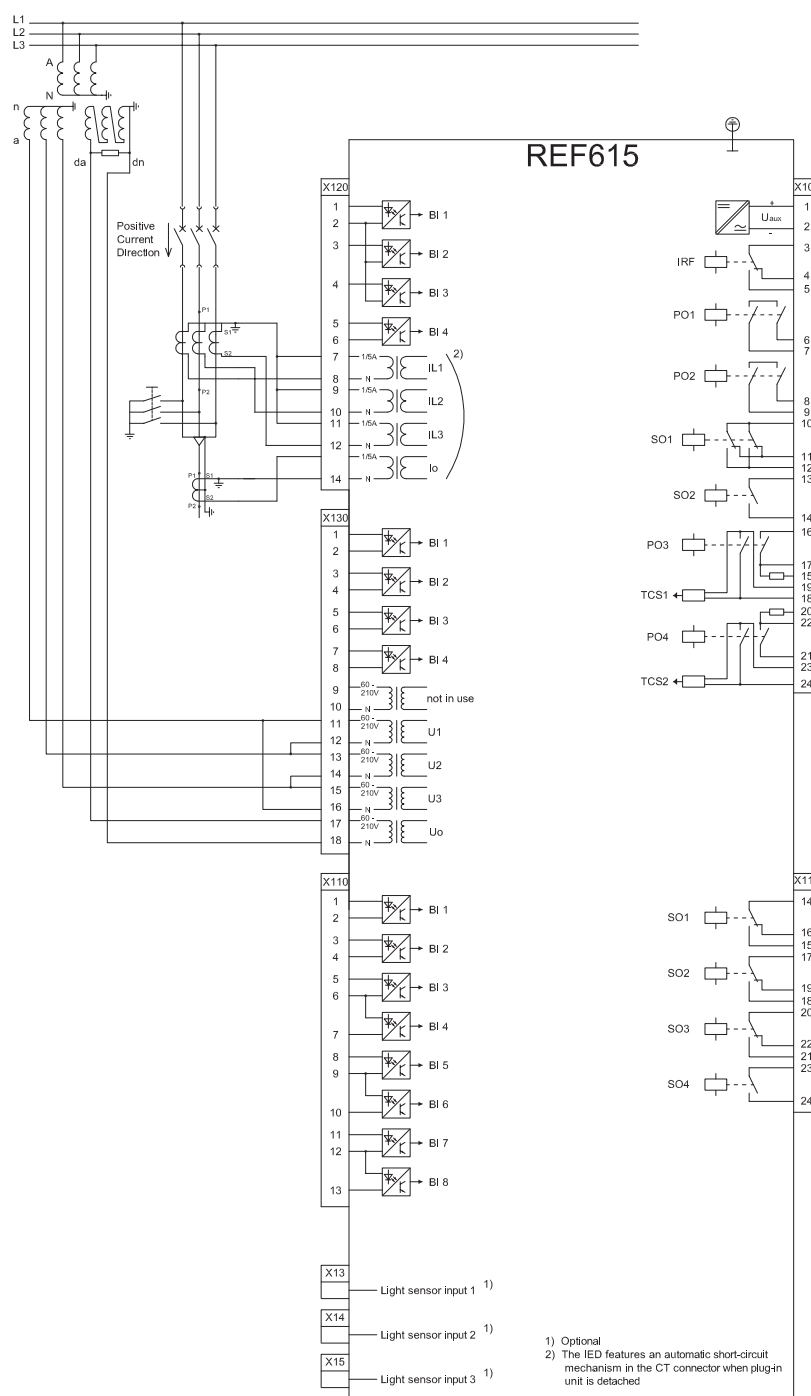
Figure 9: Connection diagram for the E and F configurations
