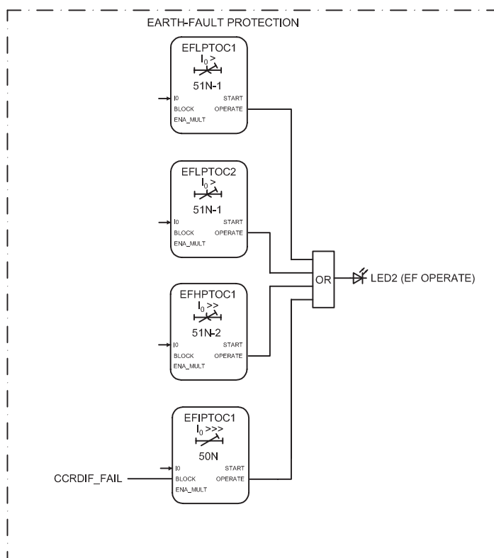
Figure 85: Non-directional earth-fault protection
