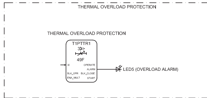
Figure 71: Thermal overload protection
