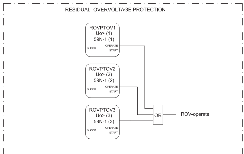
Figure 63: Residual overvoltage protection
