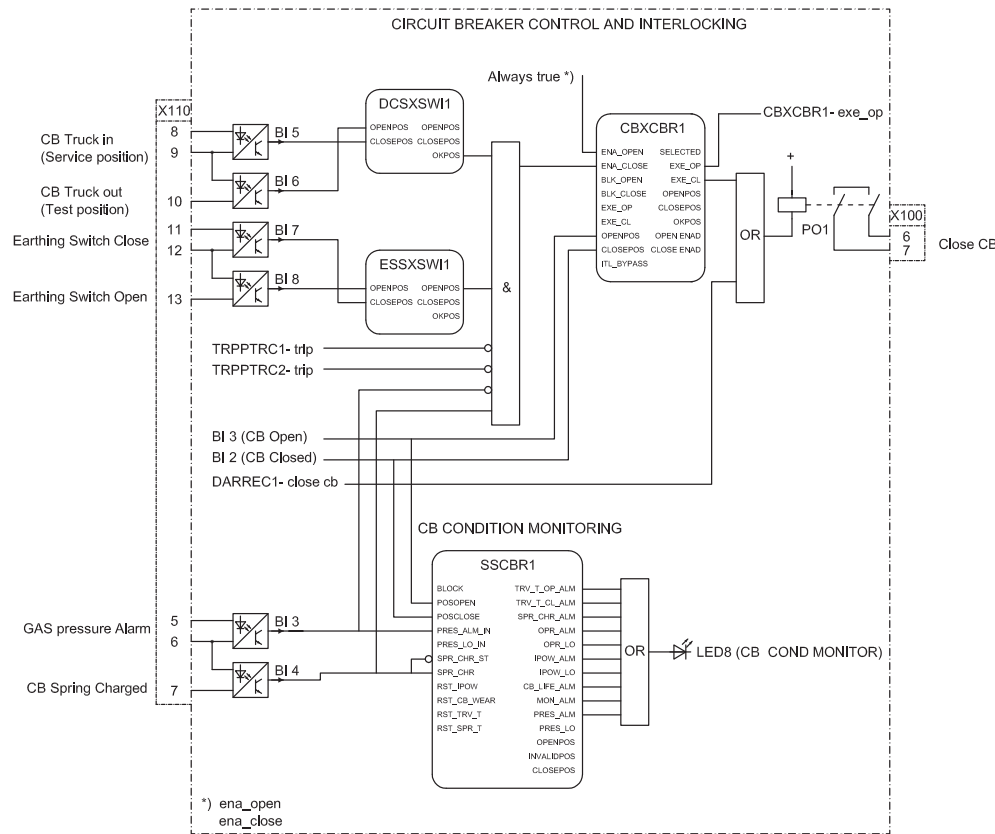
Figure 29: Circuit breaker control
