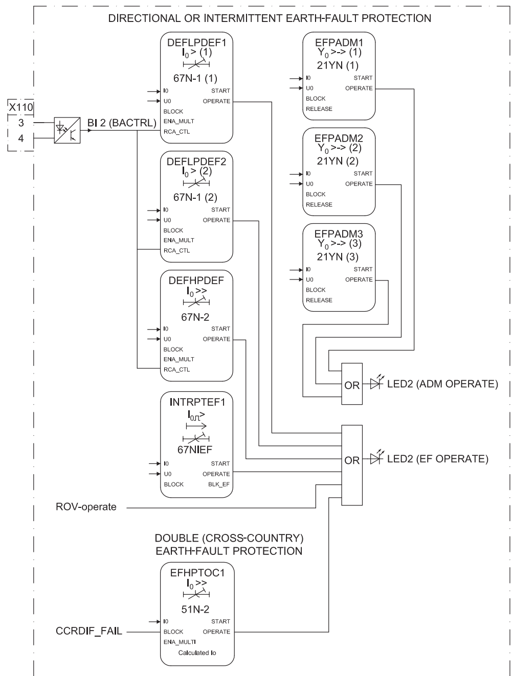
Figure 58: Directional earth-fault protection
