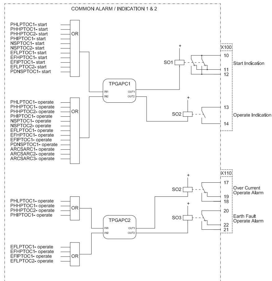
Figure 46: Alarm indication
