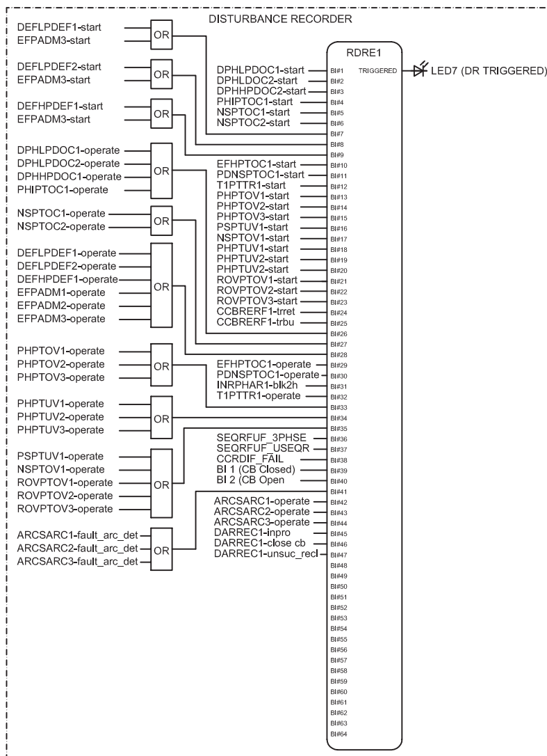
Figure 79: Disturbance recorder
