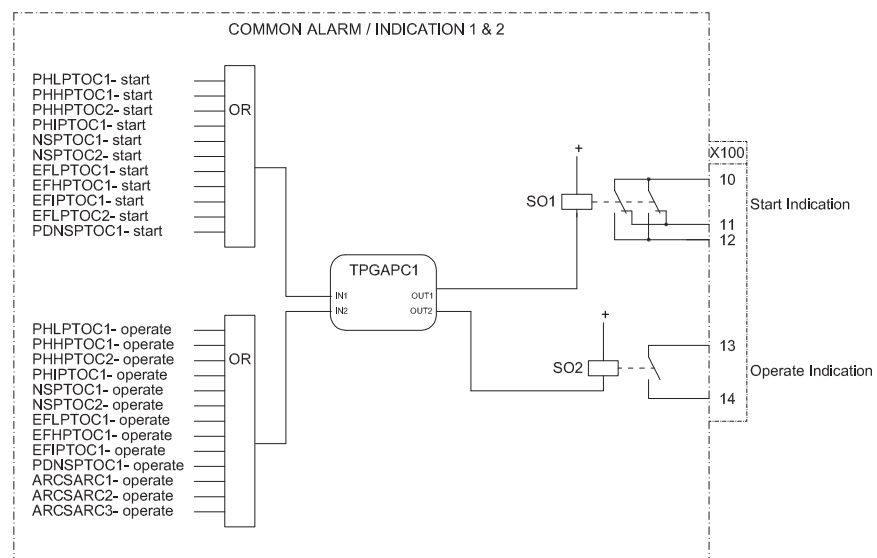
Figure 38: Alarm indication
