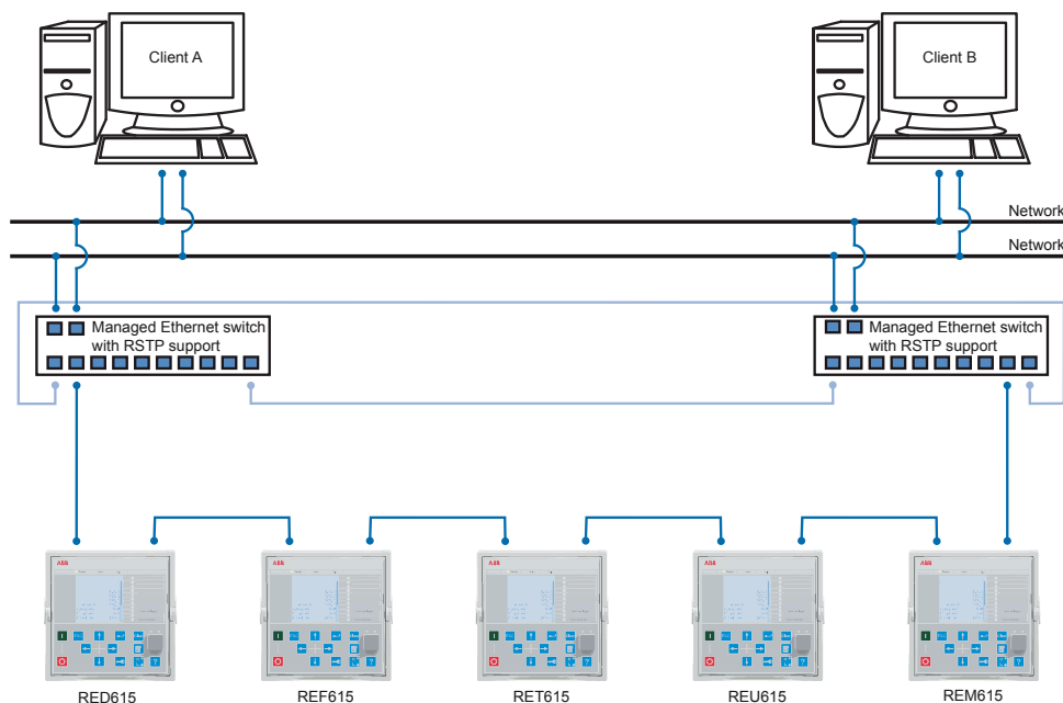
Figure 6: Redundant Ethernet solution
