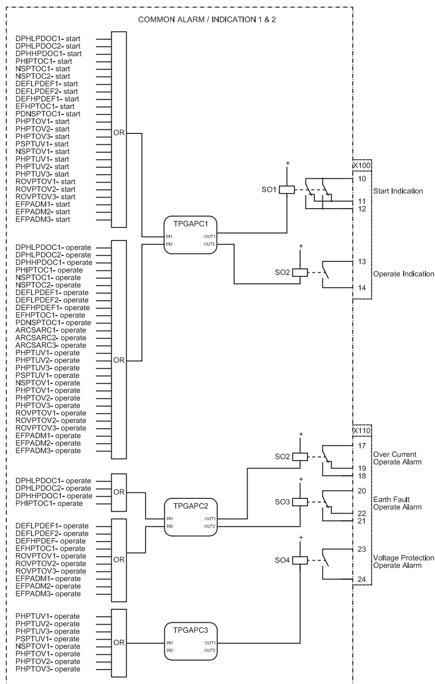
Figure 83: Alarm indication
