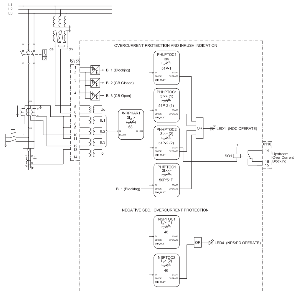
Figure 22: Overcurrent protection
