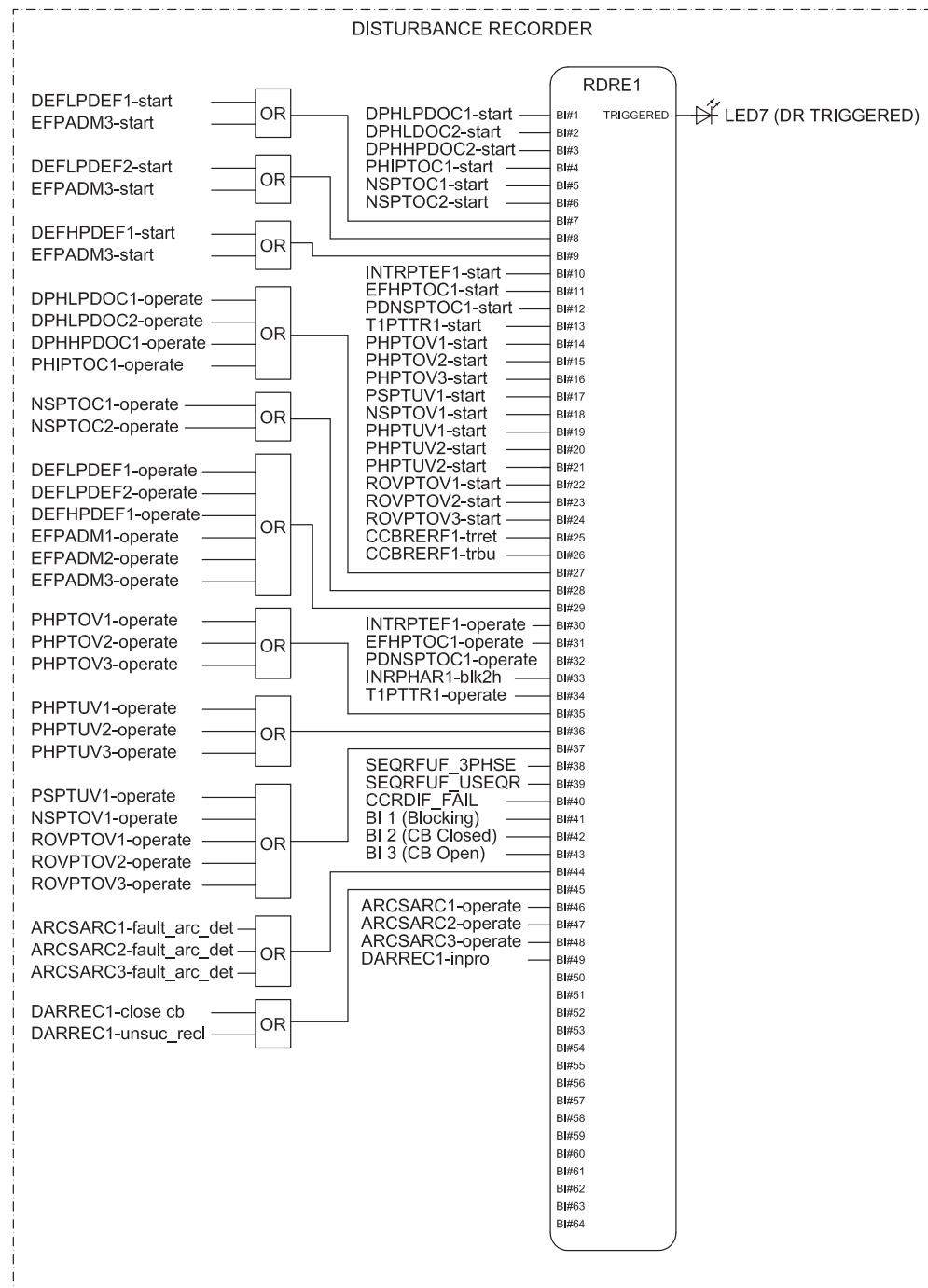
Figure 64: Disturbance recorder
