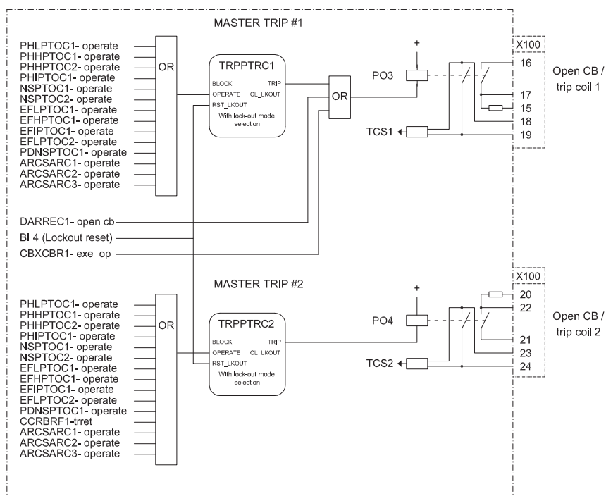
Figure 44: Master trip
