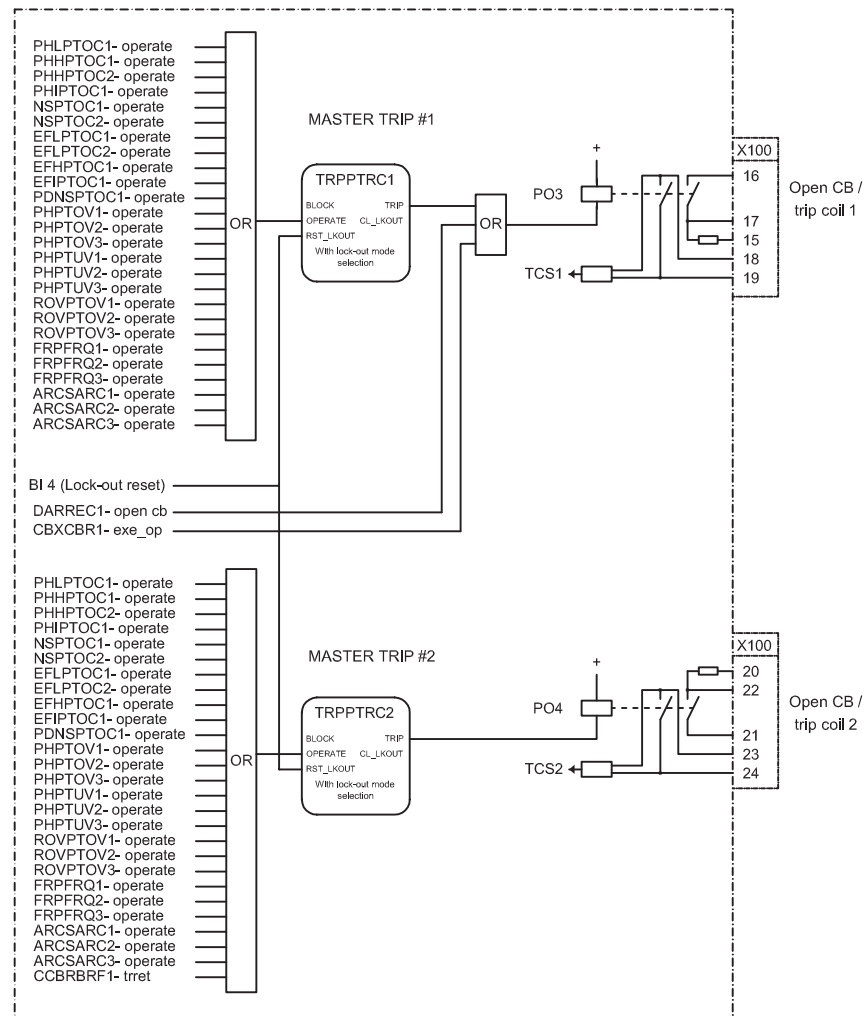
Figure 96: Master trip
