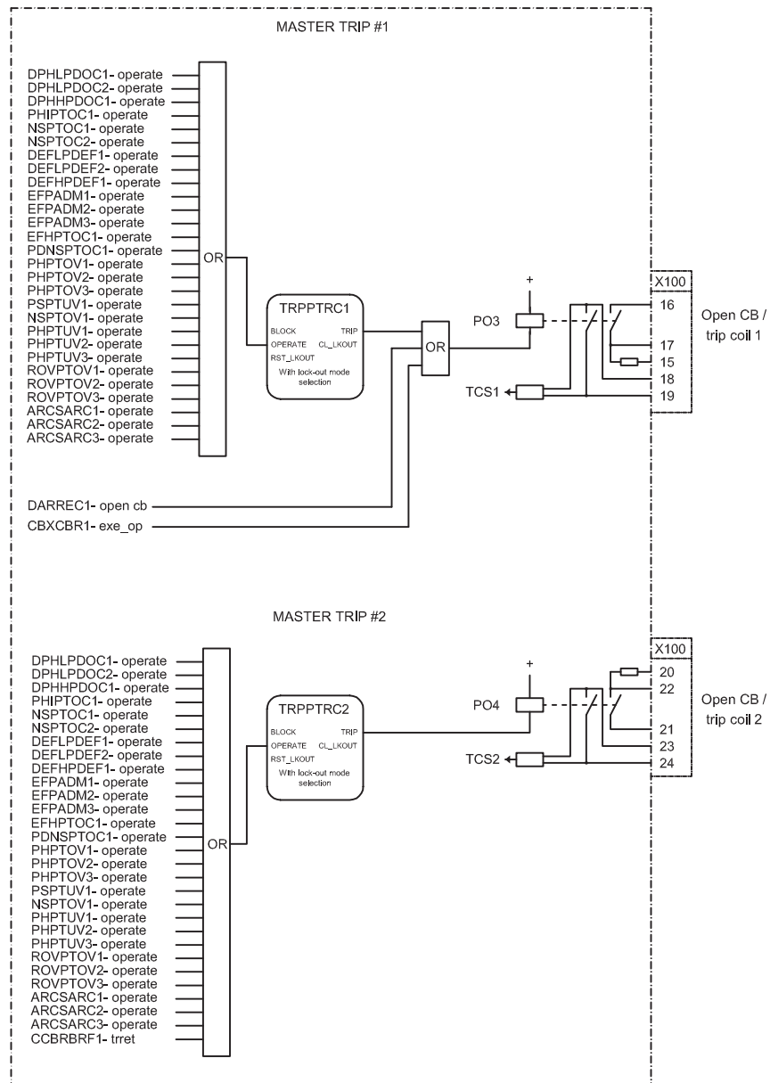
Figure 81: Master trip
