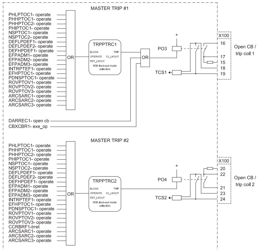
Figure 19: Master trip
