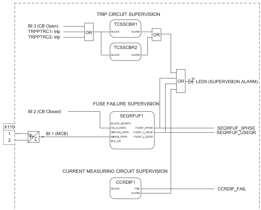
Figure 65: Trip circuit supervision
