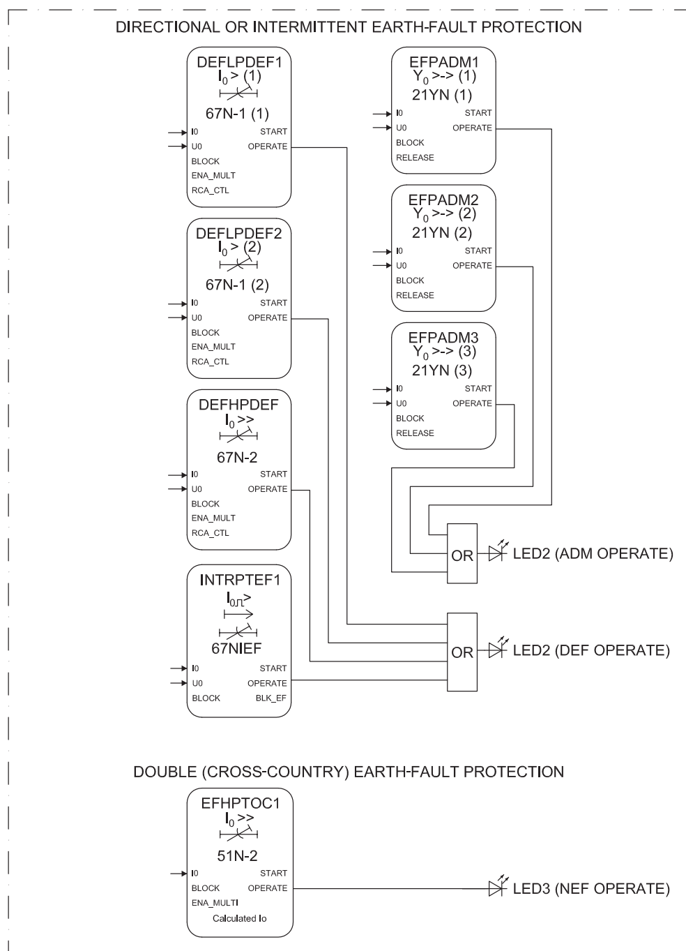
Figure 14: Directional earth-fault protection
