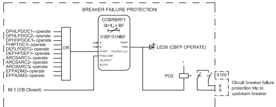
Figure 73: Circuit breaker failure protection
