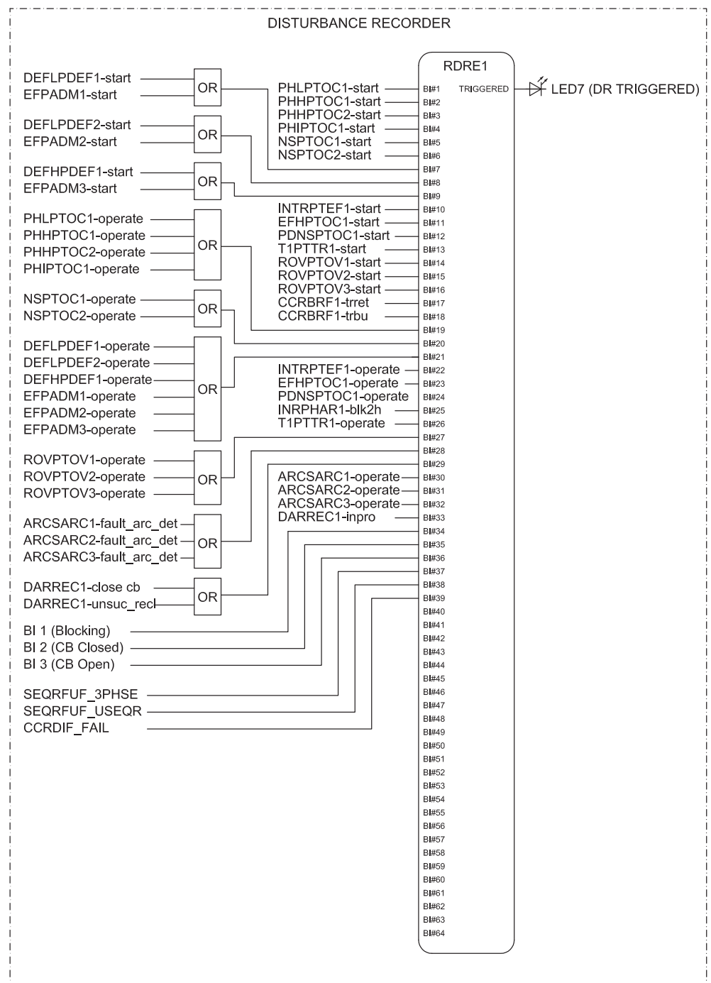
Figure 52: Disturbance recorder
