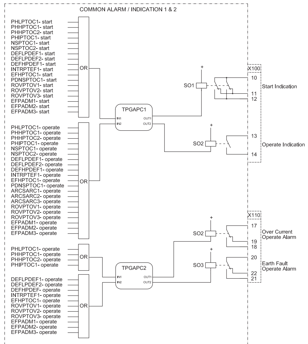
Figure 56: Alarm indication
