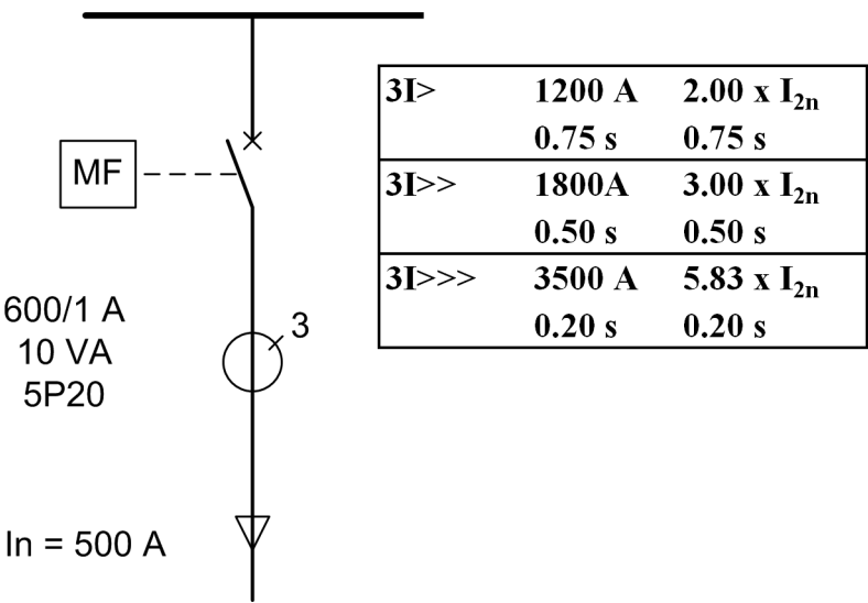
Figure 99: Example of three-stage overcurrent protection
