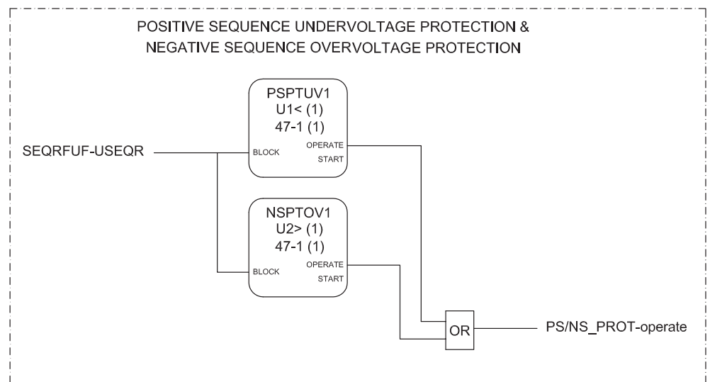
Figure 62: Positive-sequence undervoltage and negative-sequence overvoltage protection
