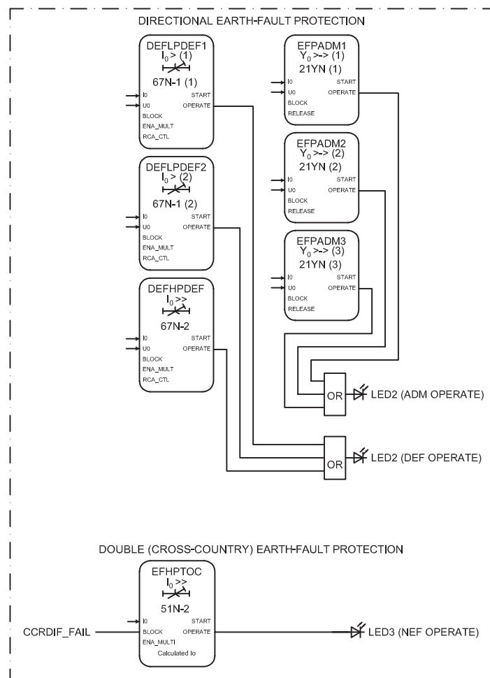
Figure 70: Directional earth-fault protection
