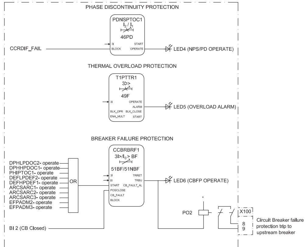
Figure 59: Phase discontinuity, thermal overload and circuit breaker failure protection
