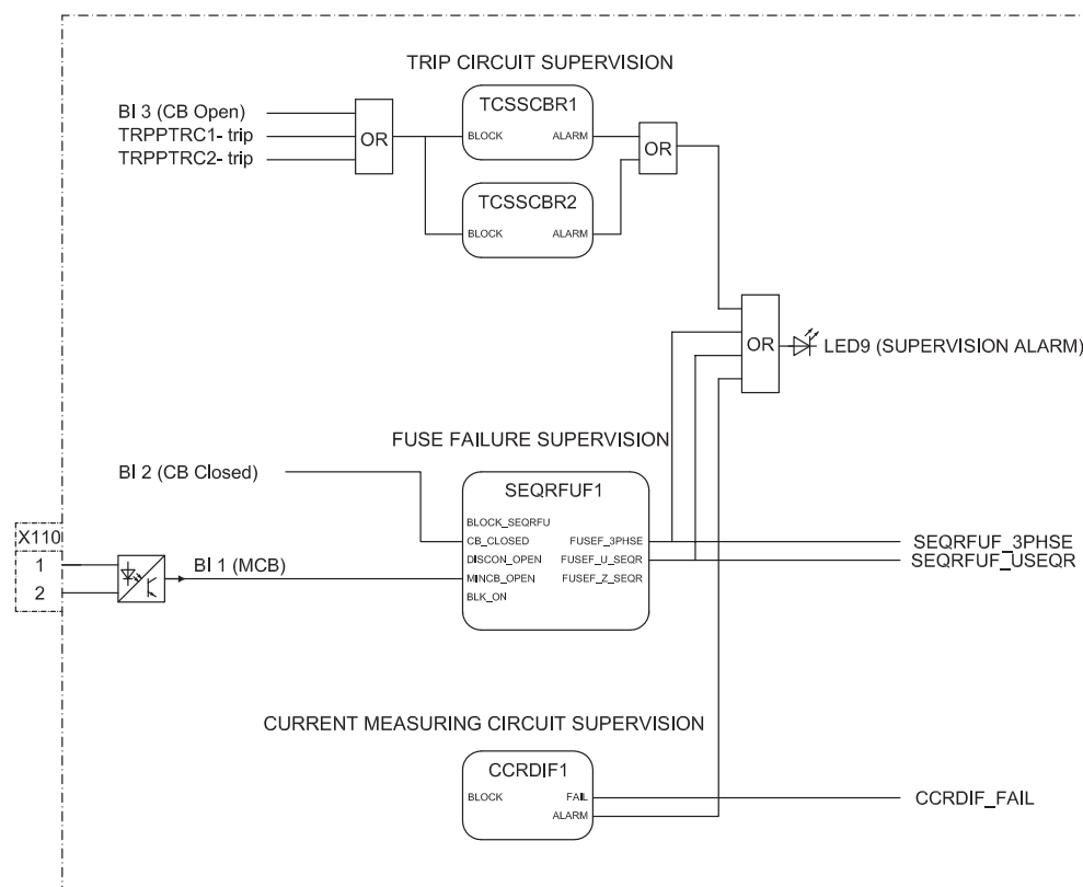
Figure 53: Trip circuit supervision
