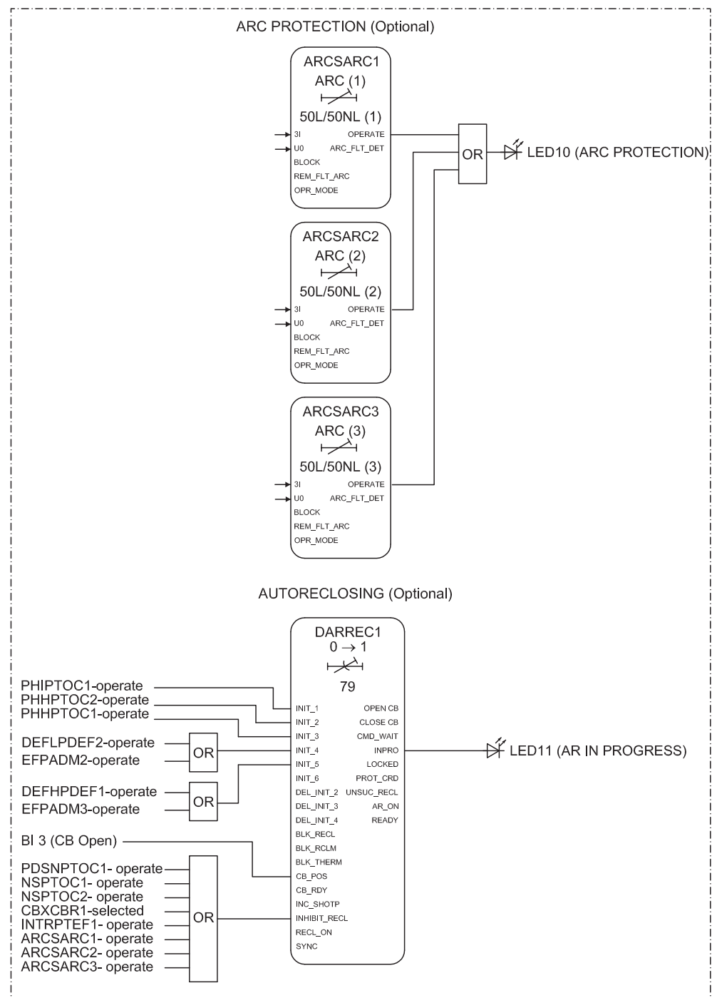
Figure 17: Arc protection
