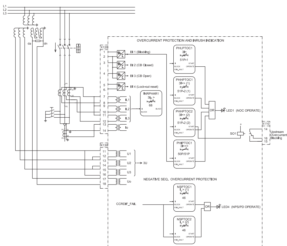
Figure 47: Overcurrent protection
