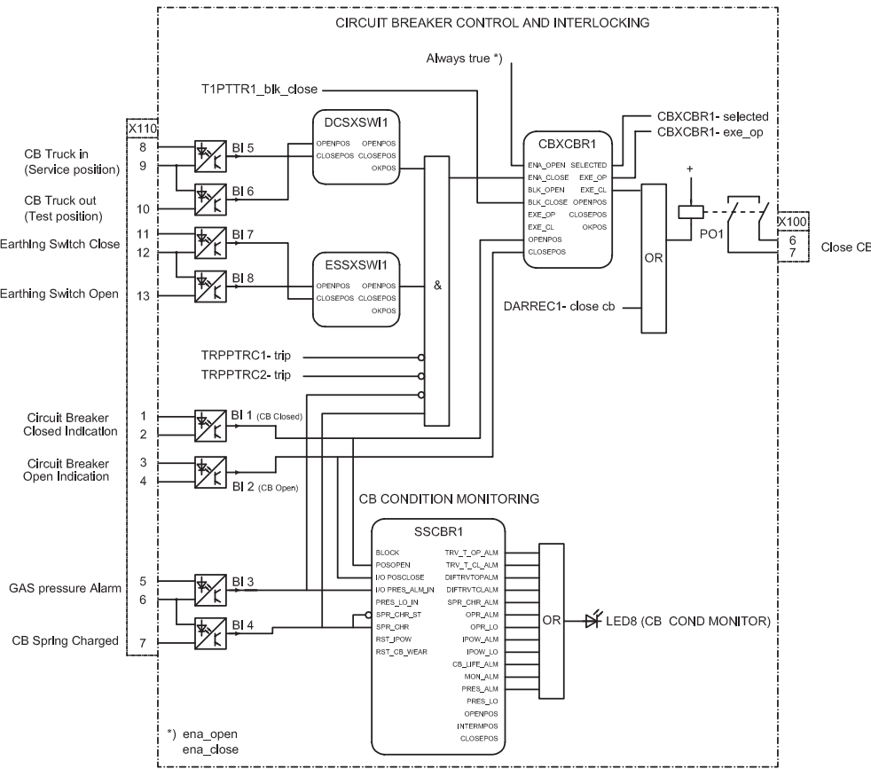
Figure 82: Circuit breaker control
