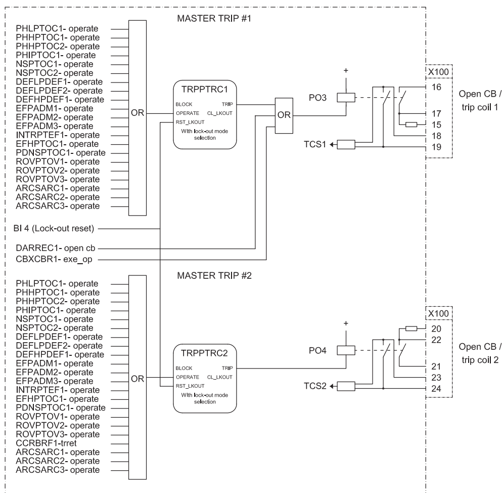
Figure 54: Master trip
