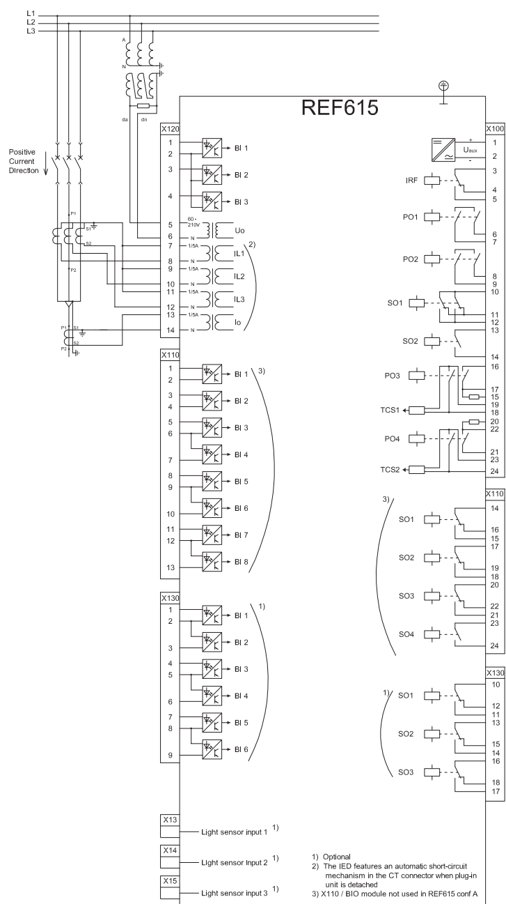
Figure 7: Connection diagram for the A and B configurations [1]
