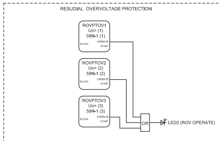
Figure 78: Residual overvoltage protection
