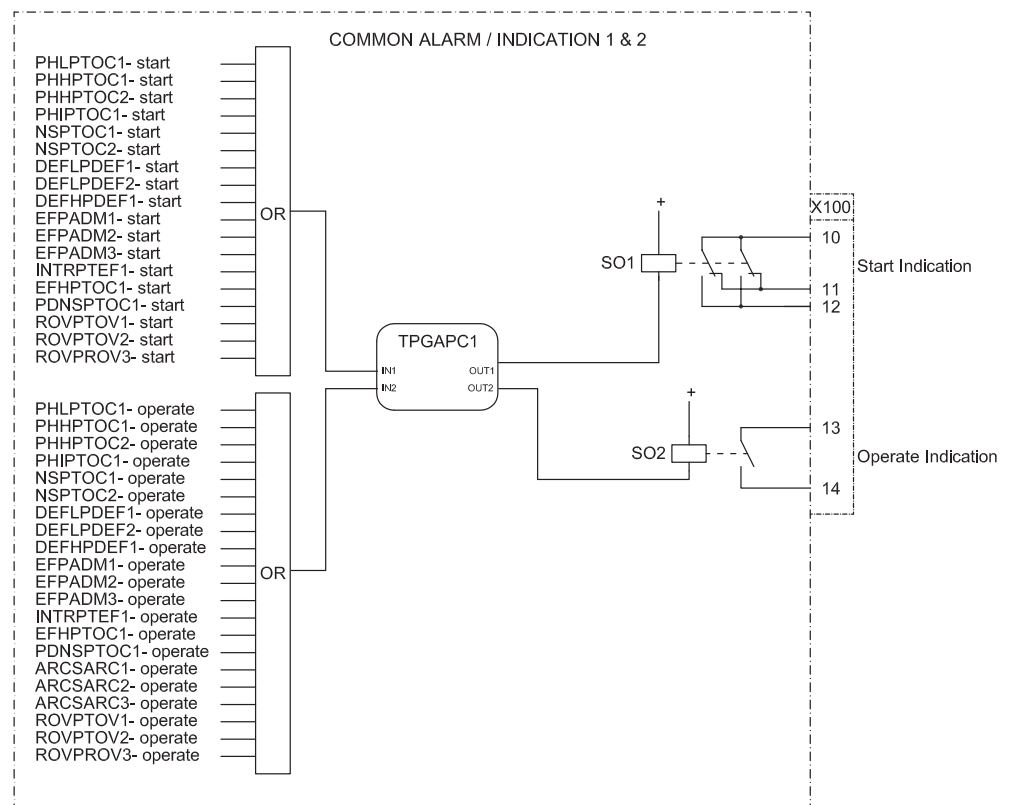
Figure 21: Alarm indication
