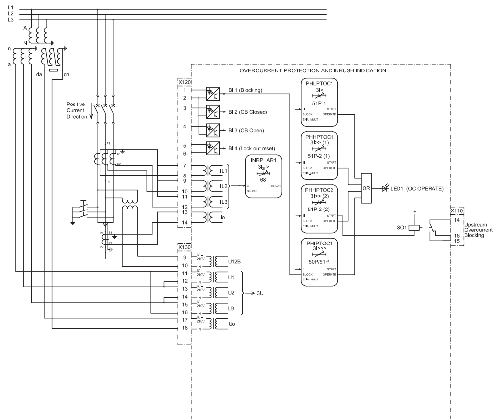
Figure 84: Non-directional overcurrent protection
