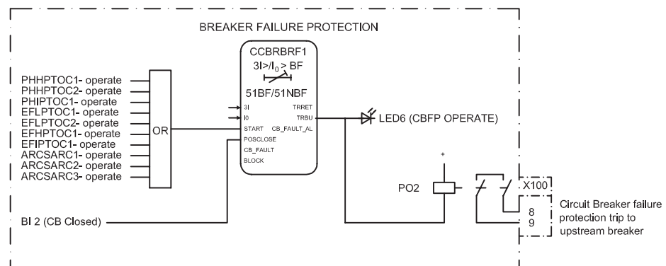
Figure 87: Circuit breaker failure protection
