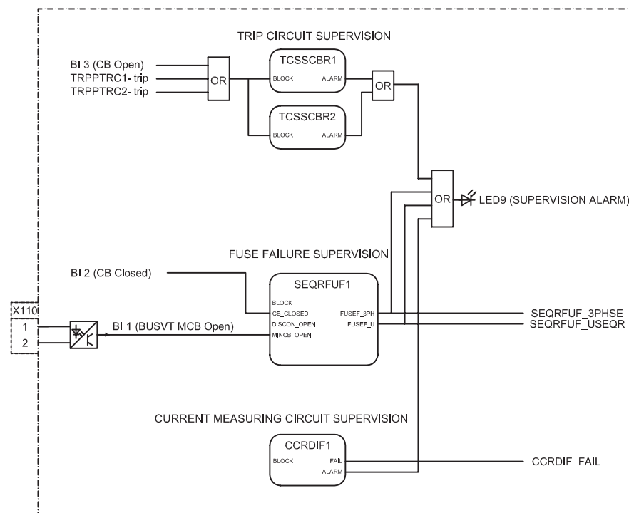
Figure 94: Trip circuit supervision
