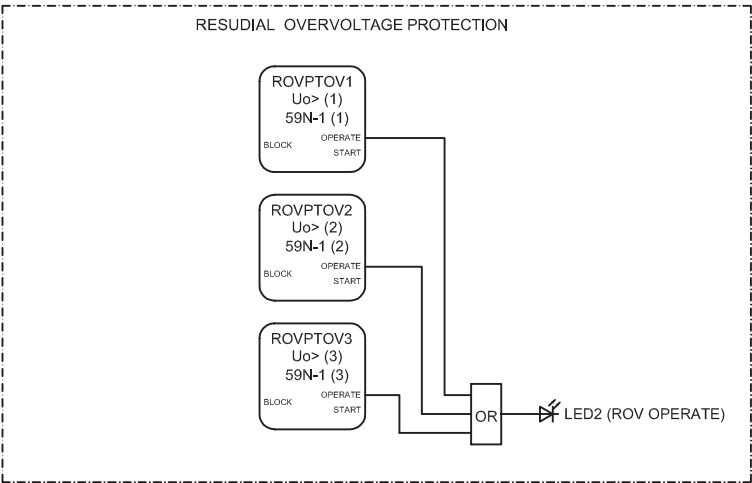
Figure 91: Residual overvoltage protection
