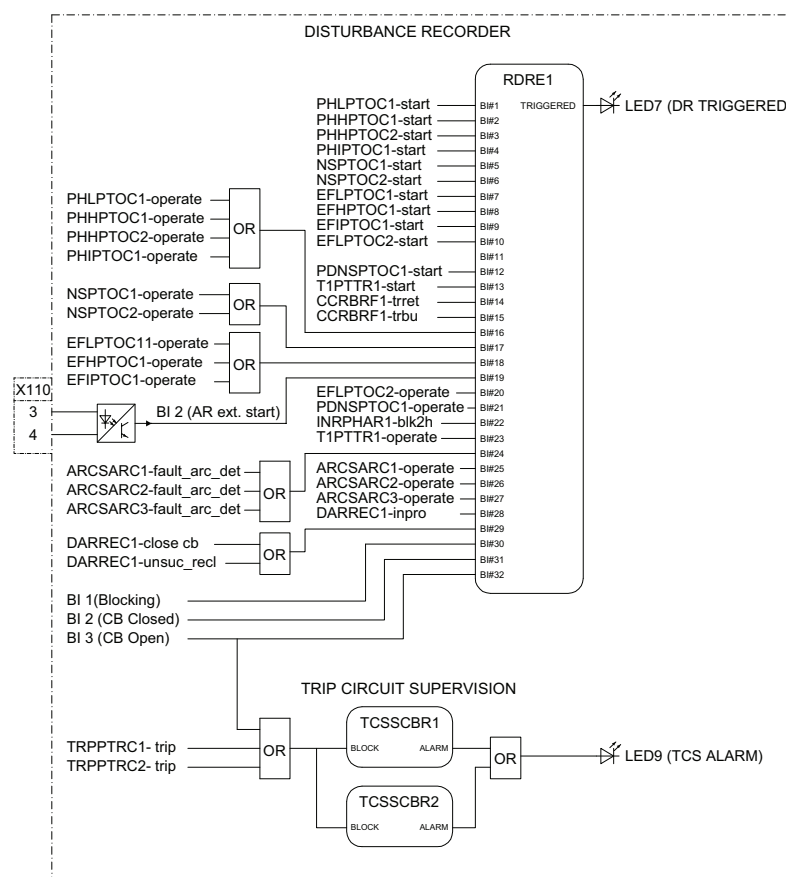
Figure 43: Disturbance recorder
