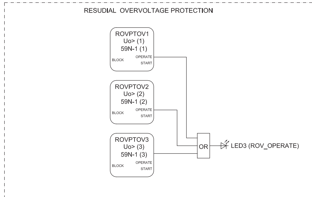
Figure 24: Residual overvoltage protection
