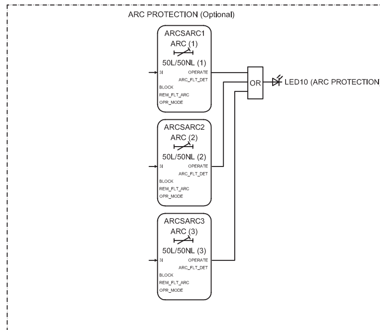
Figure 88: Arc protection
