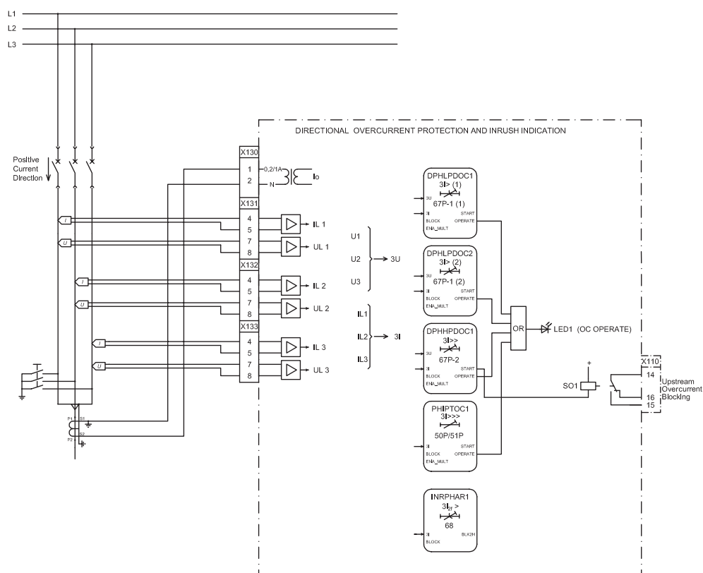
Figure 69: Directional overcurrent protection
