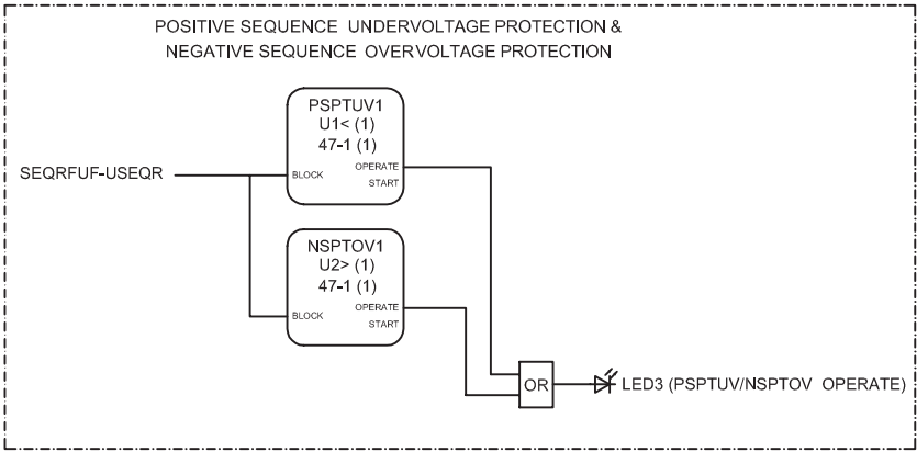
Figure 77: Positive-sequence undervoltage and negative-sequence overvoltage protection
