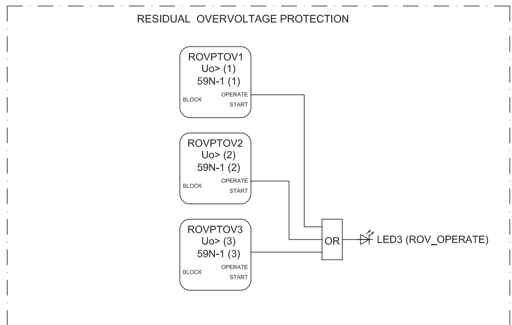
Figure 49: Residual overvoltage protection
