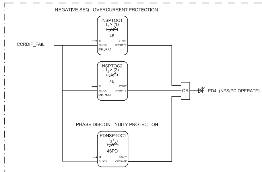
Figure 72: Negative sequence and phase discontinuity protection
