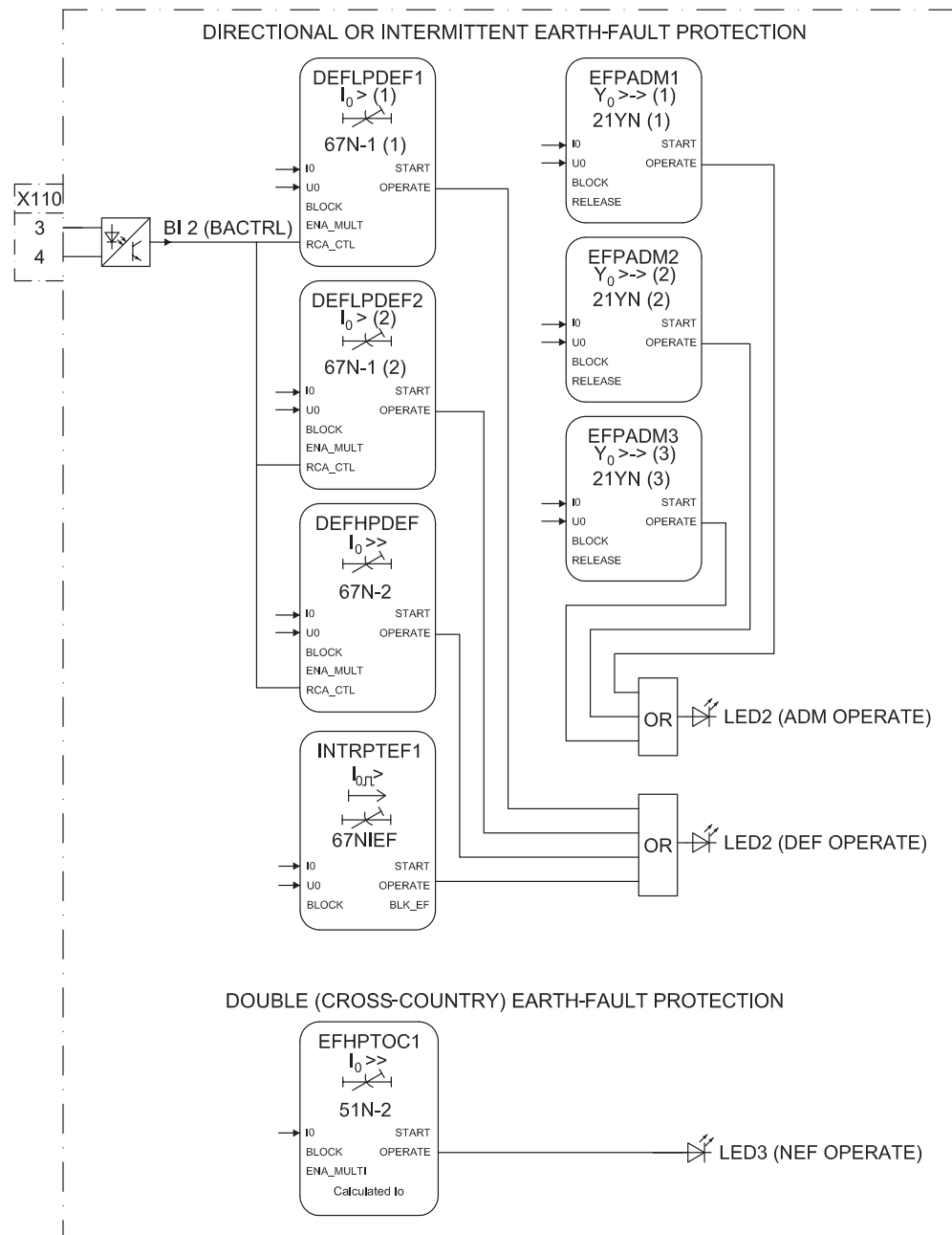
Figure 48: Directional earth-fault protection
