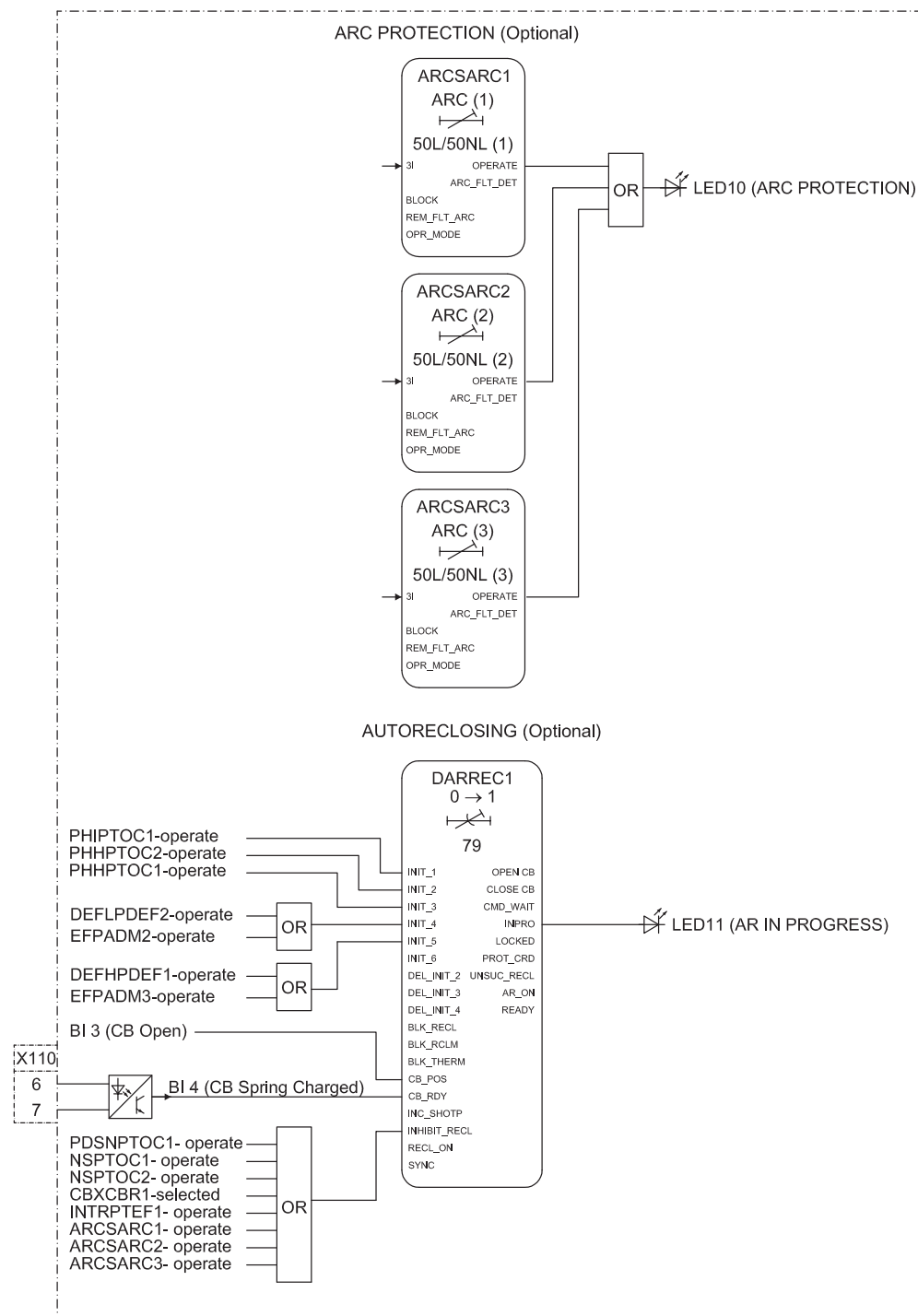
Figure 26: Arc protection
