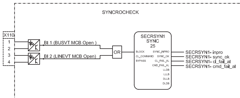
Figure 95: Synchrocheck
