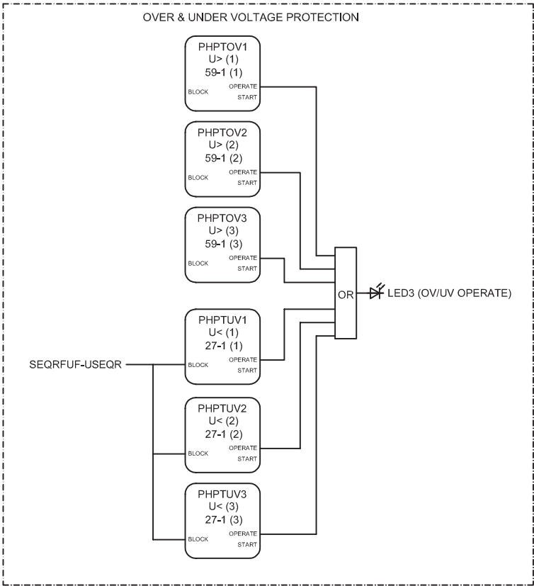
Figure 76: Overvoltage and undervoltage protection
