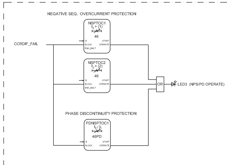
Figure 86: Negative sequence and phase discontinuity protection
