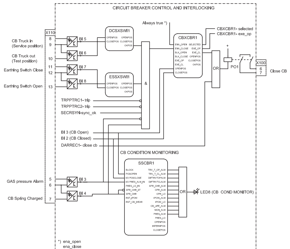
Figure 97: Circuit breaker control
