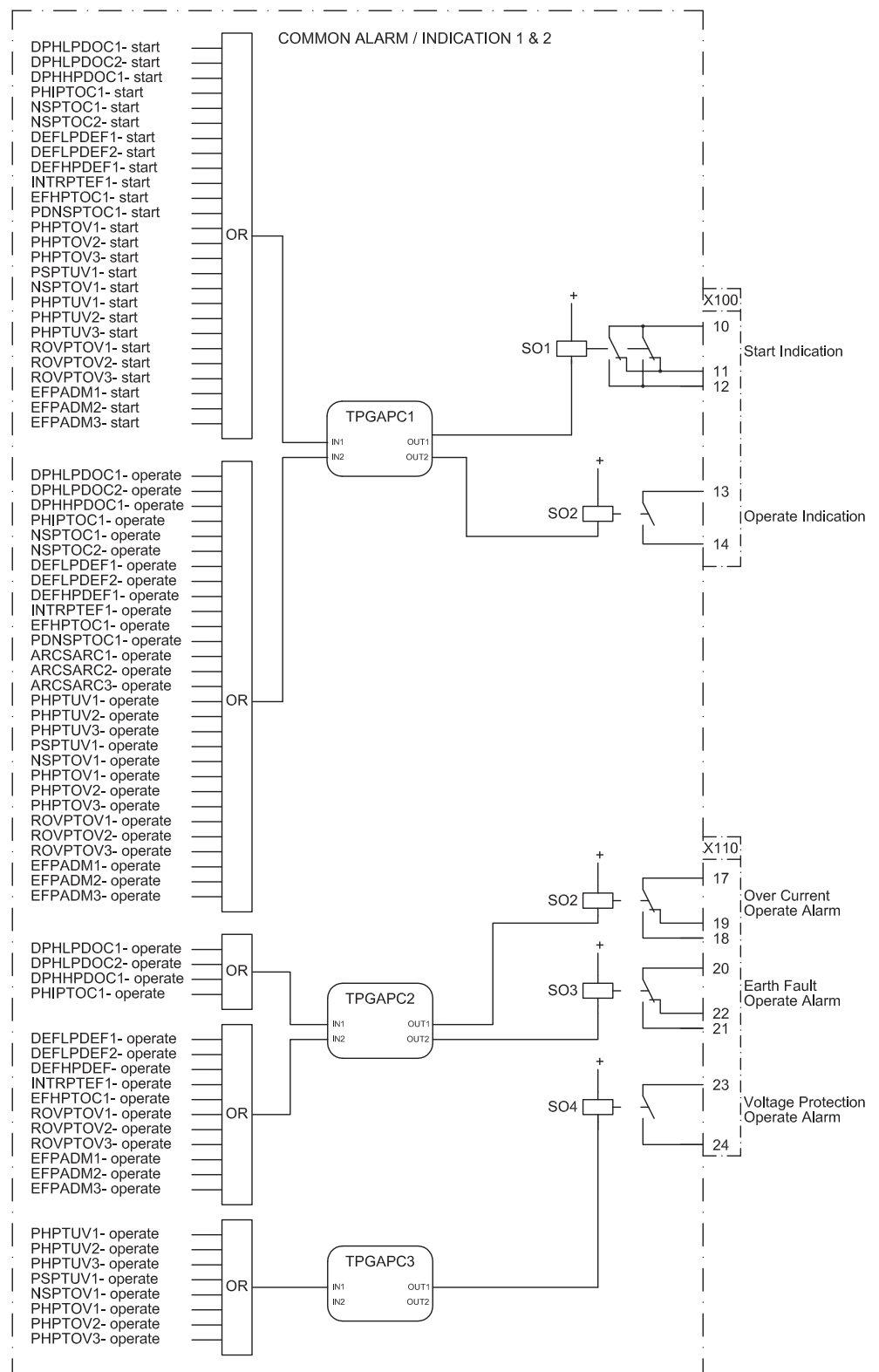
Figure 68: Alarm indication
