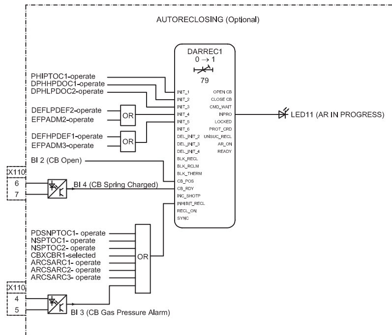
Figure 75: Autoreclosing
