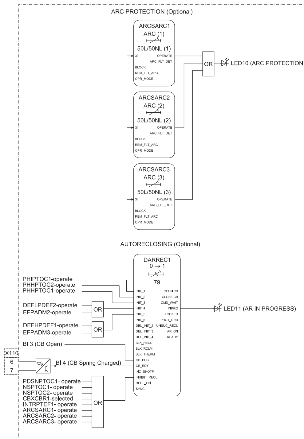
Figure 51: Arc protection
