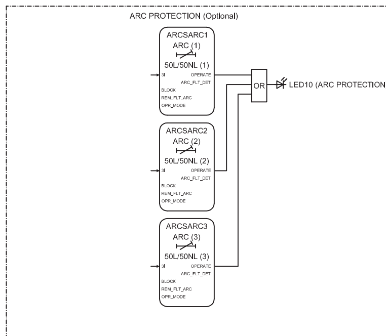
Figure 74: Arc protection
