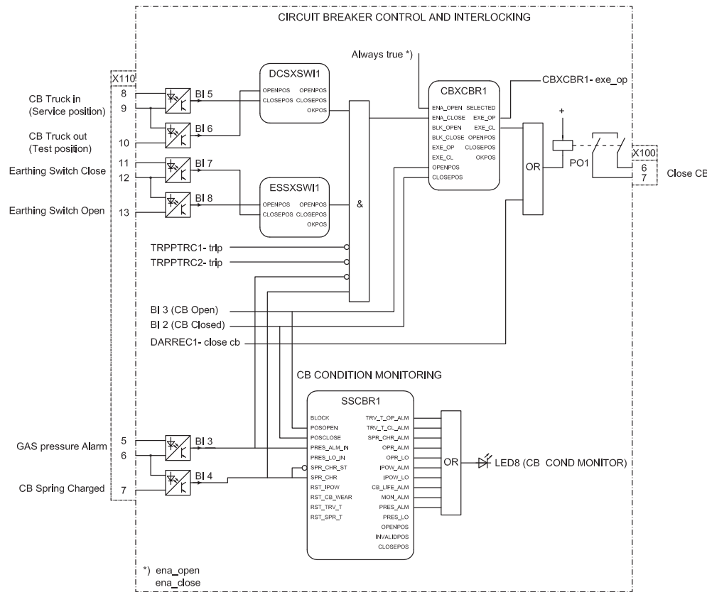
Figure 55: Circuit breaker control
