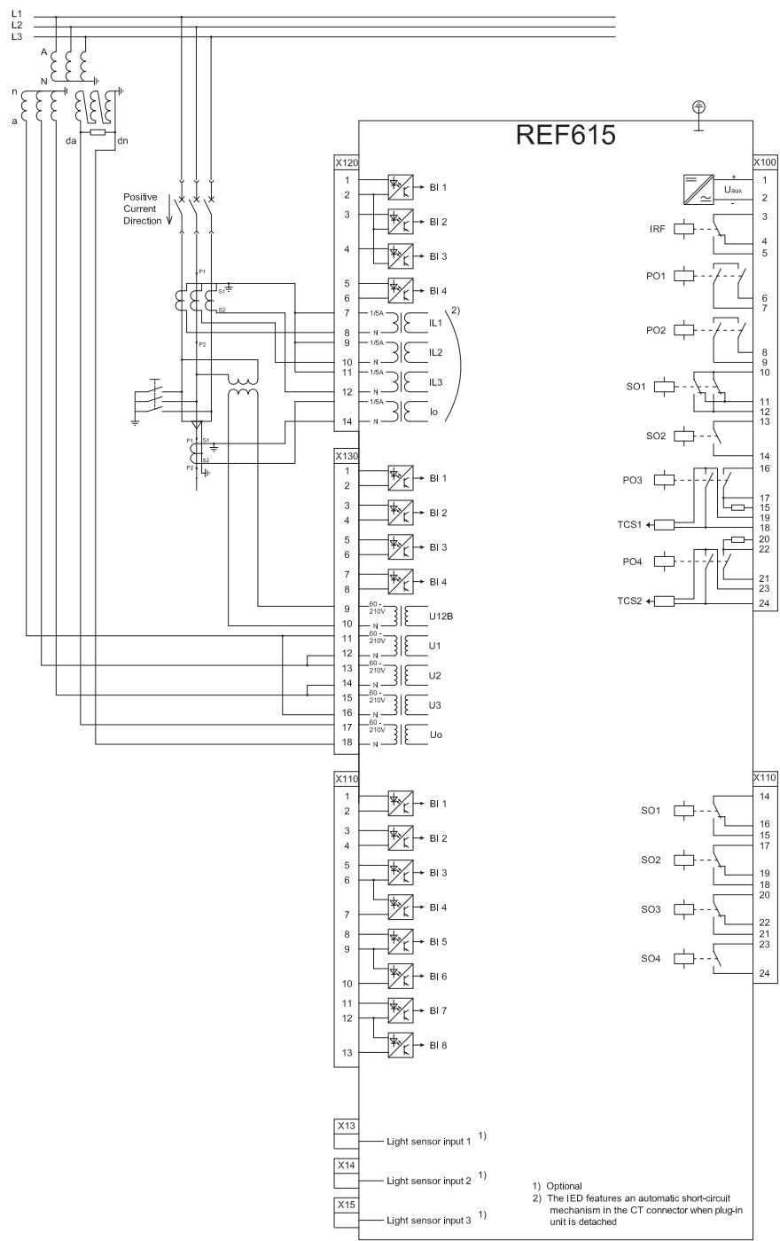
Figure 12: Connection diagram for the H configuration
