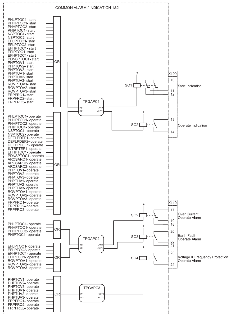
Figure 98: Alarm indication
