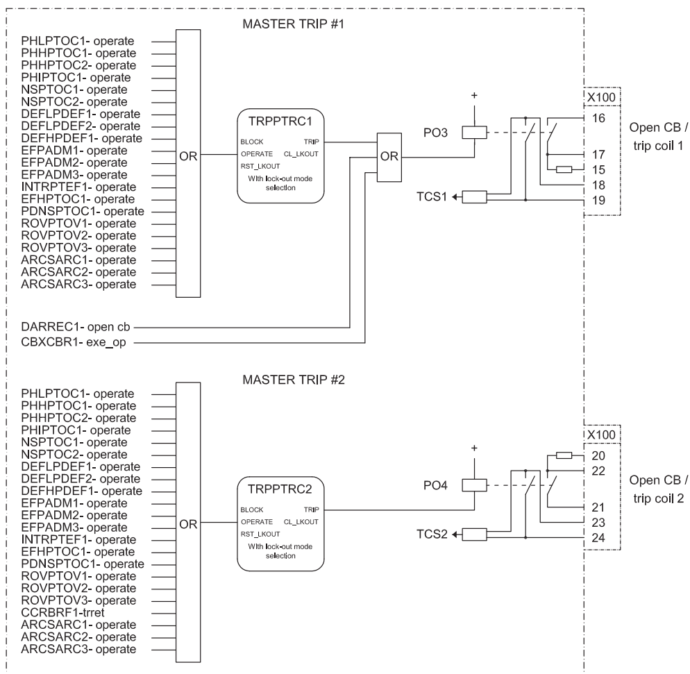
Figure 28: Master trip
