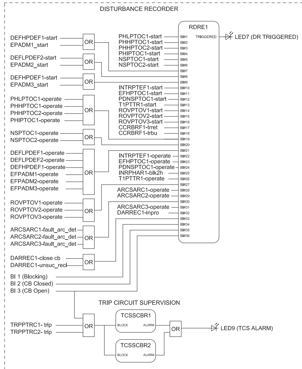
Figure 18: Disturbance recorder
