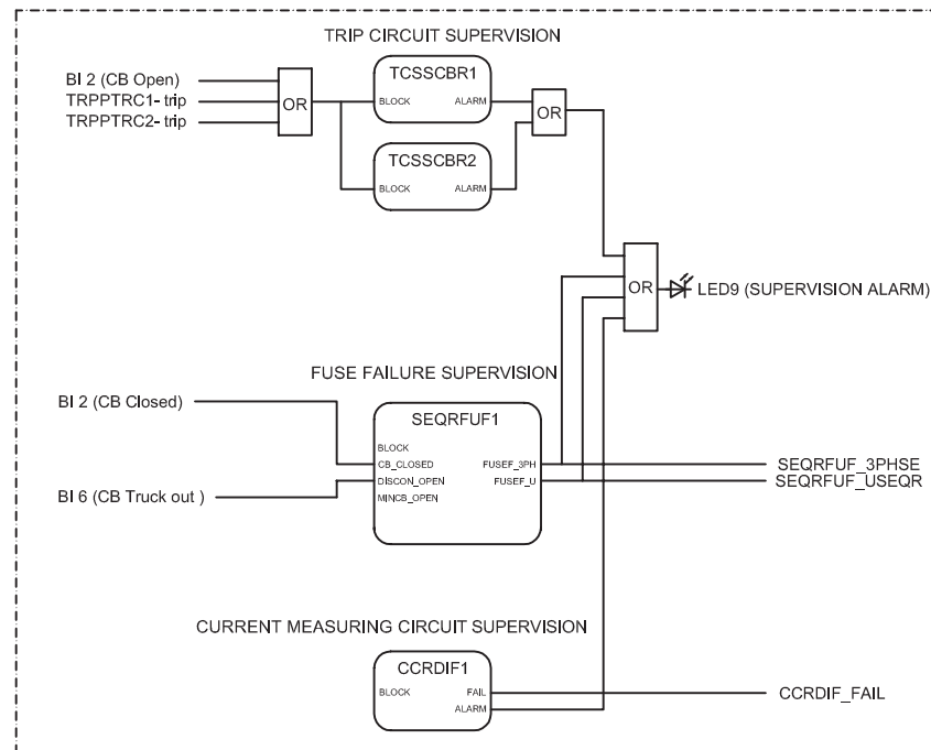
Figure 80: Trip circuit supervision
