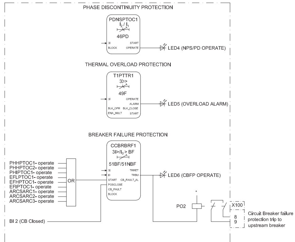
Figure 41: Phase discontinuity, thermal overload and circuit breaker failure protection
