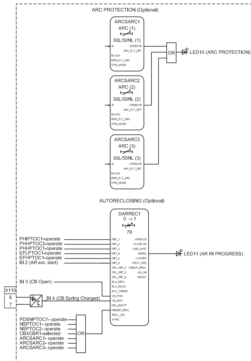
Figure 42: Arc protection
