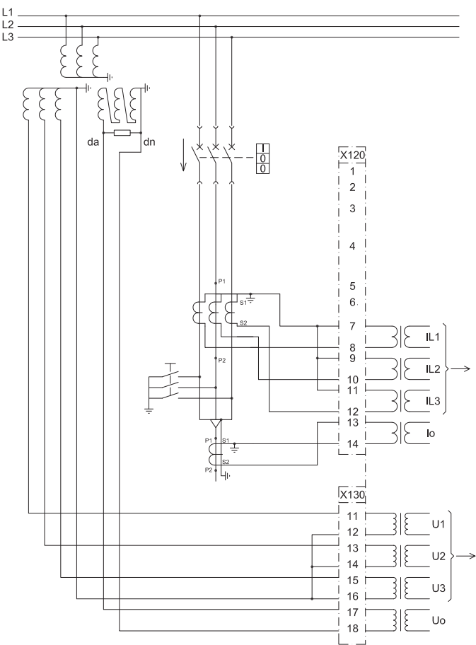
Figure 10: Connection diagram for the E and F configurations
