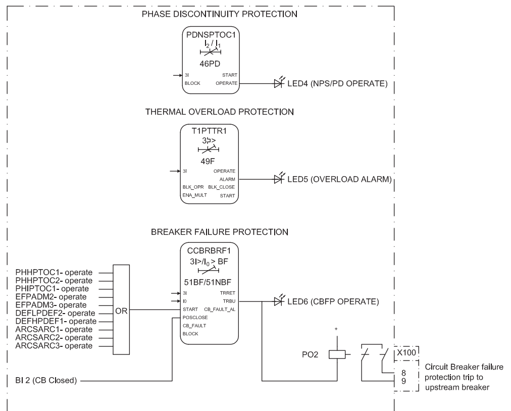
Figure 16: Phase discontinuity, thermal overload and circuit breaker failure protection
