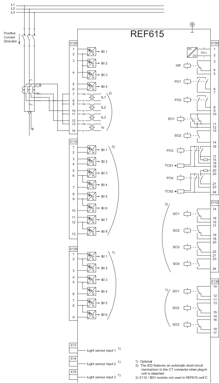
Figure 8: Connection diagram for the C and D configurations [2]
