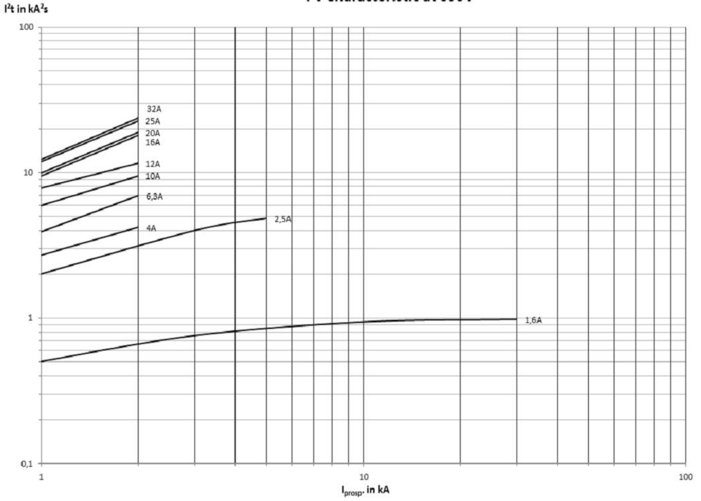
I 2 t-Characteristic at 690V
