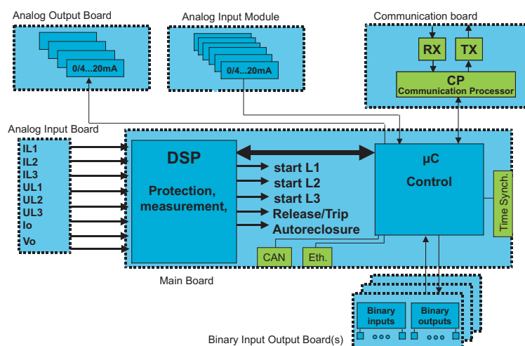
Fig. 3.-4 REF 542plus block diagram
