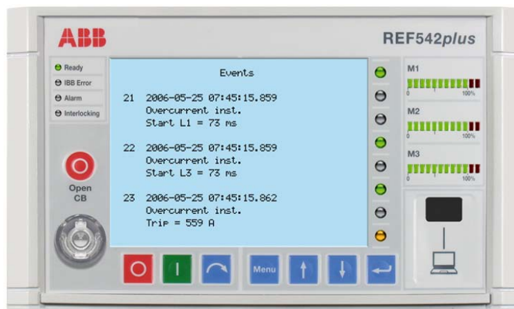
Fig. 4.5.-1 Event list on the LCD of the HMI
