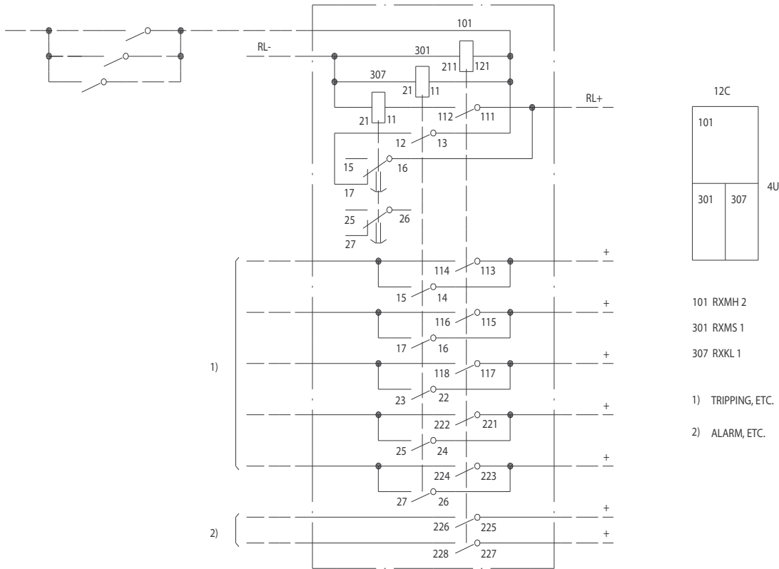
Figure 5. High-speed tripping assembly, RK 651 231-AB, Diagram No. 5651 109-AB
