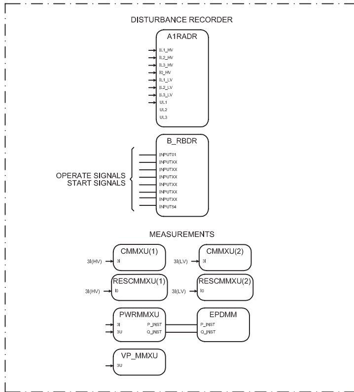
Figure 16: Measurement and analog recording
