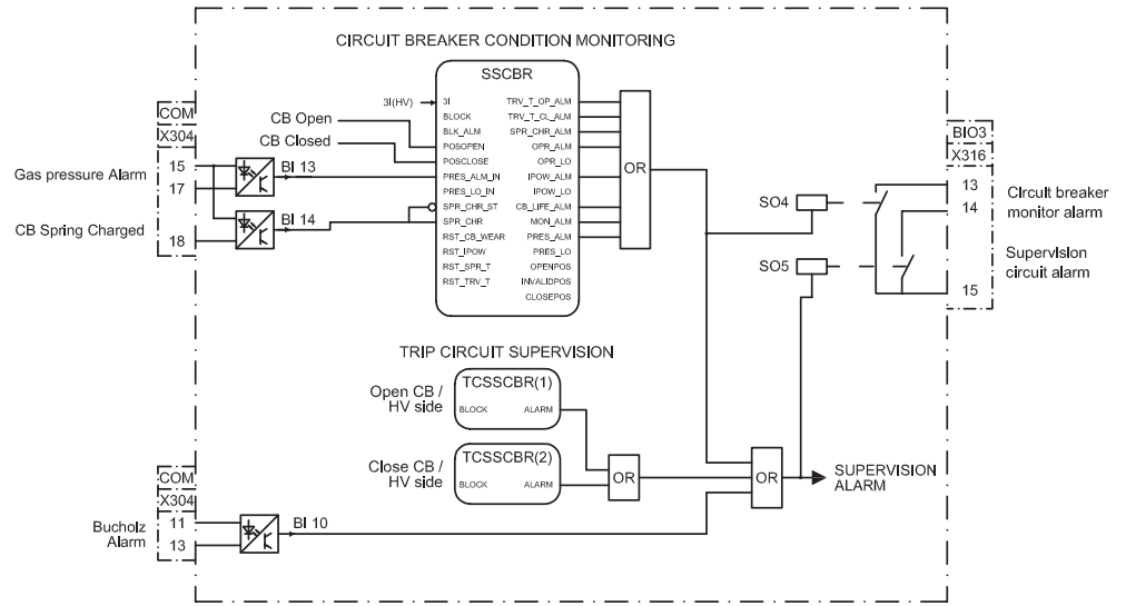
Figure 25: Circuit-breaker condition monitoring
