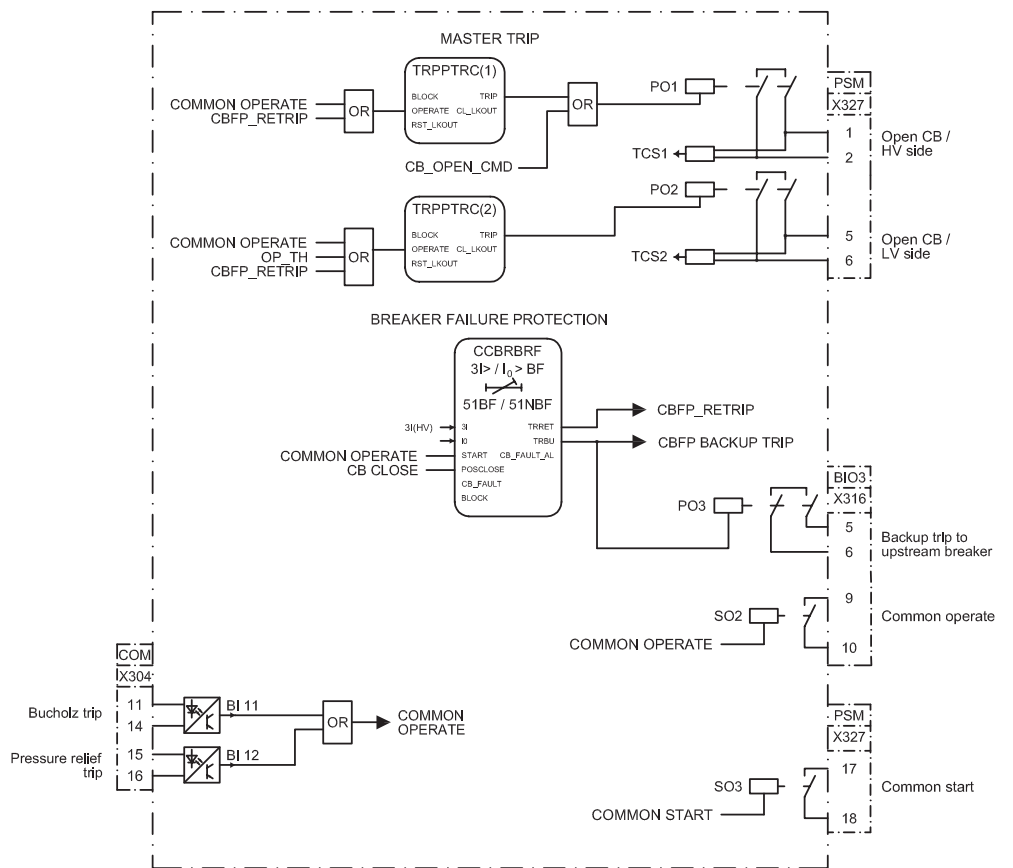
Figure 24: Tripping logic
