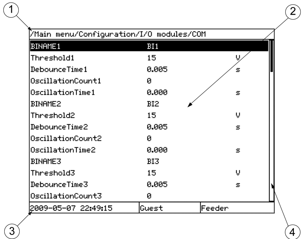
Figure 3: Display layout
