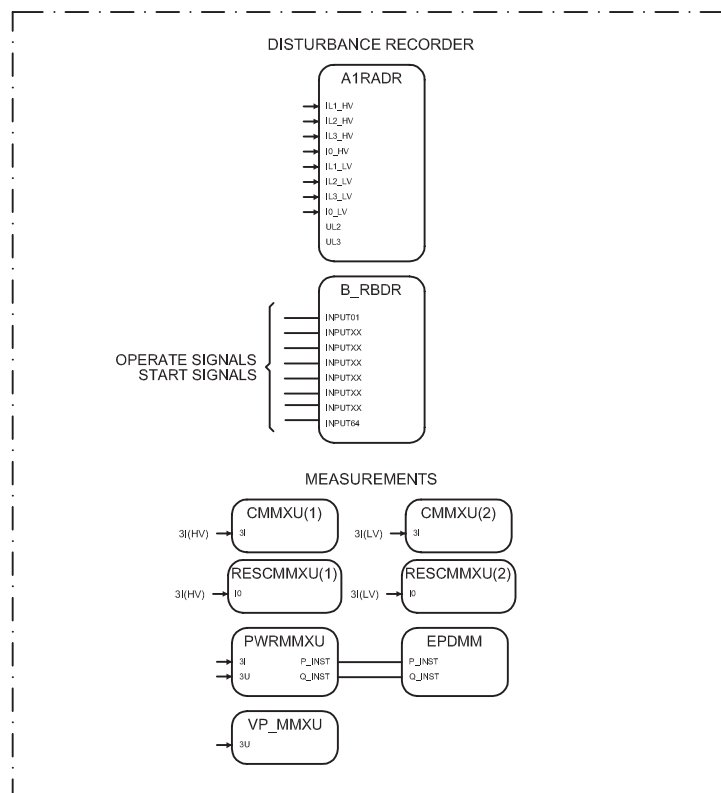
Figure 26: Measurement and analog recording
