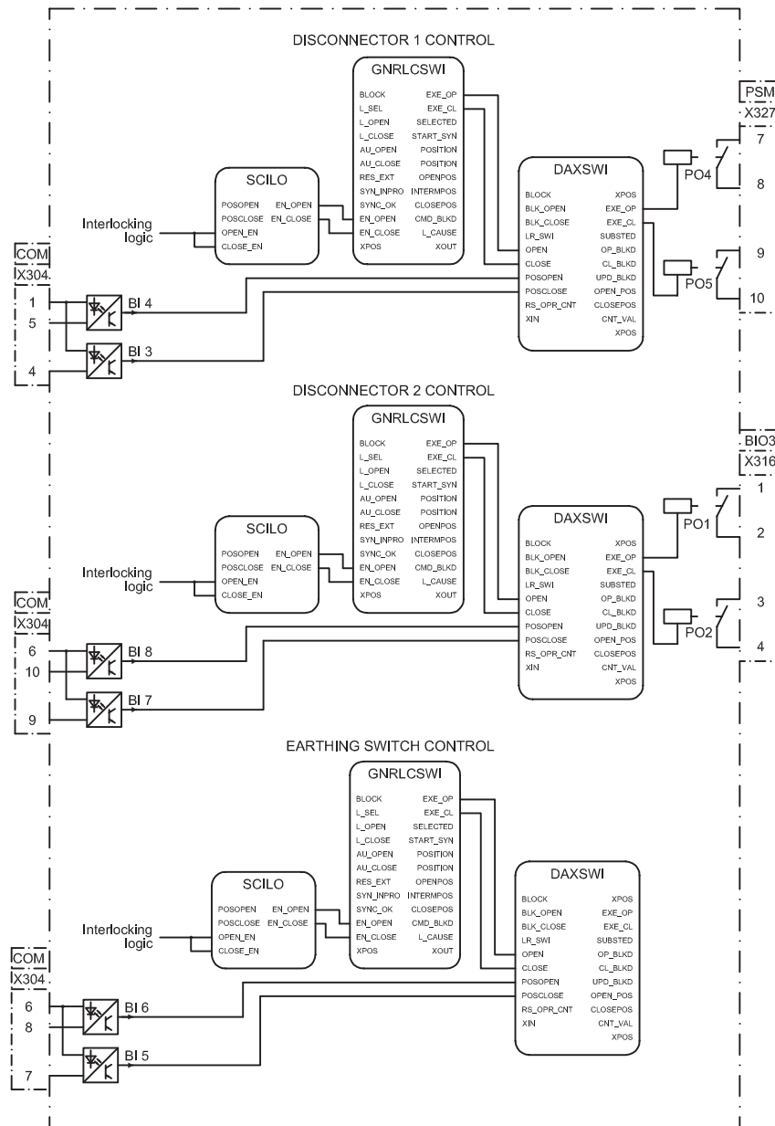
Figure 10: Disconnector control
