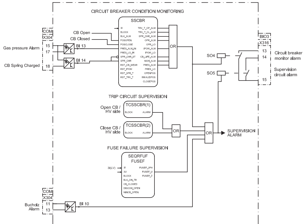
Figure 15: Circuit-breaker condition monitoring
