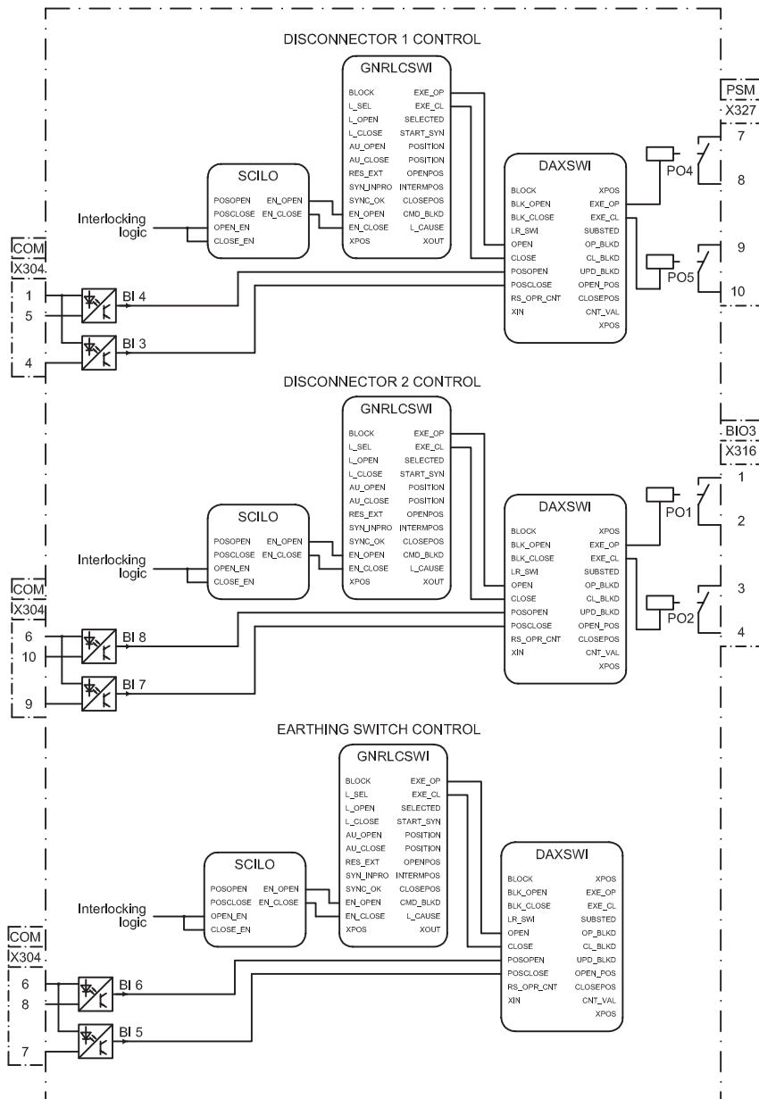
Figure 19: Disconnector control
