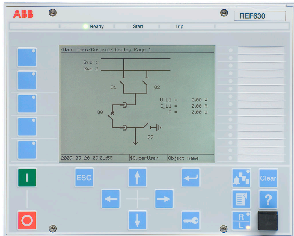
Figure 2: 19" LHMI
