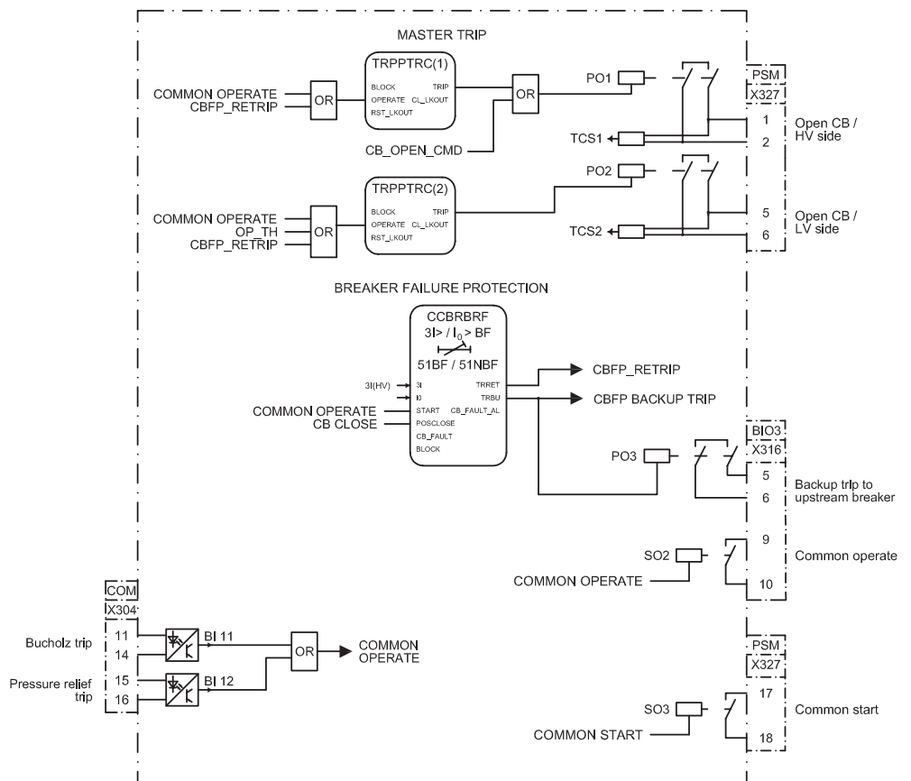
Figure 14: Tripping logic
