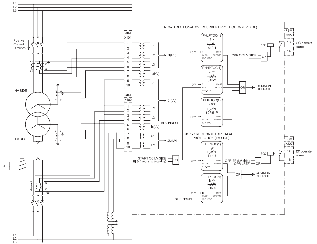
Figure 20: Non-directional overcurrent protection
