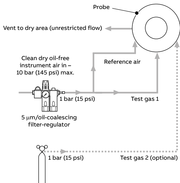
Figure 9 AutoCal with air supply and restrictors
