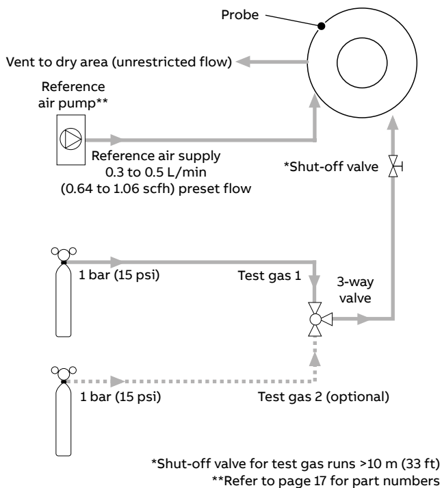
Figure 14 Non-AutoCal with test gas(es) and restrictors
