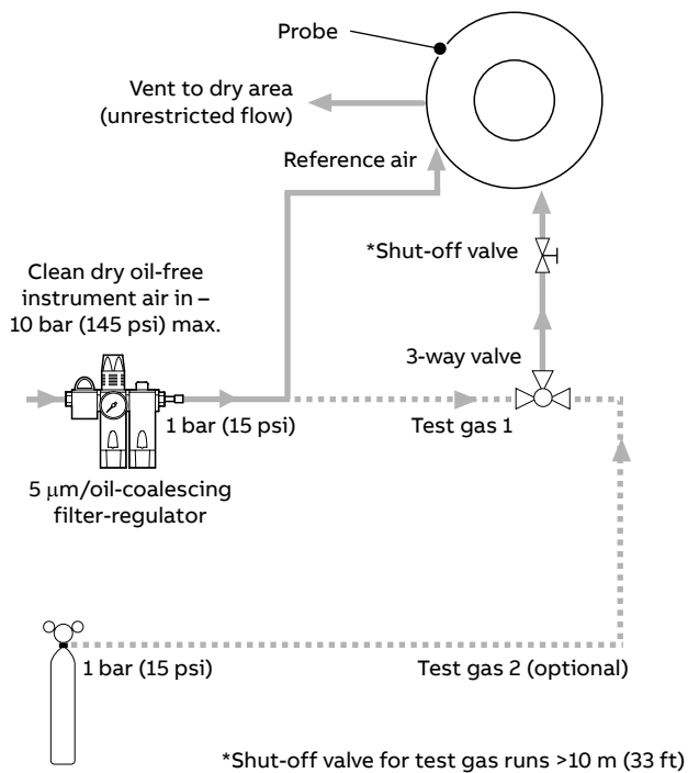
Figure 13 Non-AutoCal with air supply and restrictors
