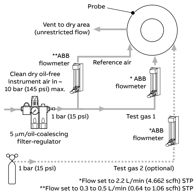
Figure 11 AutoCal with air supply and no restrictors
