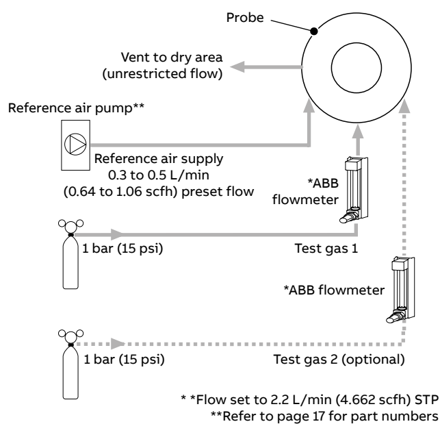
Figure 12 AutoCal with test gas(es) and no restrictors
