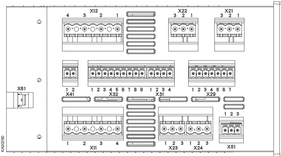
Figure 5.3 Connectors, OMD800
