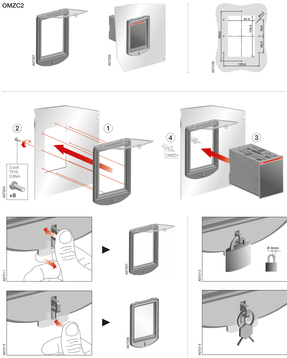
Figure 10.2 Door drilling and mounting of the cover plate OMZC2, when the automatic control unit OMD800 is mounted on the door
