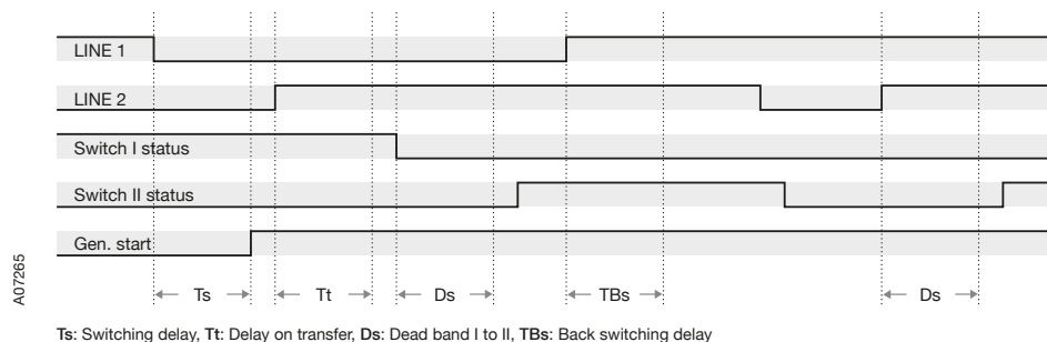
Figure 3.4 Automatic Switching Sequence, Manual back switching
