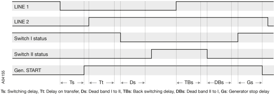
Figure 3.1 Automatic Switching Sequences in OMD800
