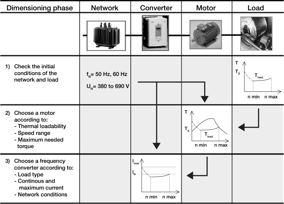
Figure 3.1 General description of the dimensioning procedure.
