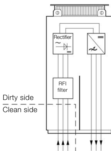
Figure 3-2 “Clean” and “dirty” sides of the BDM.
