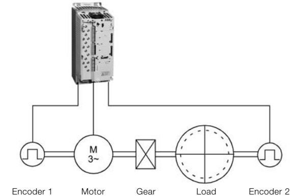
Figure 8.14 Both motor and load have an own encoder.
