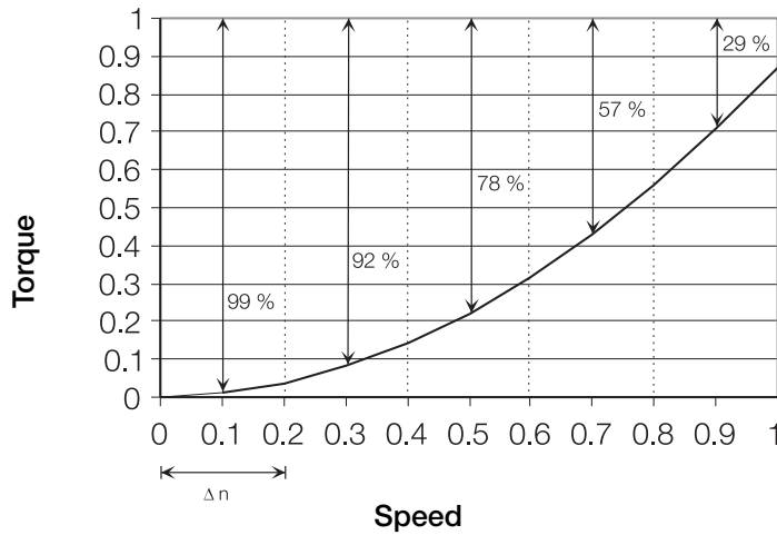
Figure 5.1 Torque characteristics of a fan. Speed and torque are shown using relative values.
