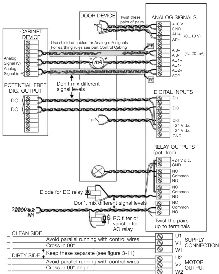
Figure 3-11 Principles of wiring inside CDM.
