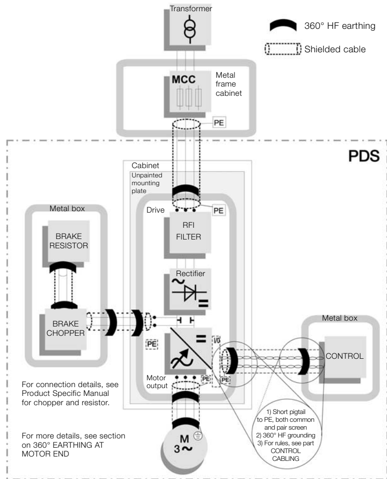
Figure 4-2 Typical PDS configuration.
