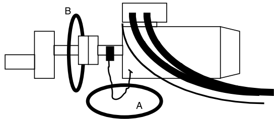
Figure 13: Basic measurements: A) circulating current measured with a jumper, B) shaft grounding current.
