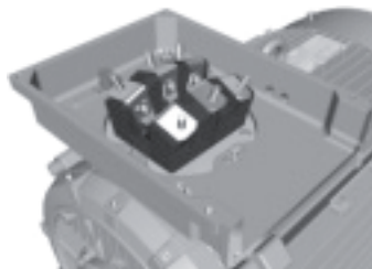
Terminal box for motor sizes 280 to 450, provided either with a cable gland or a cable box.
