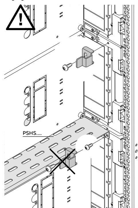
Segregation Form 2a 3a
