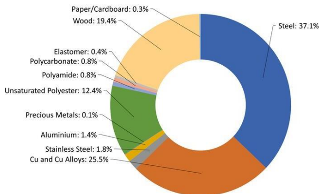
Figure 1: Material composition of DR MPACT F1 65 kA 3P to E2.2 IEC
