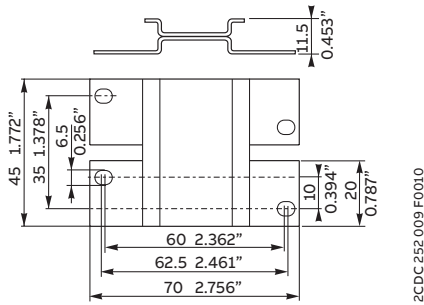
ADP.02 - Adapter for screw mounting
