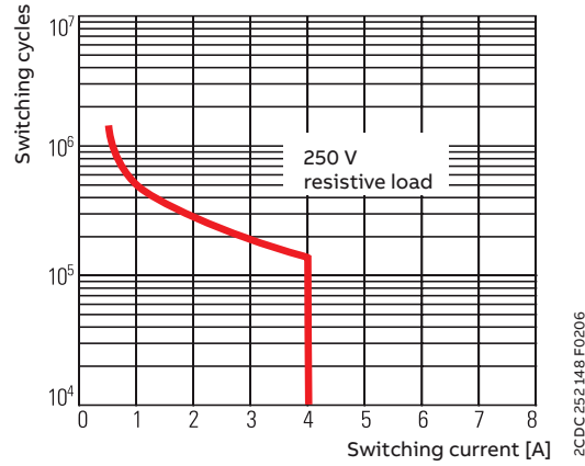
Contact lifetime
