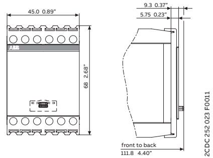
COV.12 - Sealable transparent cover
