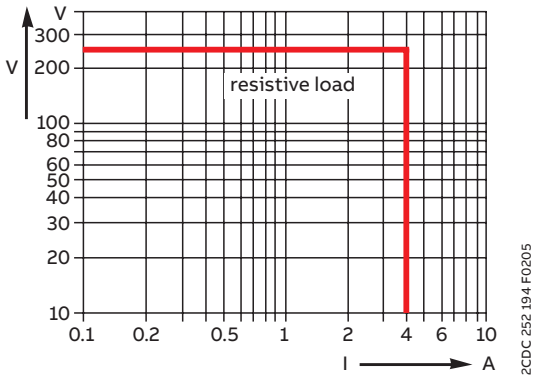
AC load (resistive)
