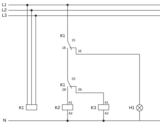
Control circuit diagram (K1 = CM-MPN.x2)
