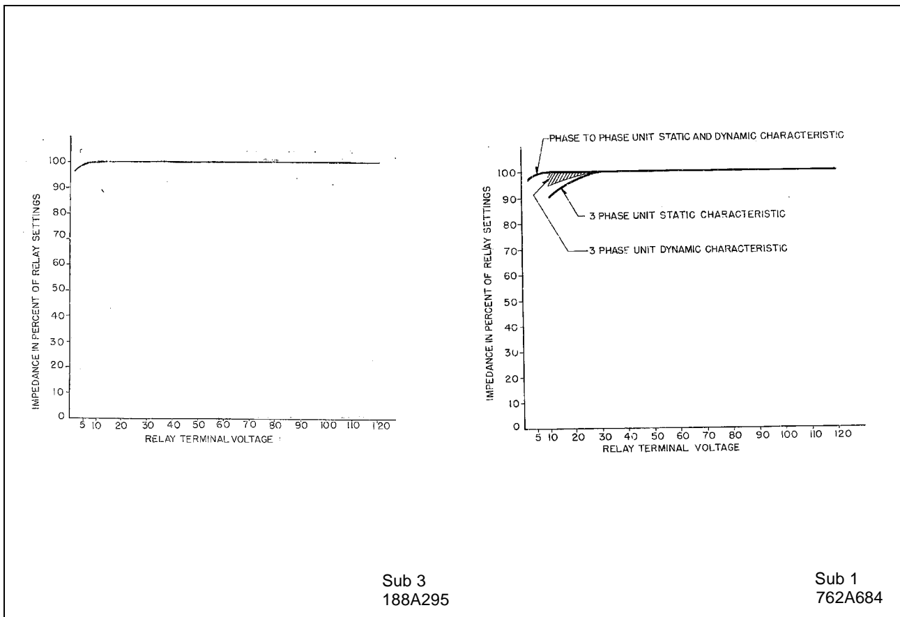
Figure 12: Impedance Curves for KD-10 Relay
