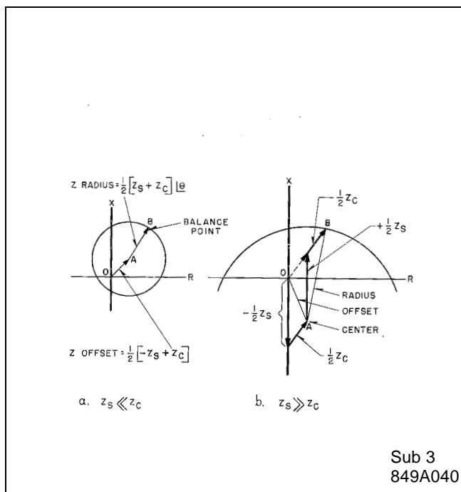
Figure 10: Impedance Circles for Phase-to-Phase Unit in the Type KD-10 and KD-11 Relay
