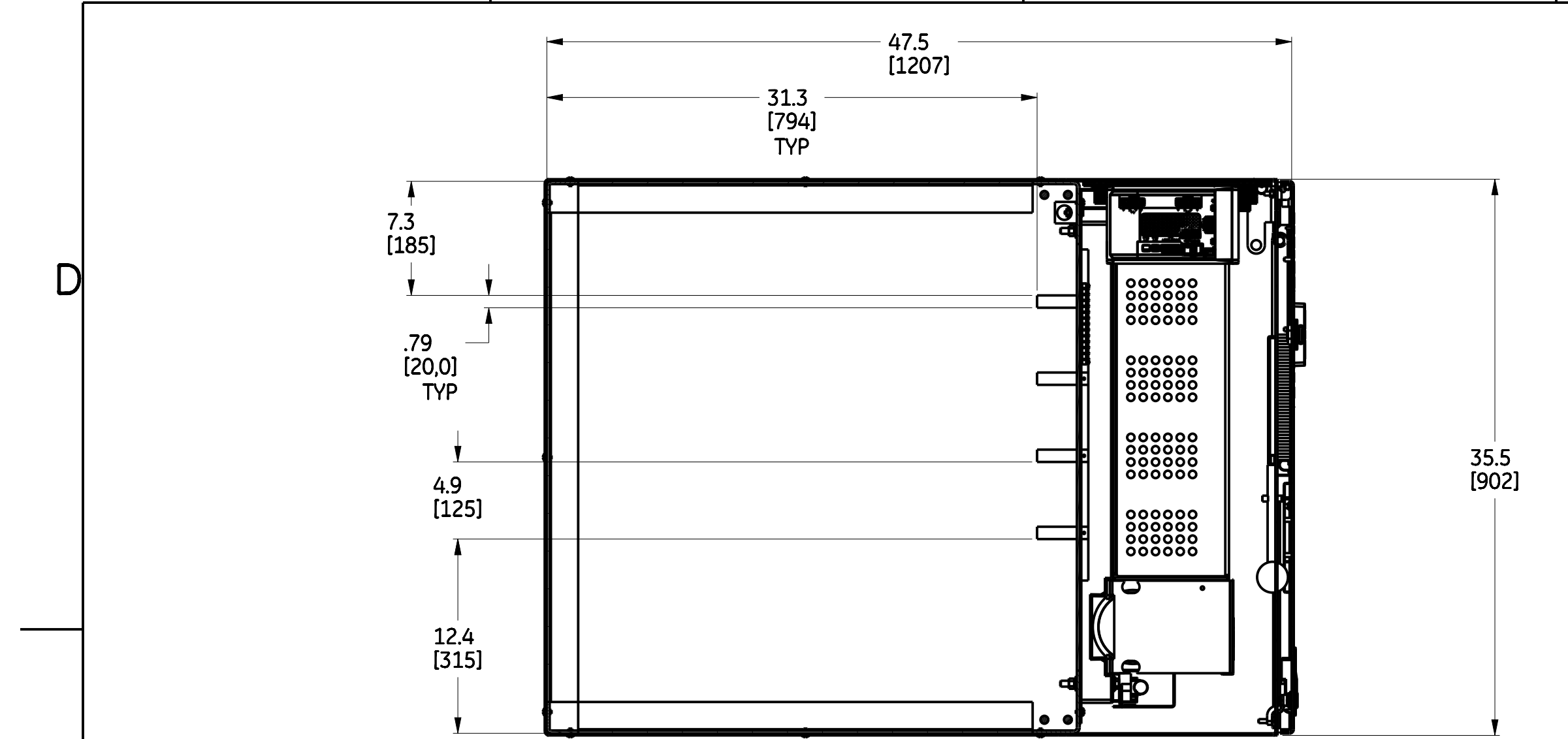
TOP VIEW PANEL REMOVED (4 POLE UNIT)
