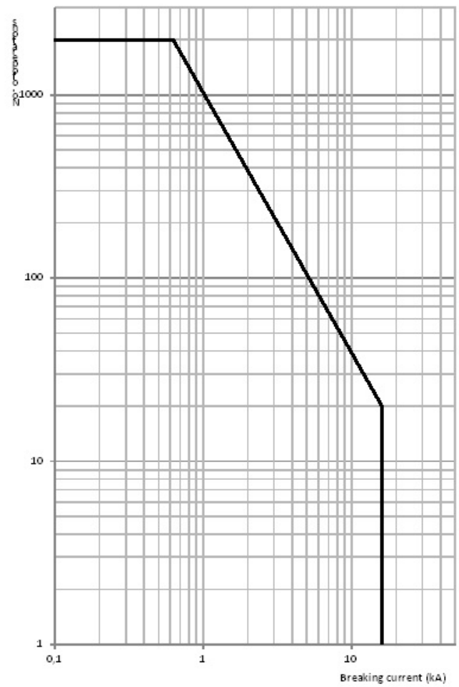
SafeRing V-module 12, 15, 17,5 and 24 kV
