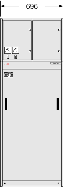
Metering module M, front view
