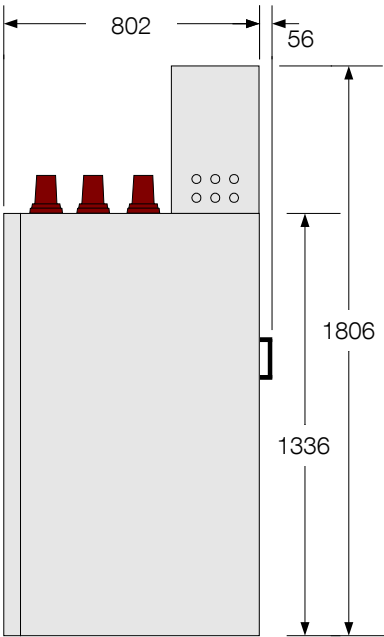
Metering module M, side view right
