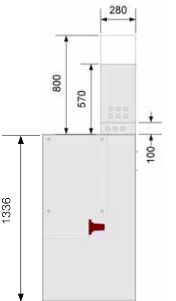
Low voltage compartment for V20/V25
