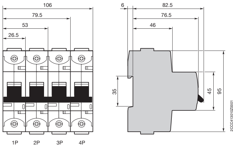
S800U approximate dimensions
