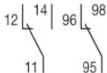
Auxiliary contact S800-AUX/ALT
