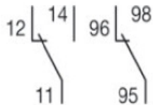
Auxiliary contact S800-AUX/ALT
