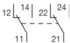
Auxiliary contact S800-AUX
