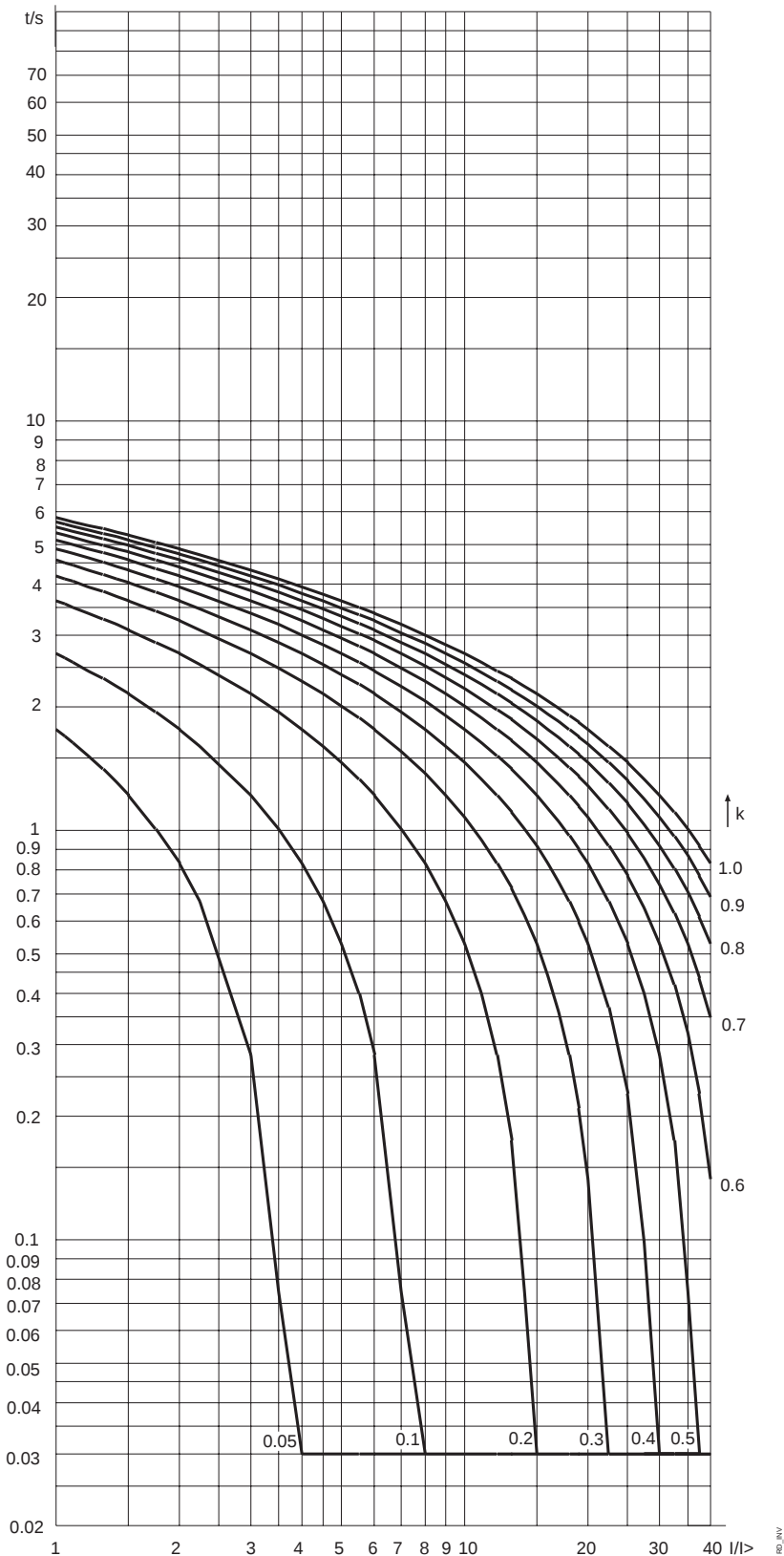
Figure 2.1.3.4-6 RD-type inverse-time characteristics
