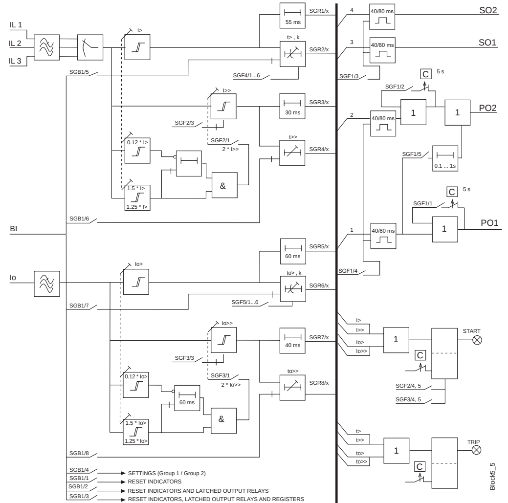
Figure 2.1.3.1-1 Block diagram of the combined overcurrent and earth-fault relay
