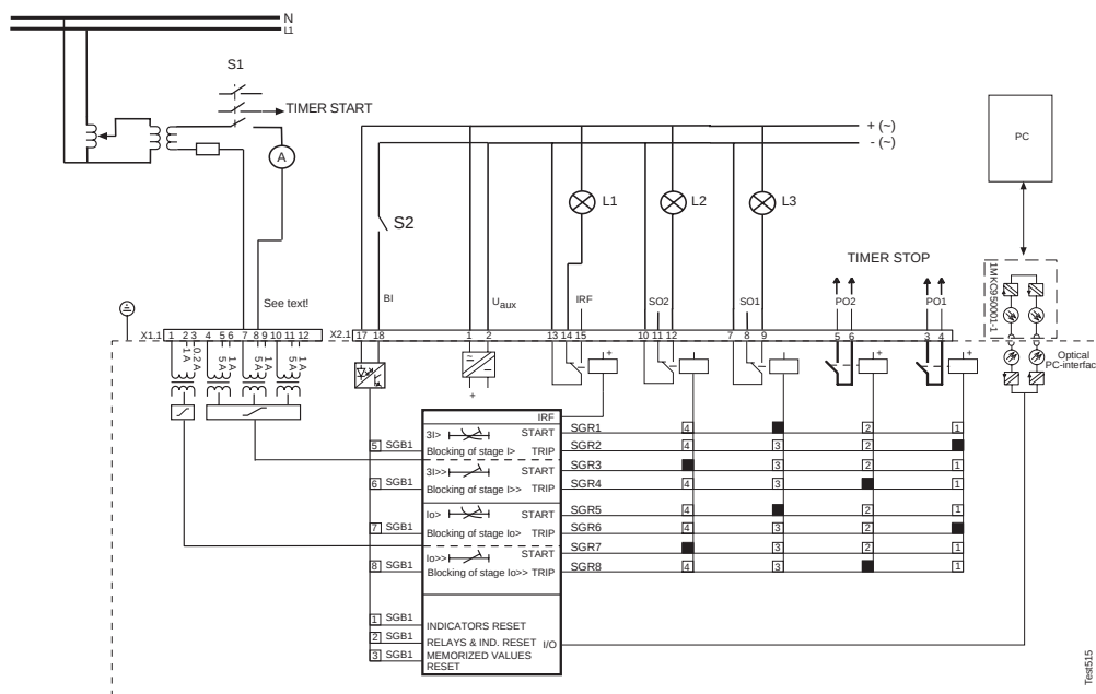
Figure 2-1 Secondary injection test circuitry for the overcurrent and earth-fault relay
