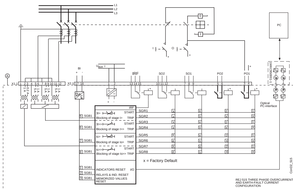
Figure 1.3-2 Connection diagram of the combined overcurrent and earth-fault relay
