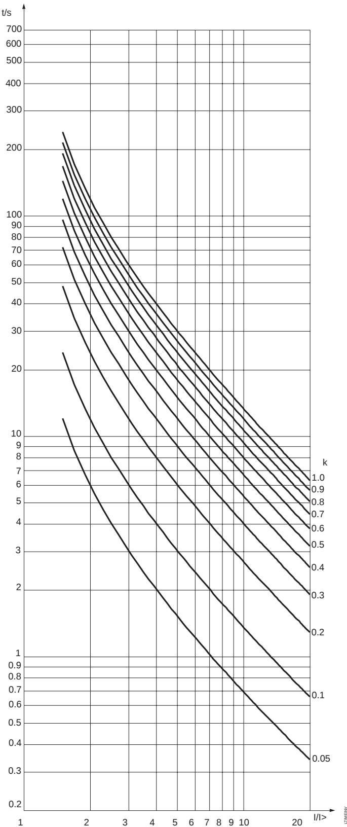
Figure 2.1.3.4-4 Long-time inverse characteristics
