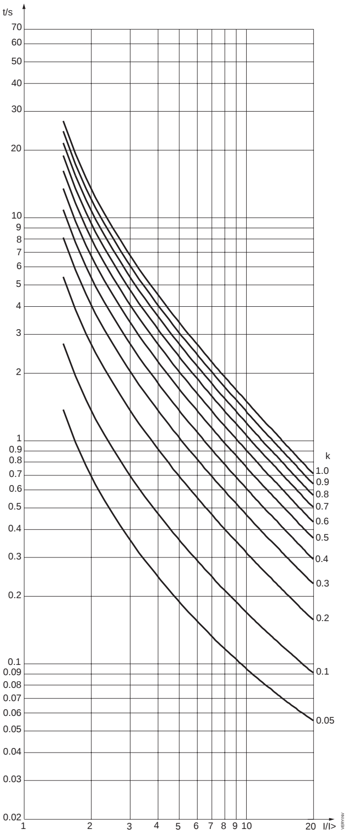
Figure 2.1.3.4-2 Very inverse time characteristics
