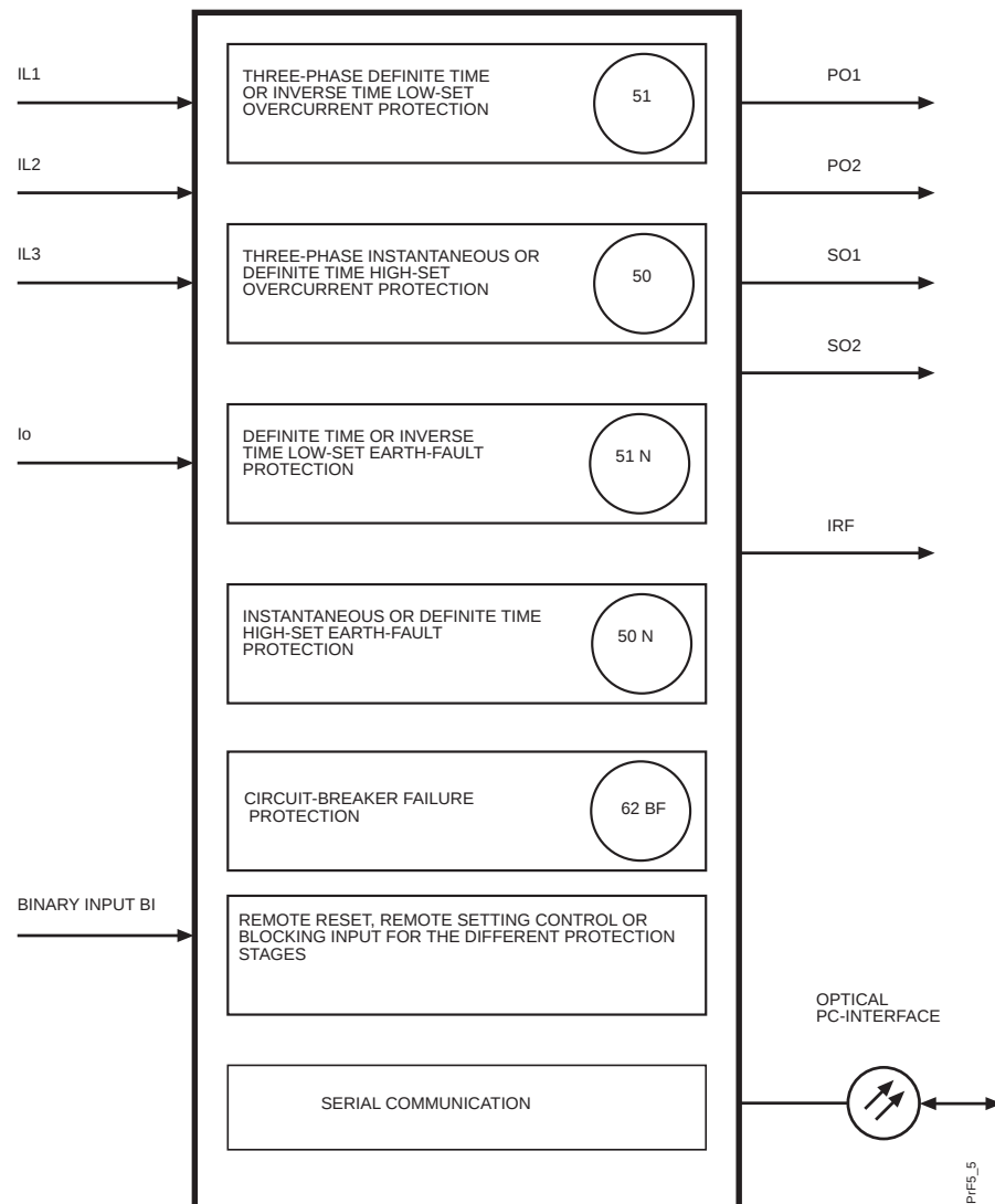
Figure 2.1.1.1-1 Schema of product functions
