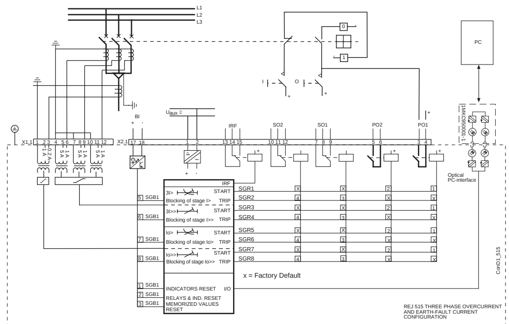
Figure 1.3-1 Connection diagram of the combined overcurrent and earth-fault relay
