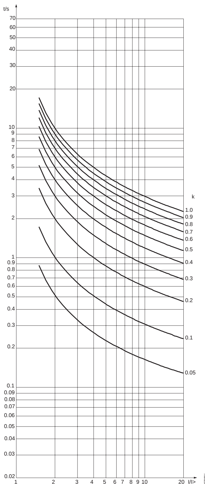
Figure 2.1.3.4-1 Normal inverse time characteristics
