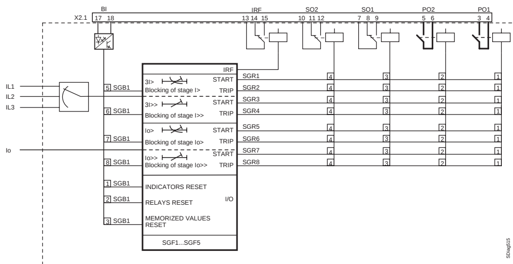
Figure 2.1.2-1 Signal diagram of the combined overcurrent and earth-fault relay
