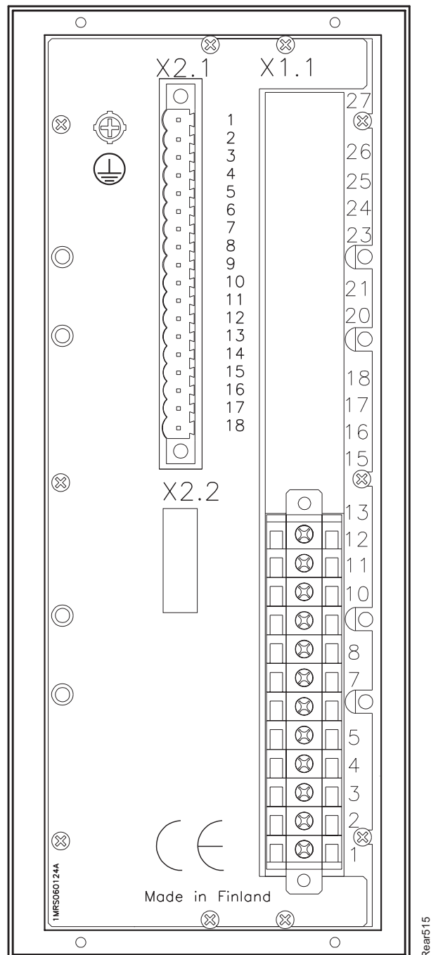
Figure 2.2.1-1 Rear view of the combined overcurrent and earth-fault relay
