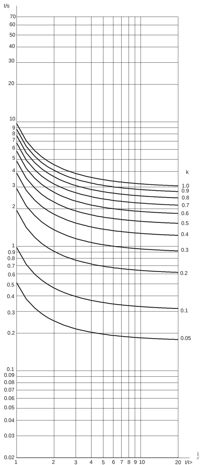
Figure 2.1.3.4-5 RI-type inverse-time characteristics
