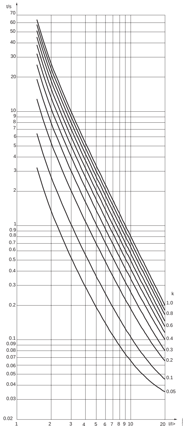
Figure 2.1.3.4-3 Extremely inverse time characteristics
