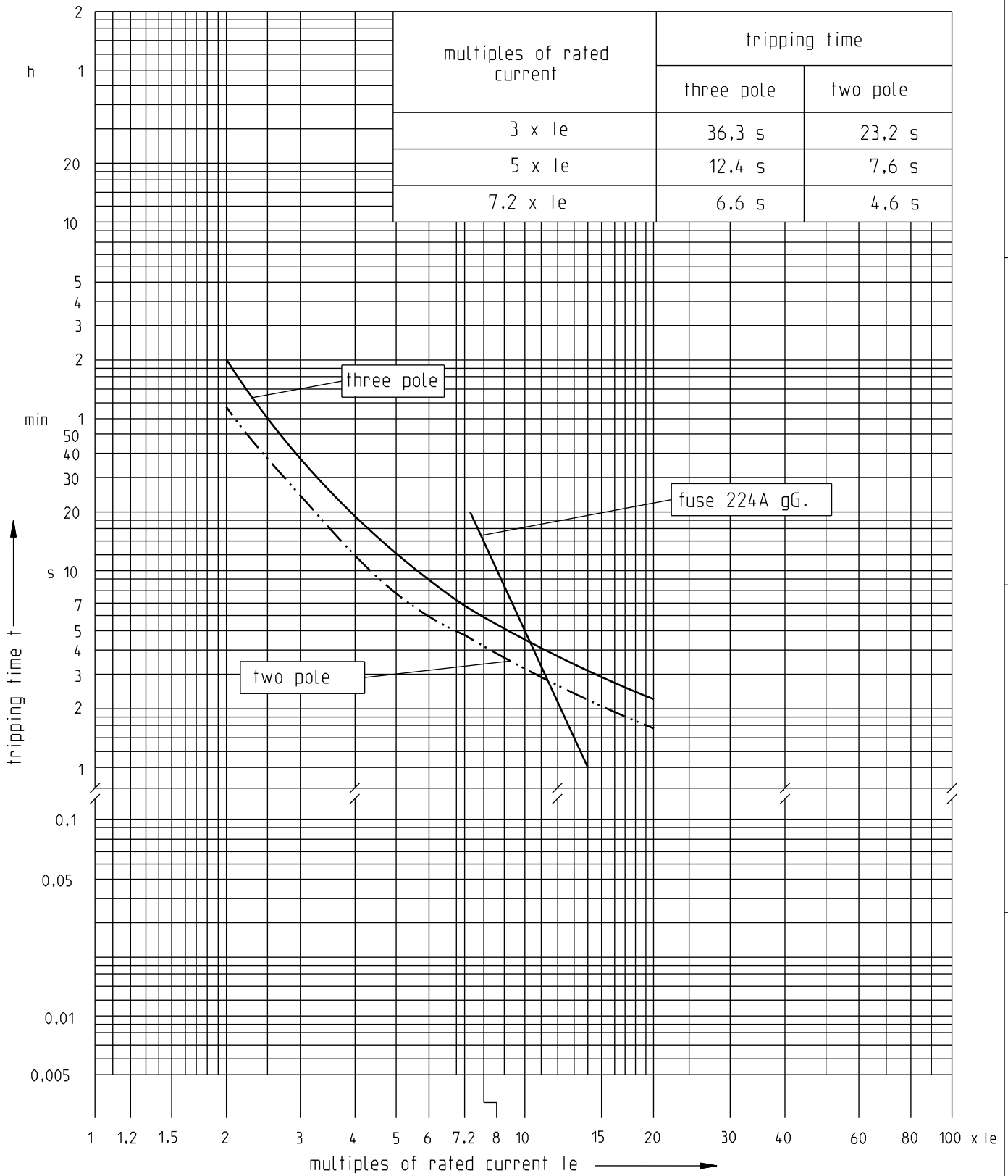
Tripping characteristic (from cold state) For currents (3-pole) between 3 and 8 times the current setting the tolerance of the tripping time is \pm 20\%
