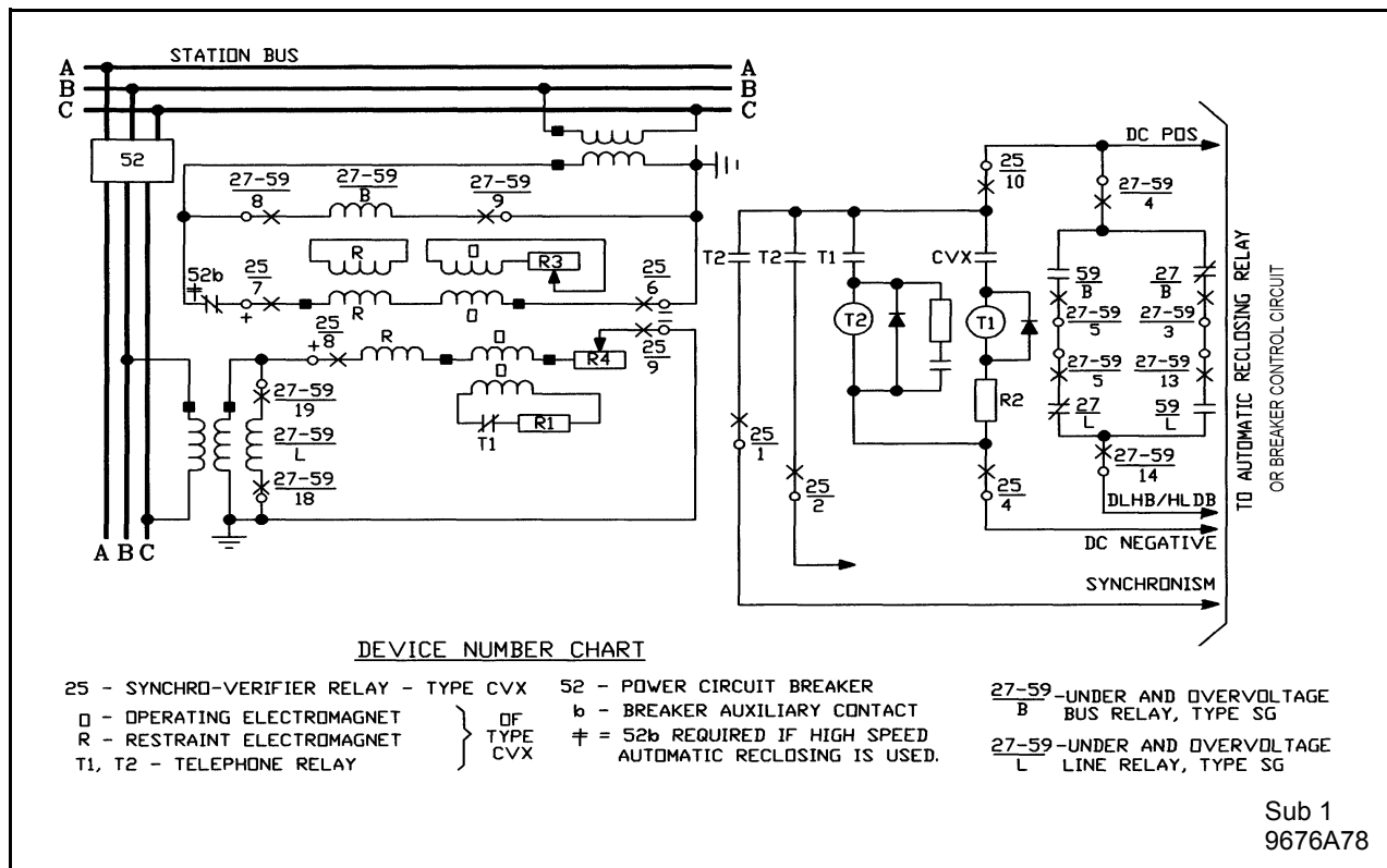
Figure 6. External Schematic of Type CVX Synchro-Verifier Relay with Isolated Potential Circuits and External Voltage Relays.
