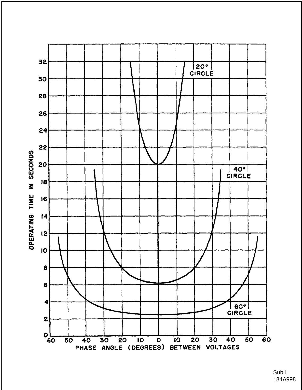
Figure 9. Typical Time Phase Angle Curves of CVX and CVX-1 Relays. Rated Voltage on Both Circuits. Number 11 Time Dial Setting.
