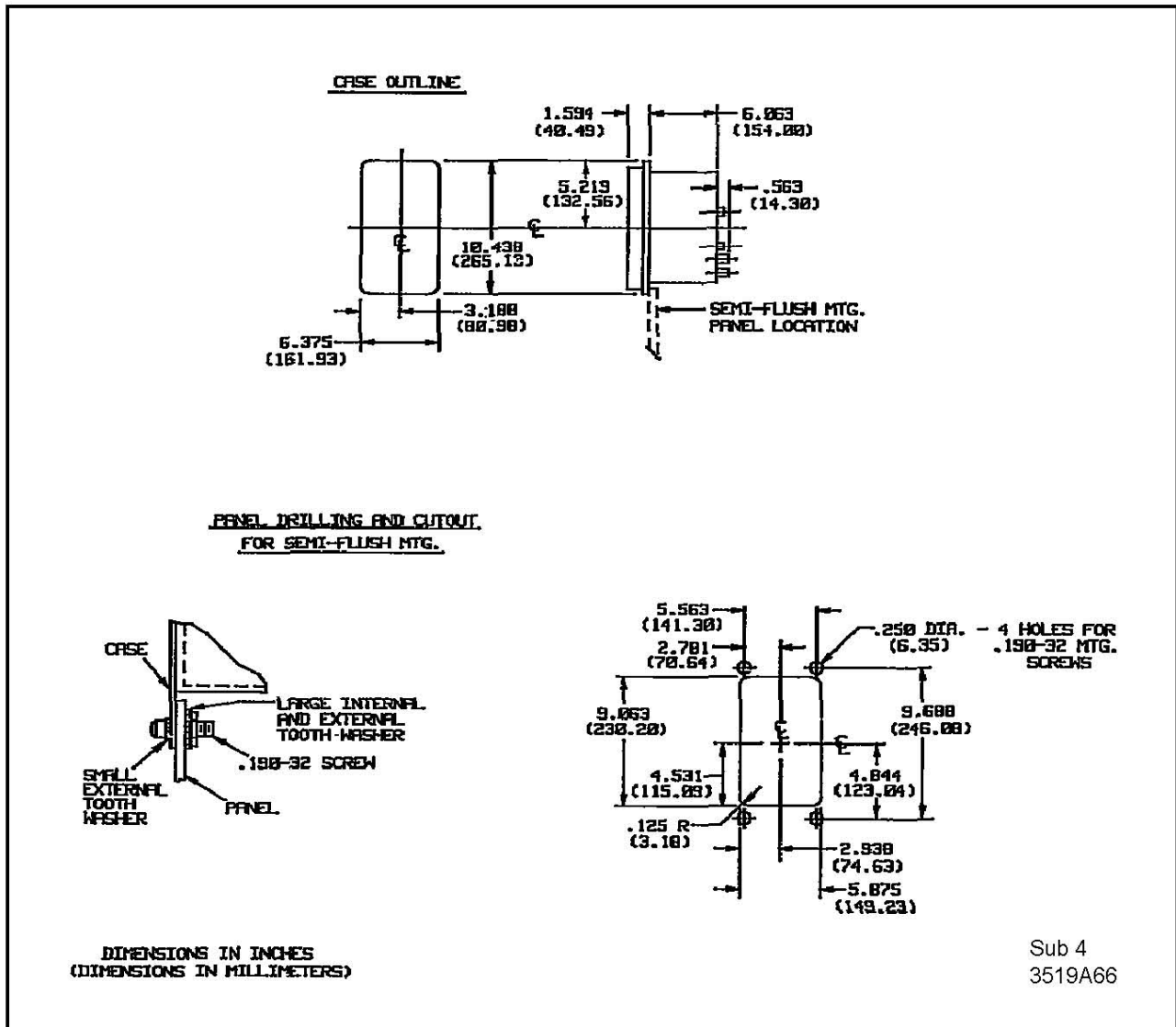
Figure 17. Outline and Drilling Plan for Type CVX and CVX-1 Relays in FT-21 Case
