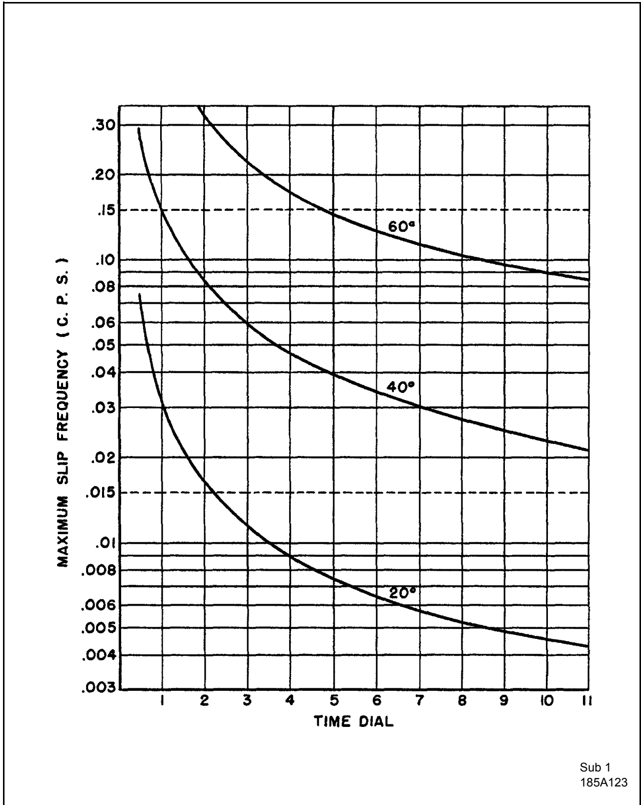
Figure 11. Approximate Maximum Slip Frequency for which Operation Occurs. Rated Voltage Both Sides.
