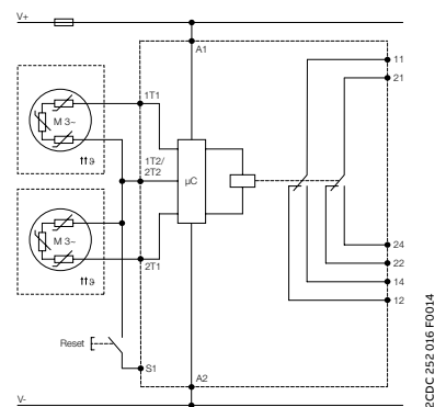
CM-MSS.51x
