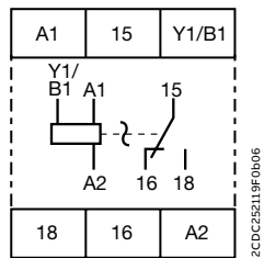
CT-TGD.12
