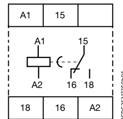
CT-ERD.12
