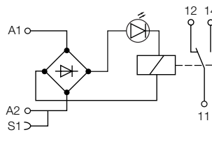
RB(R)122G-115VUC/230VUC
