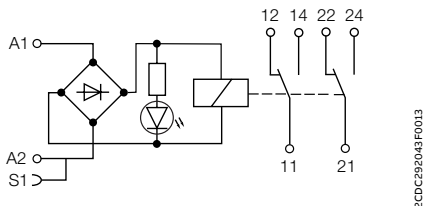
RB(R)122G-24VUC/48-60VUC
