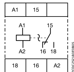
CT-EBD.12
