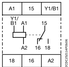
CT-MFD.12
