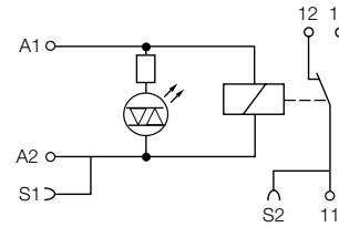
RB(R)121-12VDC/24VDC
