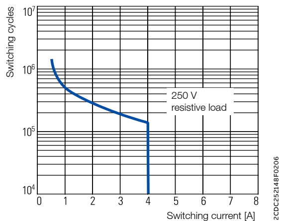
Contact lifetime
