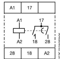
CT-SAD.22
