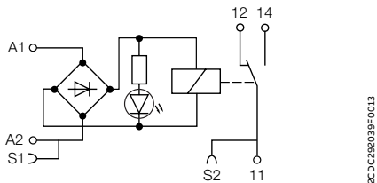
RB(R)121(G)-24VUC
