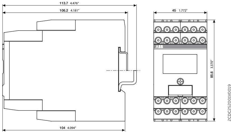
CM-TCN.011
