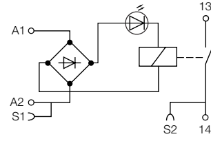
RB111-115VUC/230VUC
