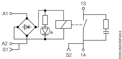
RB(R)111R-24VUC
