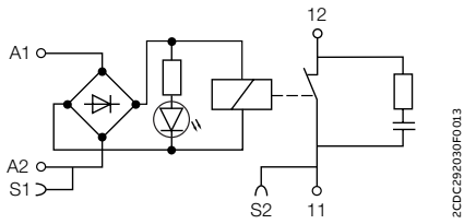
RB(R)101R-24VUC
