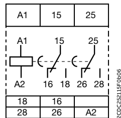
CT-ERD.22
