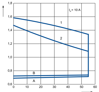
Operating range of AC coil – 3 c/o
