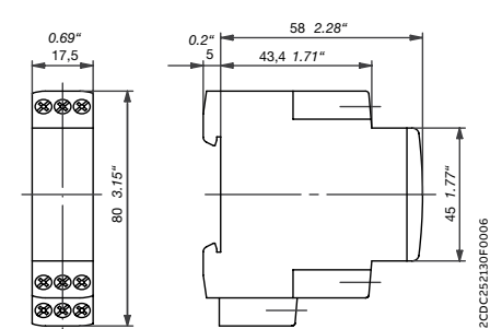
CT-D devices with 2 c/o contacts
