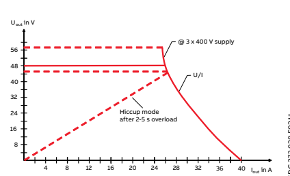
CP-T 48/20.0
