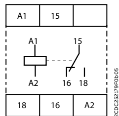
CT-VWD.12
