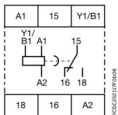
CT-AHD.12
