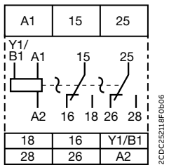
CT-TGD.22
