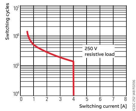
Contact lifetime
