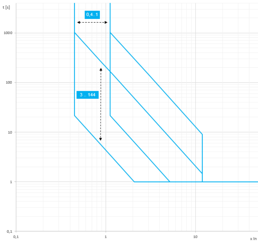
L 曲线 ( t = k/I^2 )
