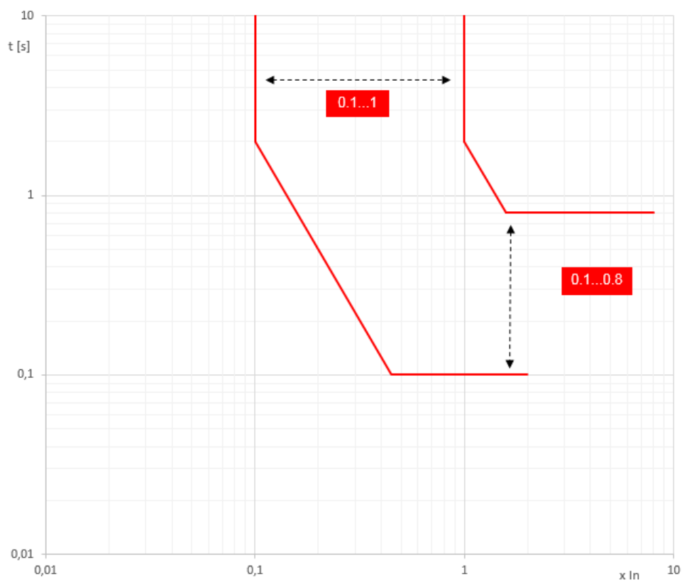
G 曲线 ( t = k/l^2 )
