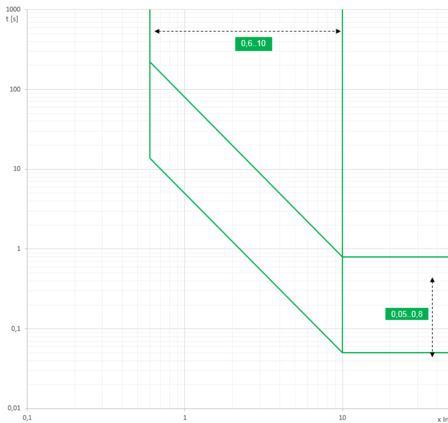
S 曲线 ( t = k/l^2 )
