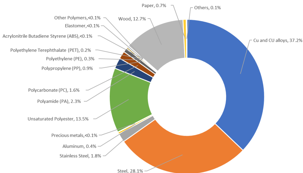
Figure 1: Composition of E6.2 5000A H-A/V-A - 3P Withdrawable Circuit Breaker
