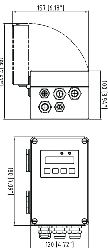
PFEA 111 Version IP65
