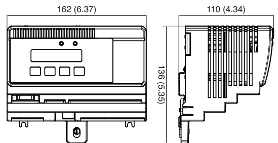
PFEA 113 Version IP20
