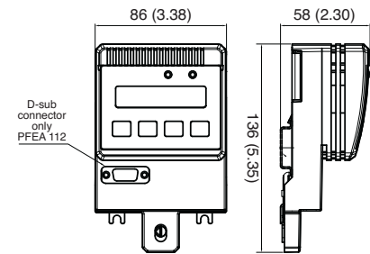
PFEA 113 Version IP20
