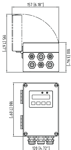
PFEA 112 Version IP65
