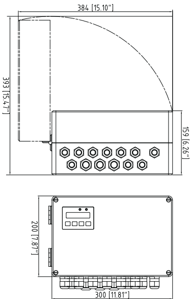
PFEA 113 Version IP65
