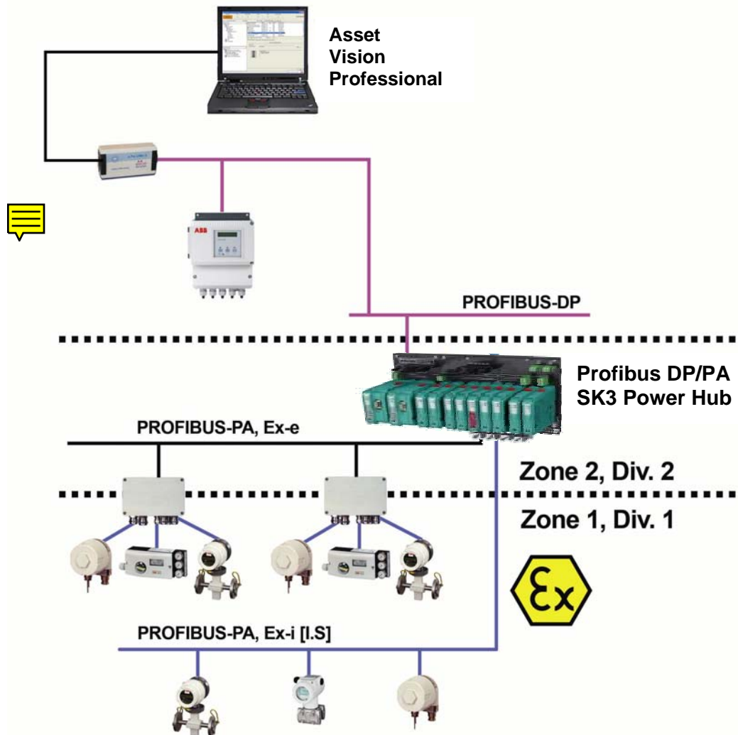
Figure 17. Example of fieldbus structure with SK3 Power Hub
