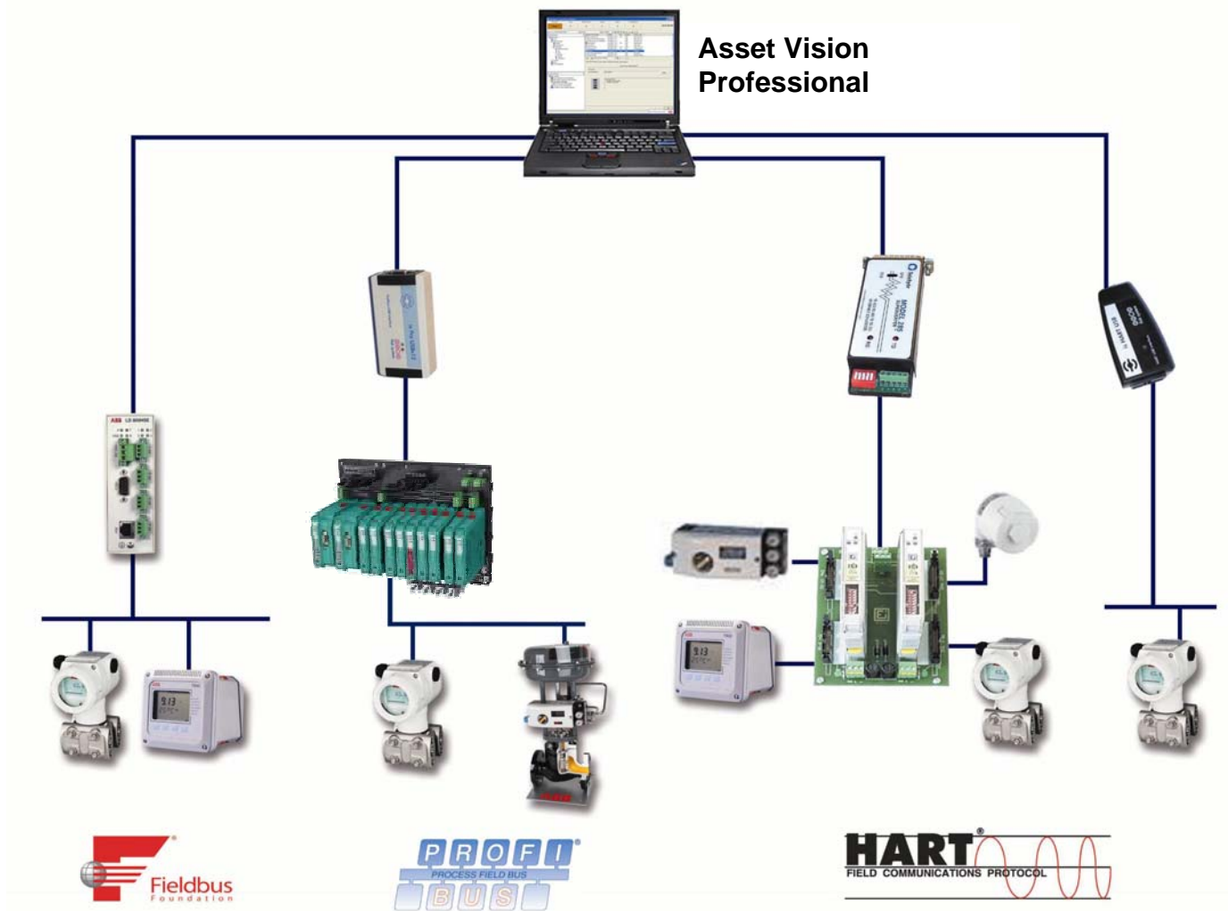
Figure 1. Asset Vision Professional Fieldbus Connections
