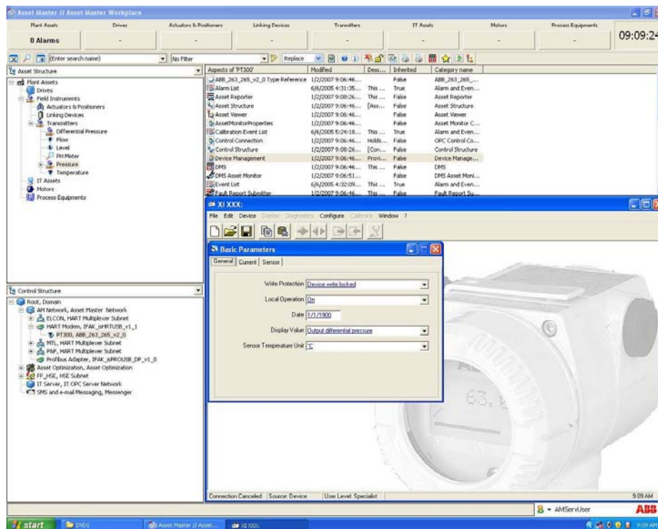
Figure 2. Field Device Planning in Asset Vision Professional
