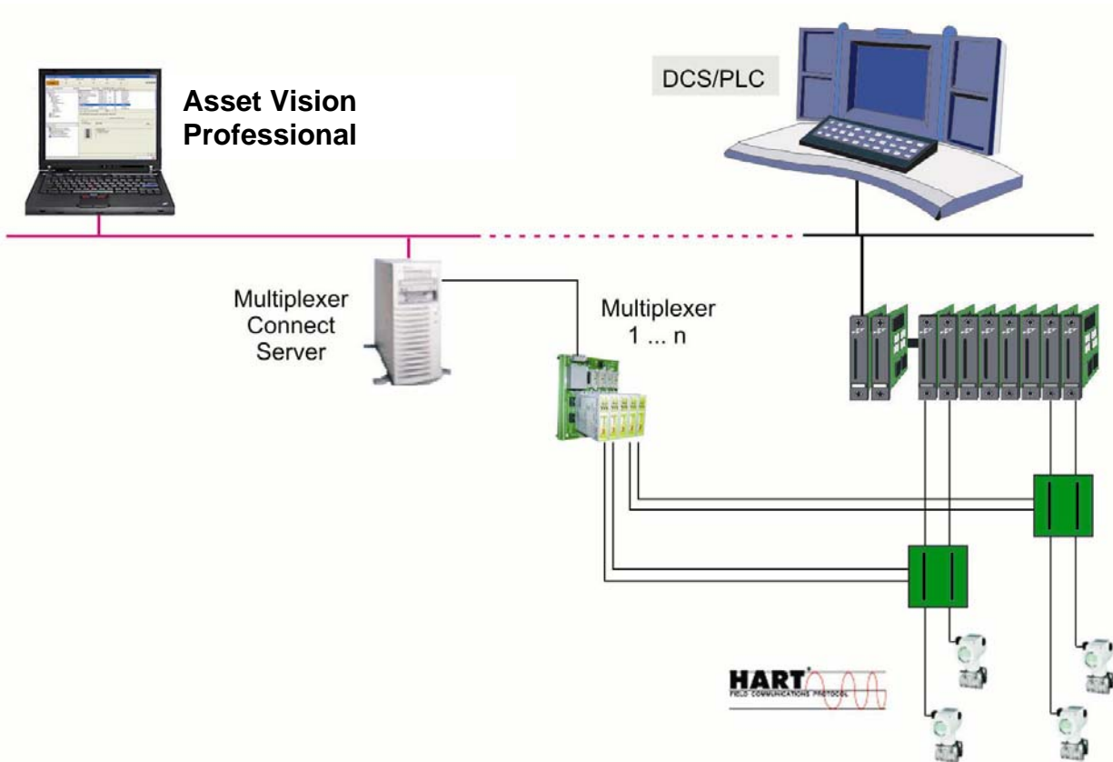
Figure 12. Example of a HART Multiplexer system topology
