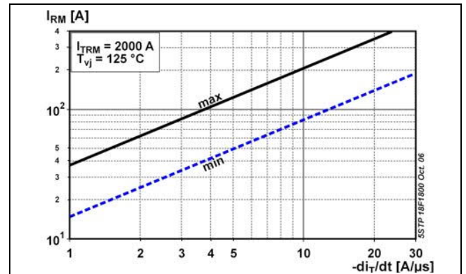
Fig. 9 Peak reverse recovery current vs. decay rate of on-state current
