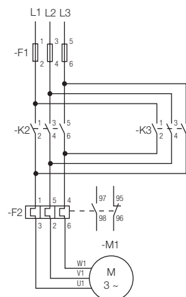
Power circuit diagram
