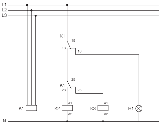
Control circuit diagram (K1 = CM-MPS.43)
