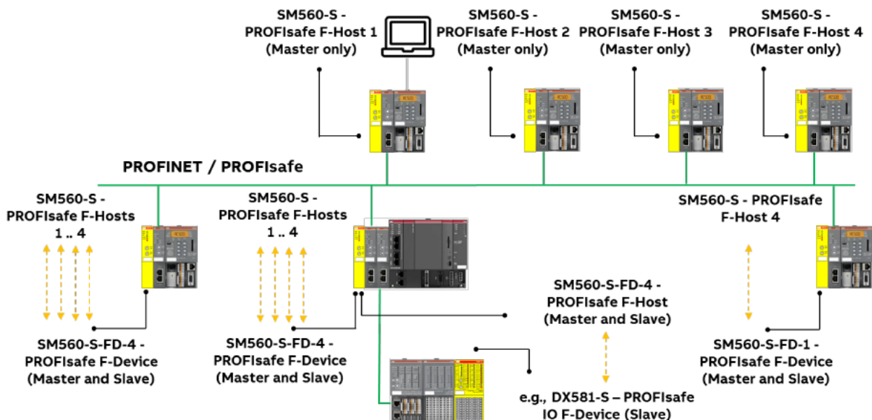
Figure 2: Safe CPU communication between Safety CPUs (SM560-S / -FD1 / -FD4) (Example)
