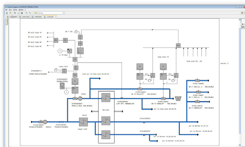
PI diagram
