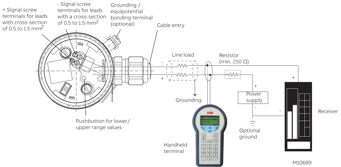
Electrical connections - HART version
