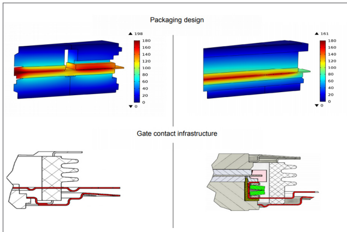
Comparison of previous (left) with improved generation 3 design platform (right).
