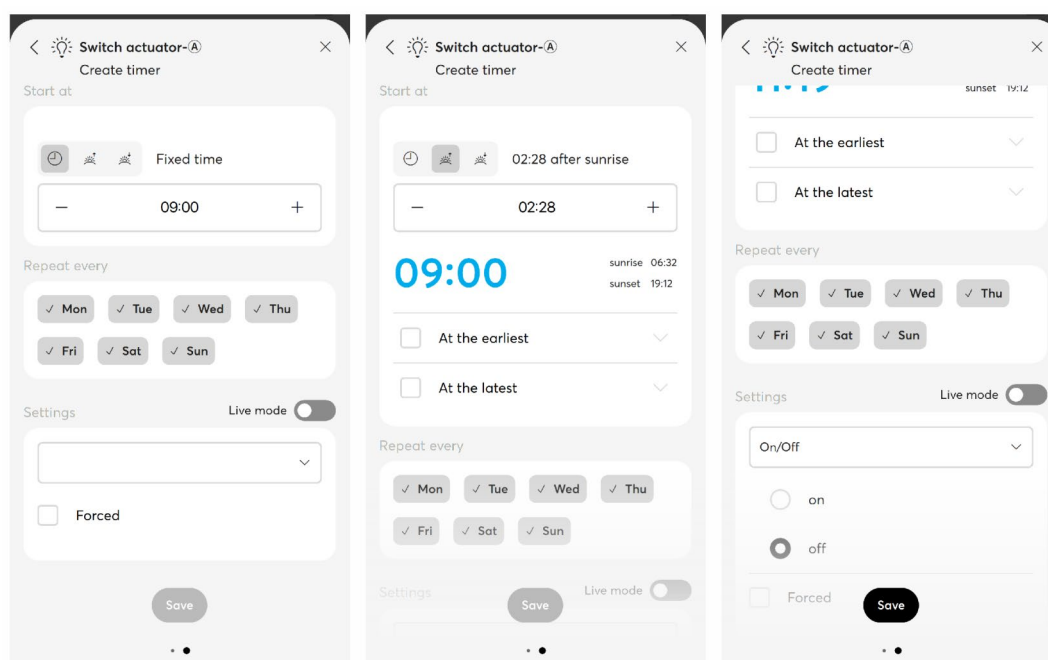
Fig. 31: Automation Settings
