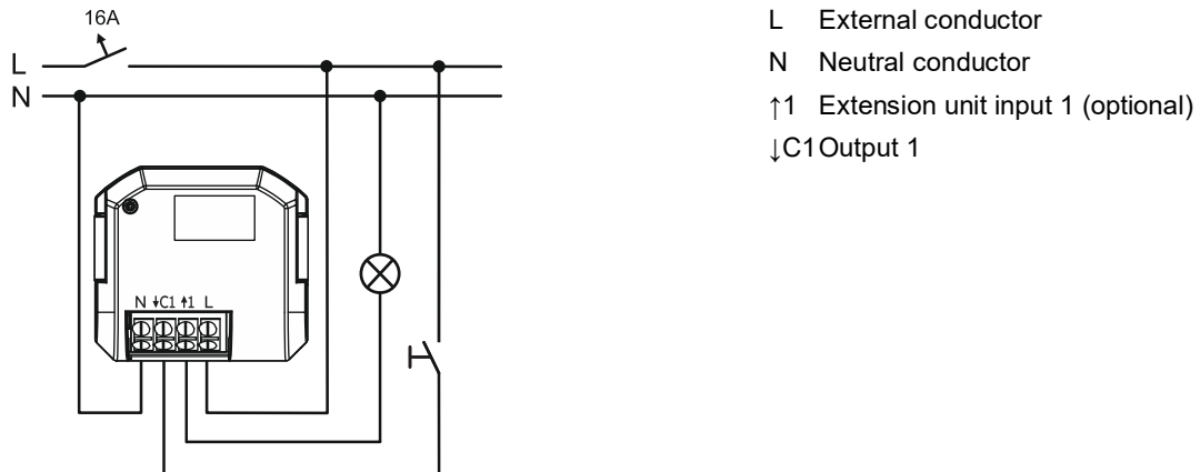
Fig. 5: Electrical connection 62811 U-WL
