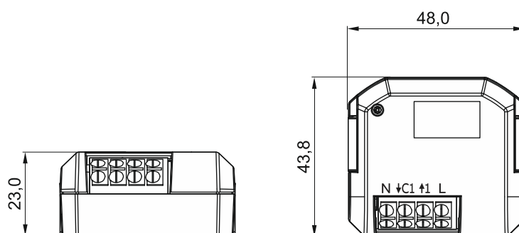
Fig. 4: Dimensions (all dimensions are in mm)
