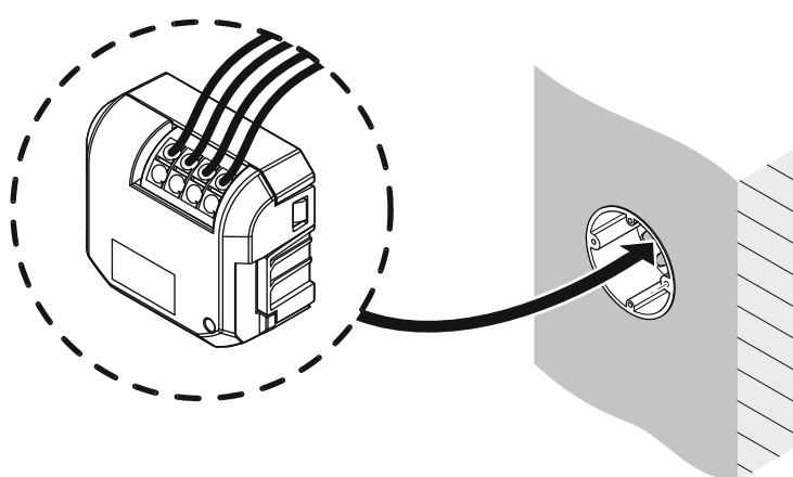
Fig. 6: Mounting in the flush-mounted box
