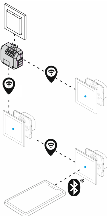
Fig. 8: Room control expansion stage
