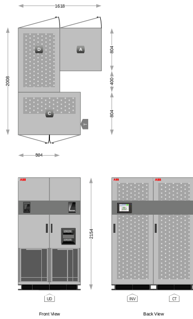
Frame Size: 1xA 1xC 1xD
