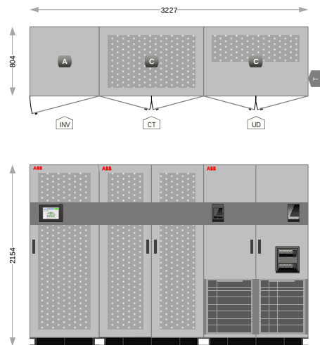
Frame Size: 1xA 2xC
