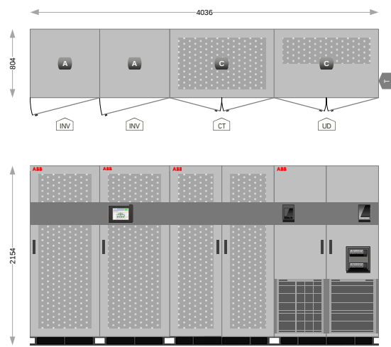
Frame Size: 2xA 2xC
