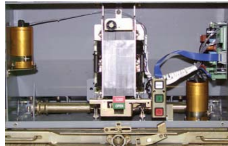
AMVAC magnetic actuator operating mechanism
