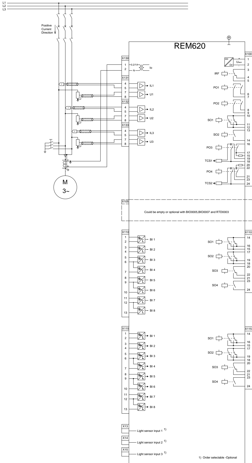
Figure: REM620 ME202 Connection diagram for standard modules
