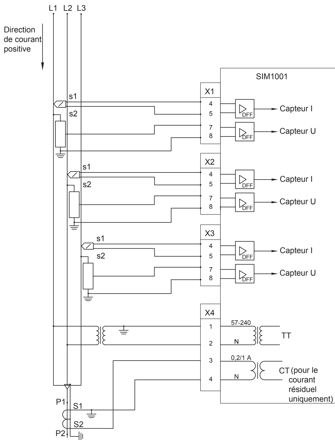
Figure 24. Module SIM1001
