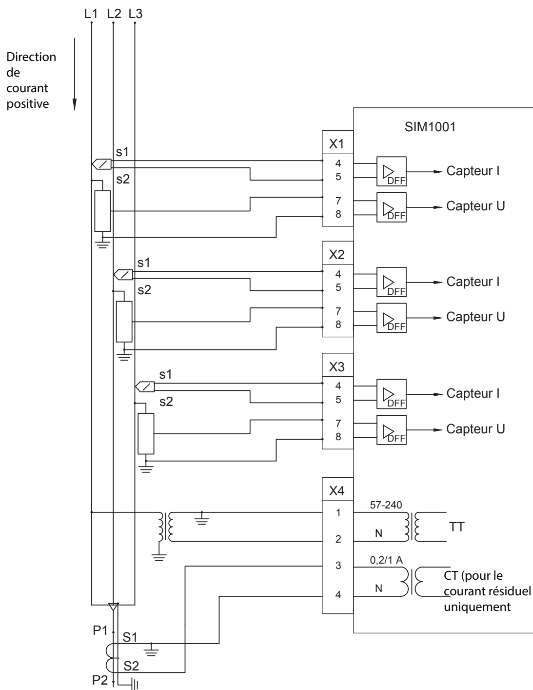
Figure 25. Module SIM1001
