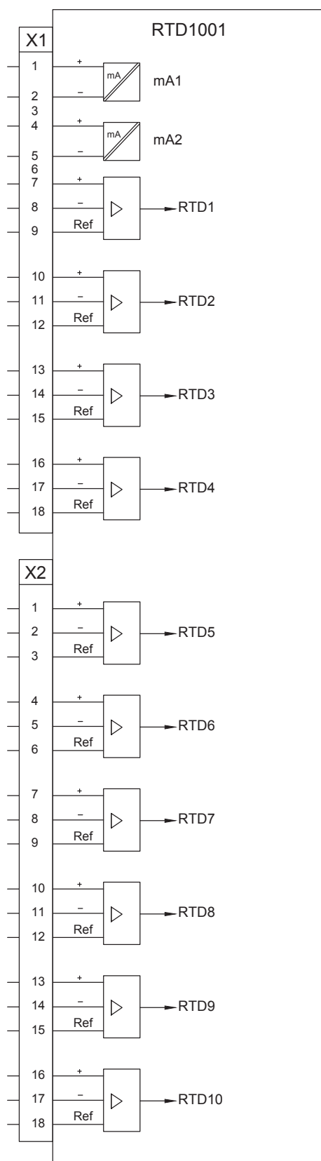
Figure 29. Module RTD1001
