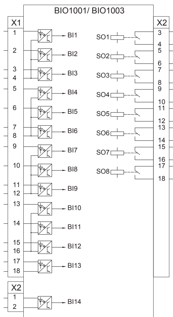
Figure 26. Modules BIO1001/BIO1003
