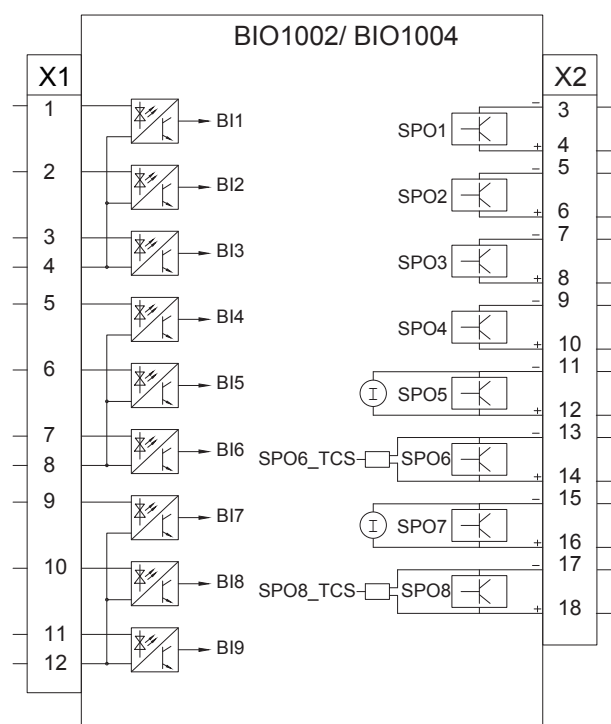
Figure 27. Modules BIO1002/BIO1004
