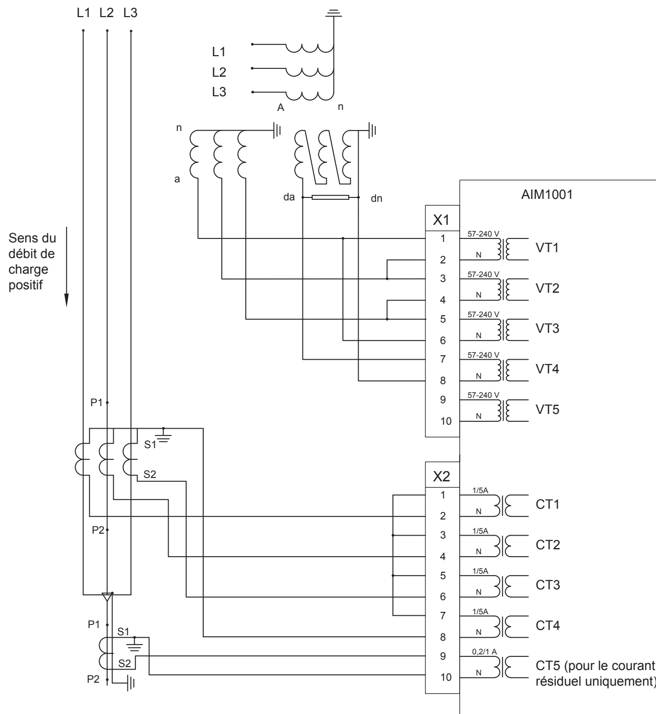
Figure 22. Module AIM1001
