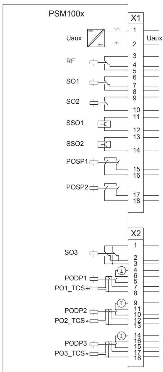
Figure 28. Module PSM100x
