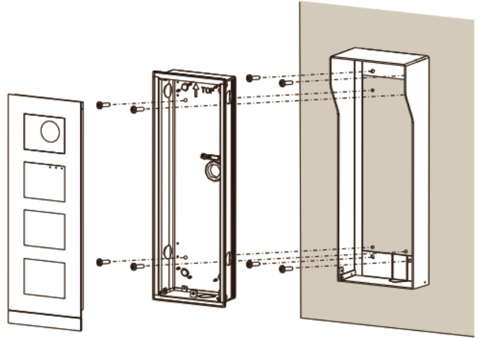
Surface mount
