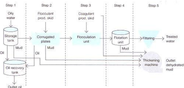
Figure 2: Oily Water Treatment Schematic
