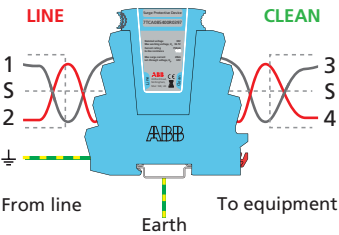
Figure 1: Series connection of OVR SL**X.
