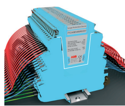
Figure 2: Installation on a 35 mm DIN rail.
