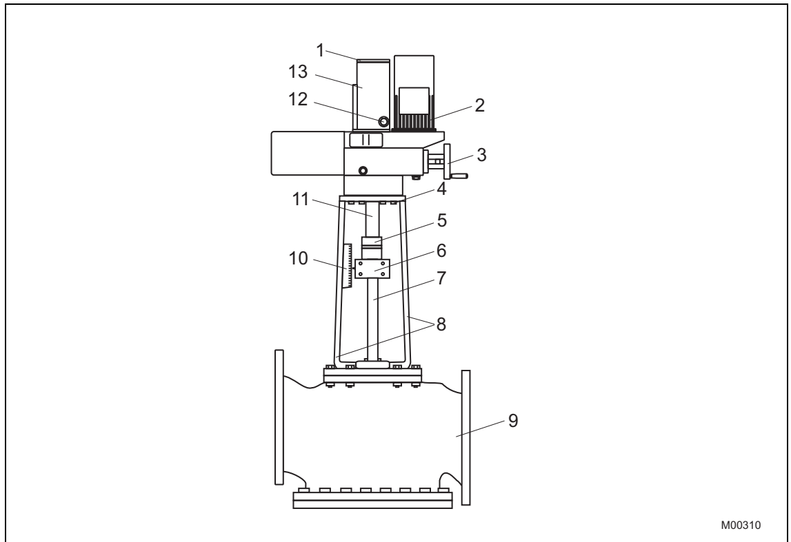
Fig. 5: Installation example RSDE10 ... 50 (Contrac)
