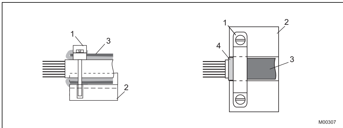
Fig. 6: Fitting the shield
