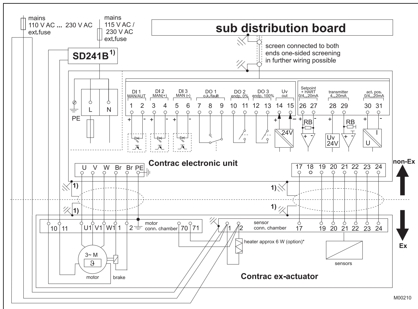
Fig. 11: Electrical connection: Ex actuator analog / digital
