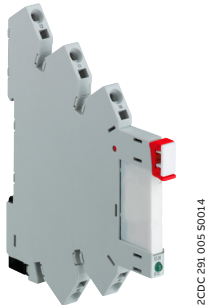
CR-S Interface relay
