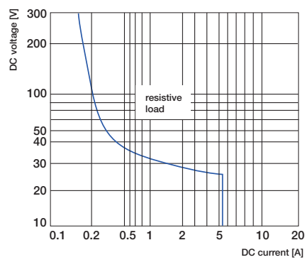
Versions with 1 n/o, 1 n/c or 1 c/o contact
