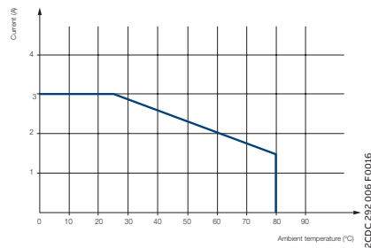
Derating curve MOS-FET output CR-S
