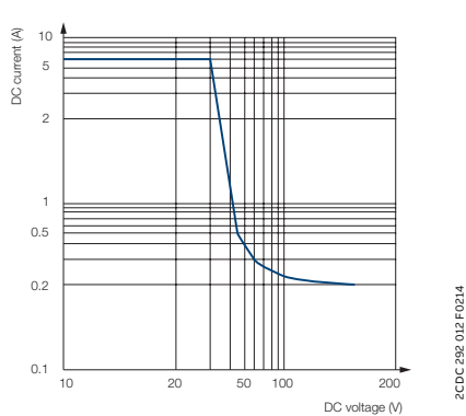
Max. DC load breaking capacity
