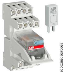
CR-M complete version relay
