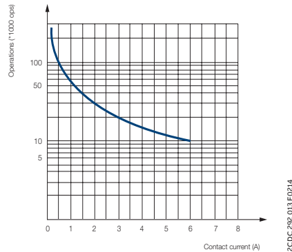
Endurance curve
