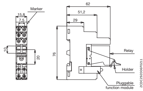
CR-PLS - screw connection
