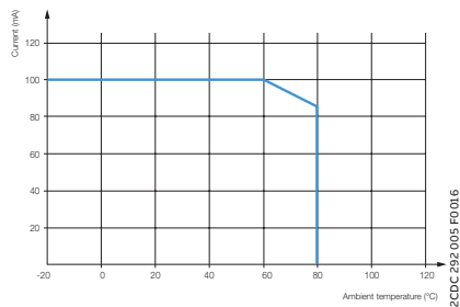
Derating curve Transistor output CR-S
