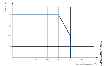
Derating curve Triac output CR-S
