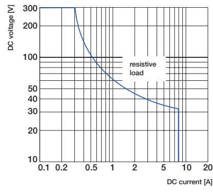
Versions with 2 c/o contacts
