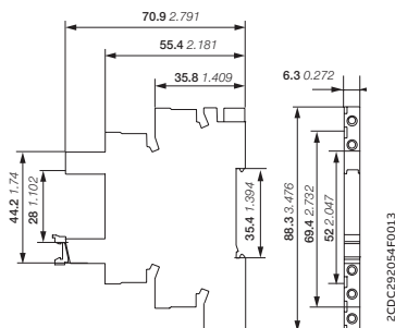
Screw socket for CR-S range interface relays
