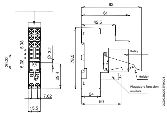
CR-PLSx - screw connection
