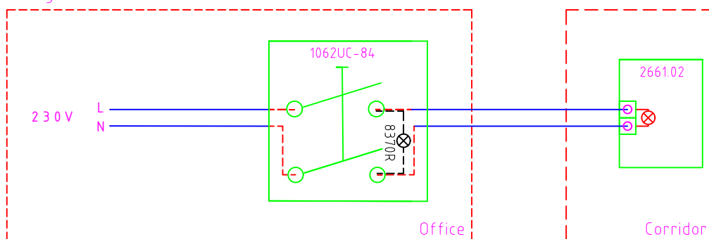
Wiring with 2 switch
